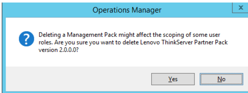
Figure 26: Confirmation Message
