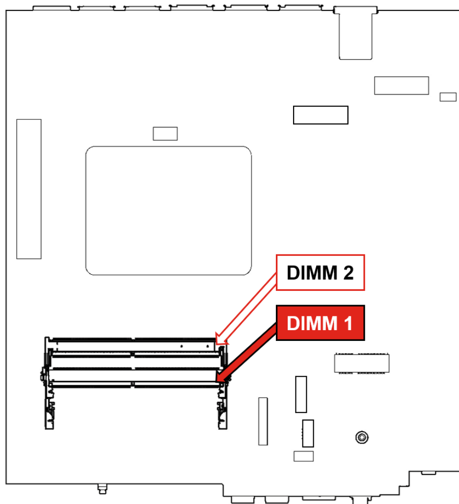
Figure 5 - P3 Ultra SFF Gen 2 Motherboard Layout (RAM Side)
