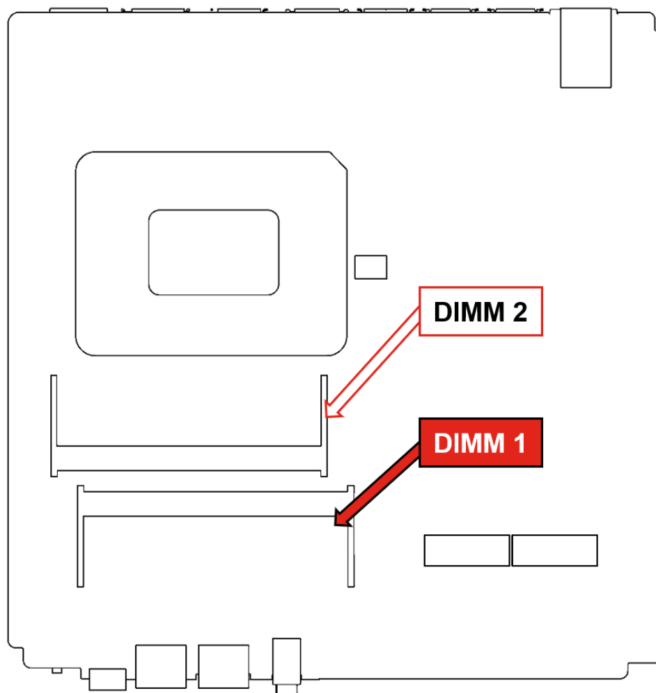
Figure 3 - P3 Tiny Gen 2 Motherboard Layout
