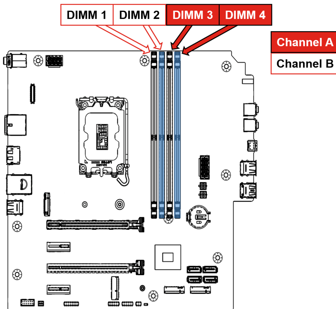
Figure 1 - P3 Tower Gen 2 Motherboard Layout
