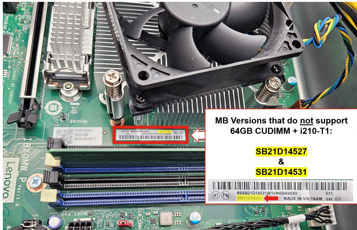
Figure 7 – P3 Tower G2 MB Version Not Supporting 64GB CUDIMM + i210-T1
