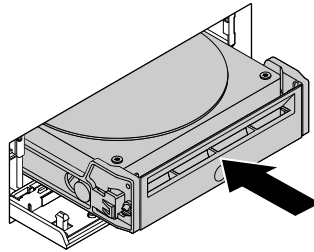
Figure 49. Installing the 3.5-inch storage drive into the front-access storage enclosure
