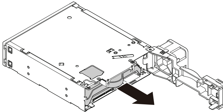
Figure 60. Removing the 3.5-inch storage drive from the rear
