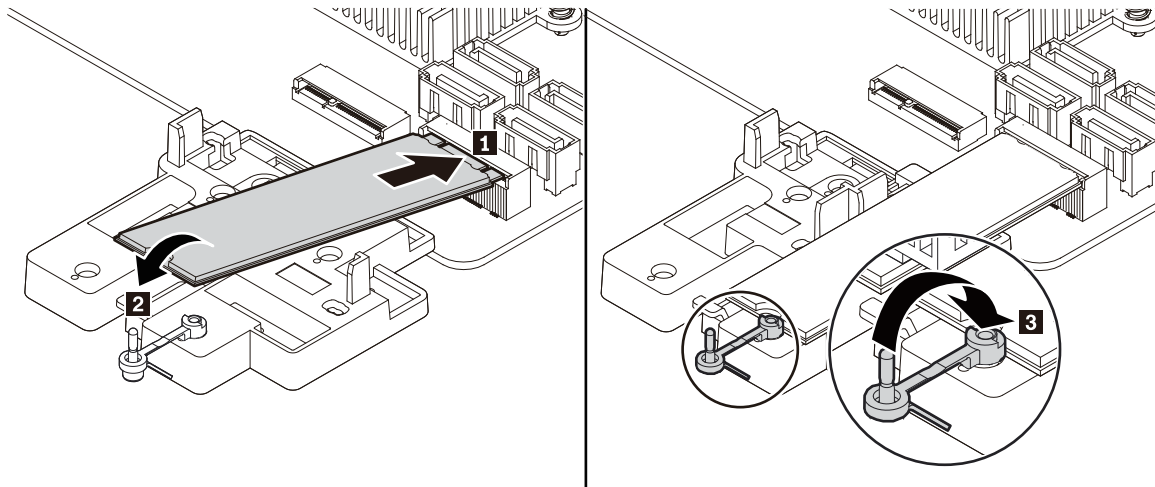
Figure 29. Installing the M.2 solid-state drive
