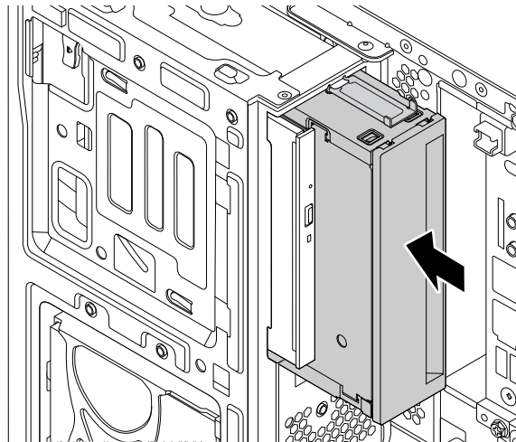
Figure 44. Installing the new flex storage enclosure
