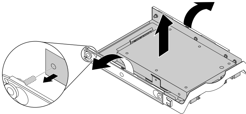
Figure 66. Removing the storage-drive converter from the 3.5-inch storage-drive bracket
