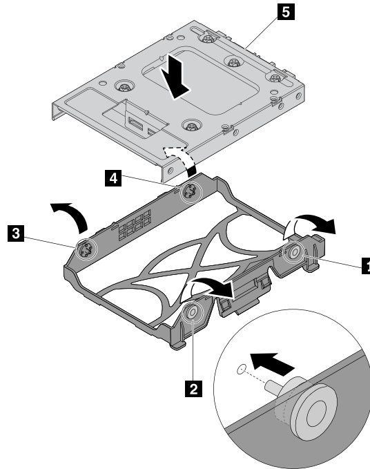
Figure 84. Installing the 2.5-inch storage drive with the storage-drive converter into the bracket
