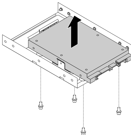
Figure 67. Removing the 2.5-inch storage drive from the storage-drive converter
