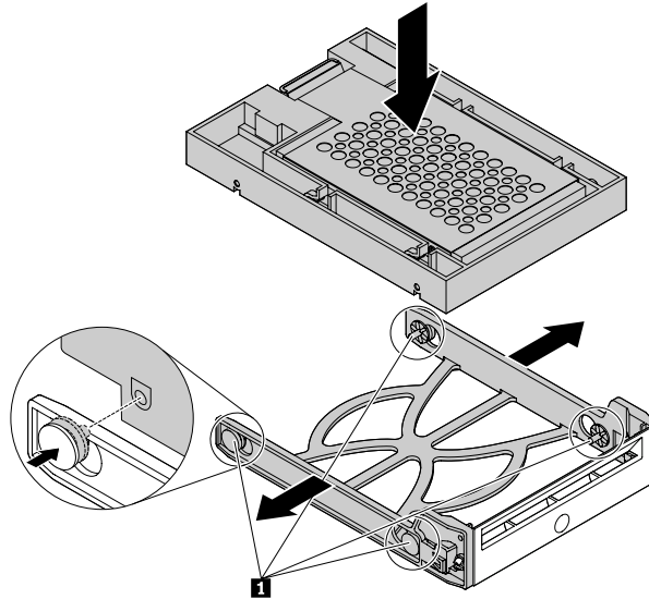
Figure 57. Installing the converter with the 2.5-inch storage drive into the plastic bracket
