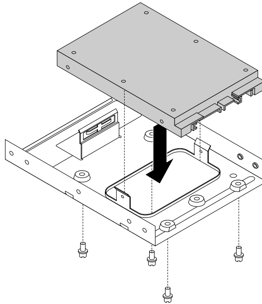
Figure 68. Installing the new solid-state drive into the storage converter
