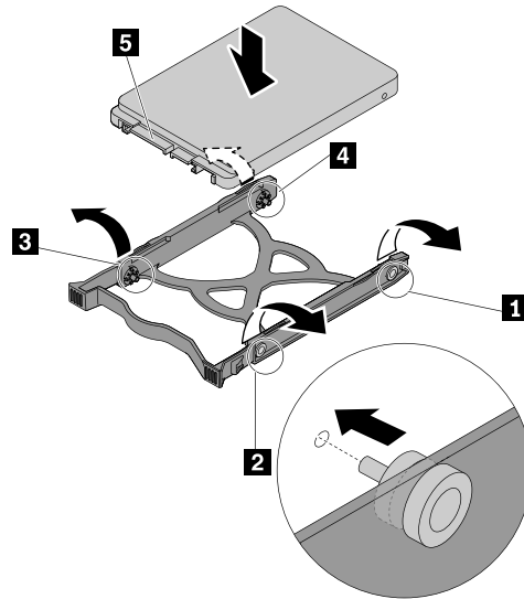
Figure 101. Installing the 2.5-inch storage drive into the bracket
