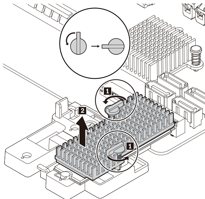
Figure 25. Removing the heat sink from the plastic holder
