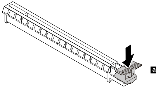
Figure 20. Disengaging the card retaining latch
