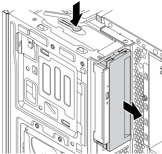
Figure 41. Removing the flex storage enclosure
