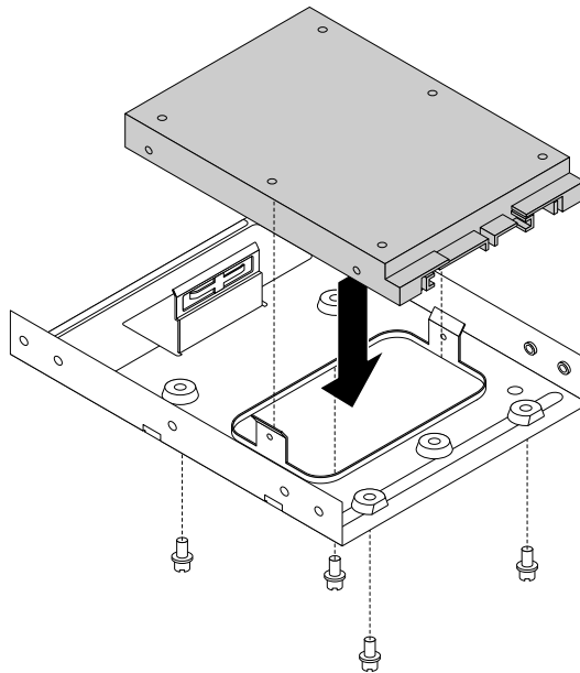
Figure 83. Installing the new 2.5-inch storage drive into the storage-drive converter
