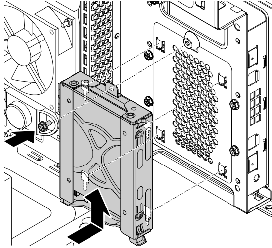
Figure 103. Installing the type-2 storage-drive cage
