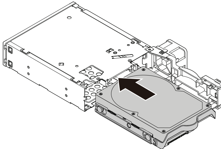
Figure 62. Installing the 3.5-inch storage drive into the enclosure
