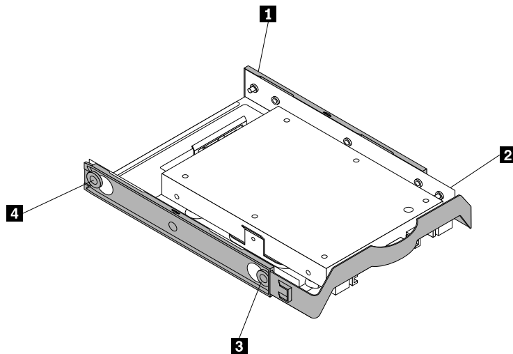
Figure 69. Installing the storage converter together with the solid-state drive into the storage drive bracket
