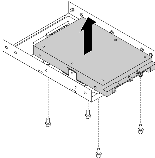
Figure 94. Removing the 2.5-inch storage drive from the storage-drive converter
