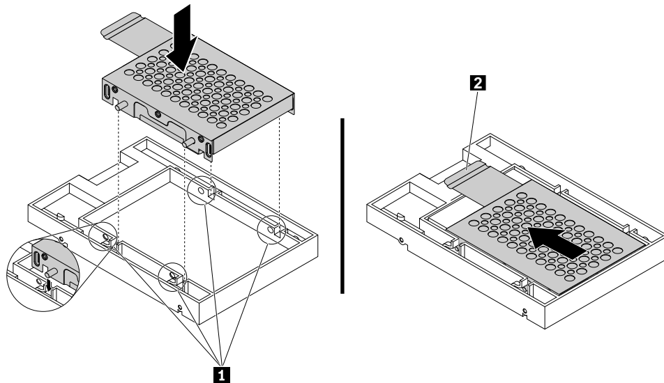
Figure 56. Installing the adapter into the converter
