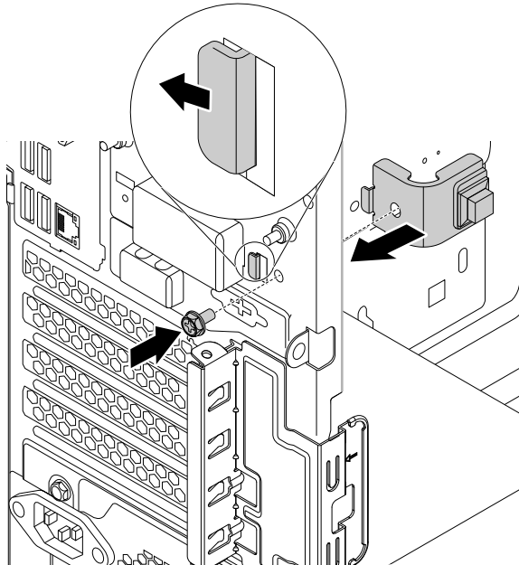
Figure 75. Installing the cover presence switch
