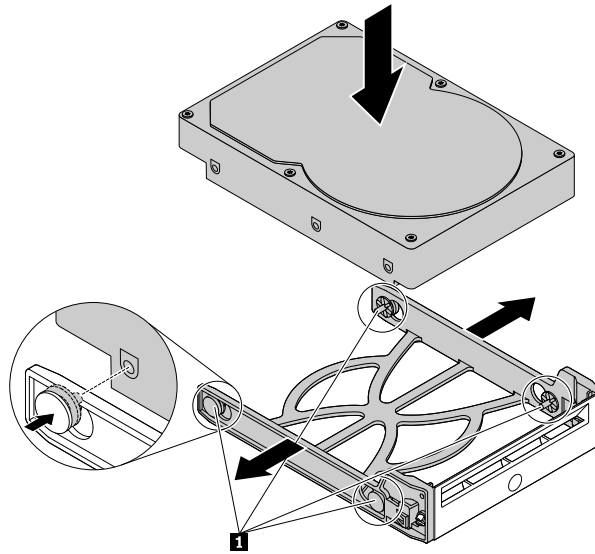
Figure 48. Installing the 3.5-inch storage drive into the bracket
