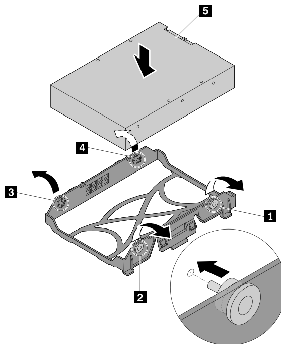
Figure 78. Installing the storage drive into the bracket
