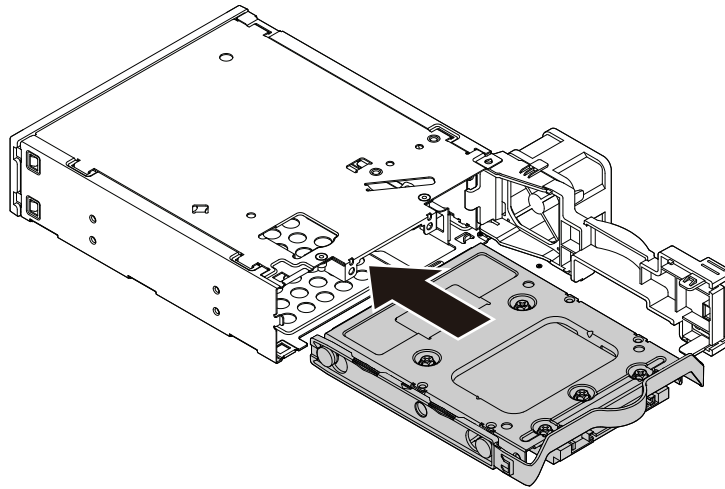
Figure 70. Installing the storage converter with the bracket into the enclosure
