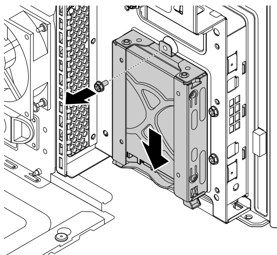
Figure 99. Removing the type-2 storage-drive cage
