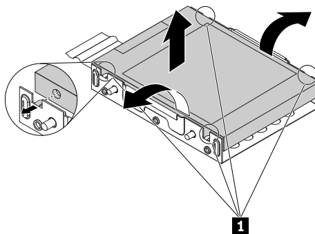
Figure 54. Removing the storage drive from the adapter
