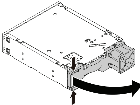
Figure 64. Opening the enclosure from the rear
