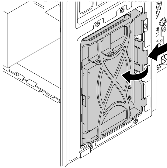
Figure 80. Removing the 2.5-inch storage drive with 3.5-inch storage-drive bracket
