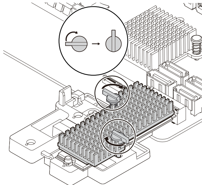
Figure 31. Securing the heat sink to the plastic holder
