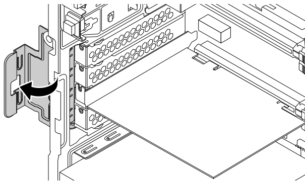
Figure 21. Rotating the PCIe card retainer
