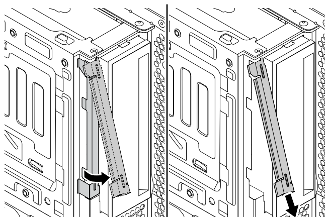
Figure 17. Removing the metal shield
