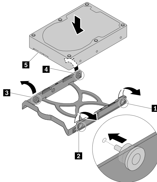
Figure 88. Installing the storage drive into the bracket
