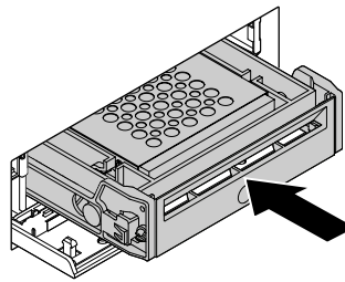
Figure 58. Installing the plastic bracket with the 2.5-inch storage drive into the front-access storage enclosure
