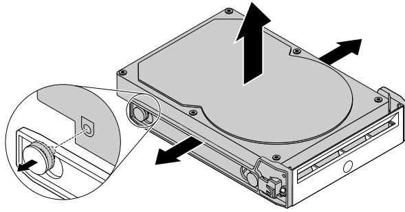
Figure 47. Removing the 3.5-inch storage drive from the bracket
