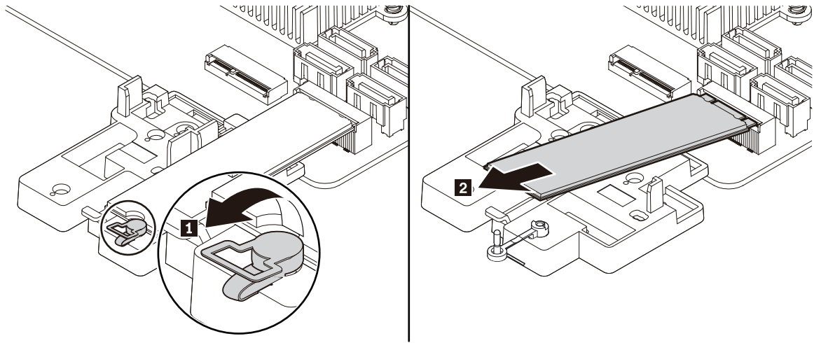
Figure 26. Opening the retention latch and removing the M.2 solid-state drive
