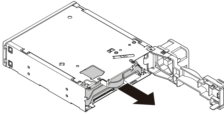
Figure 65. Removing the 2.5-inch storage drive from the rear
