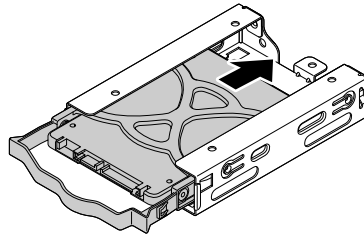
Figure 102. Installing the 2.5-inch storage drive into the type-2 storage-drive cage
