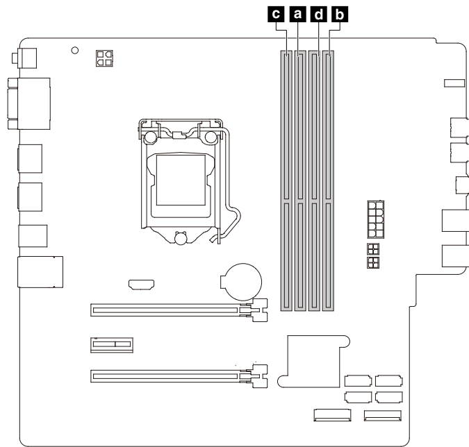
Figure 37. Memory module installation sequence
