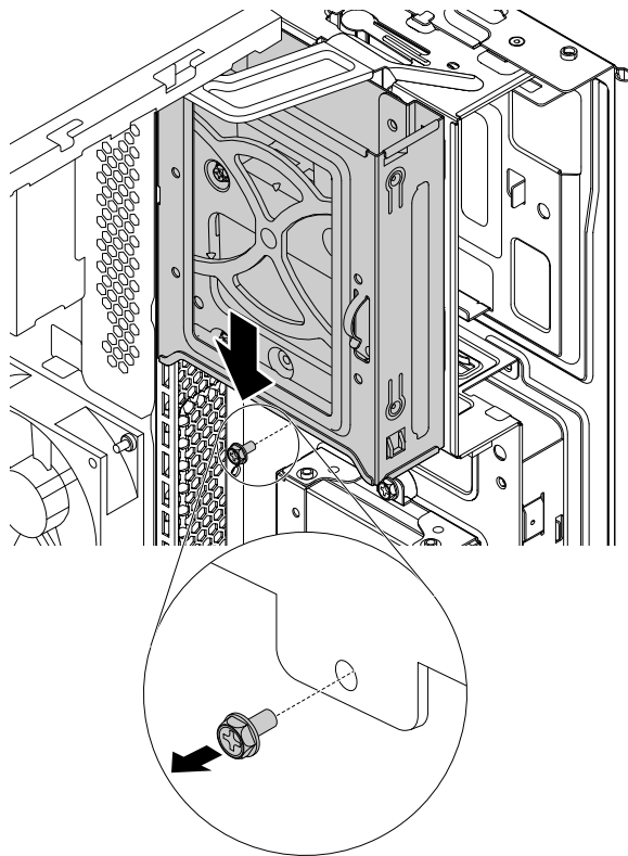
Figure 91. Removing the type-1 storage-drive cage
