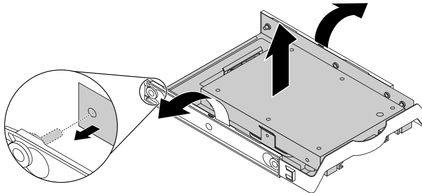
Figure 81. Removing the storage-drive converter from the 3.5-inch storage-drive bracket
