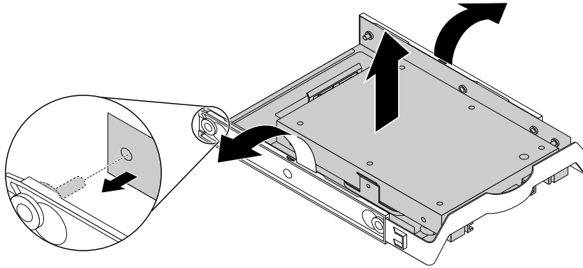
Figure 93. Removing the storage-drive converter from the storage-drive bracket
