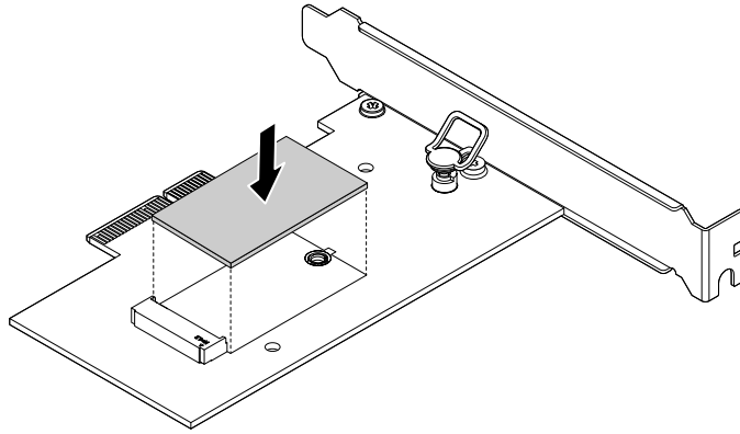
Figure 34. Installing the thermal pad
