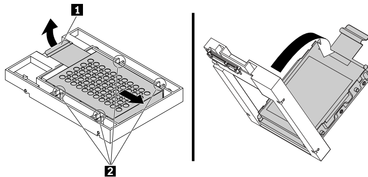
Figure 53. Removing the adapter from the converter
