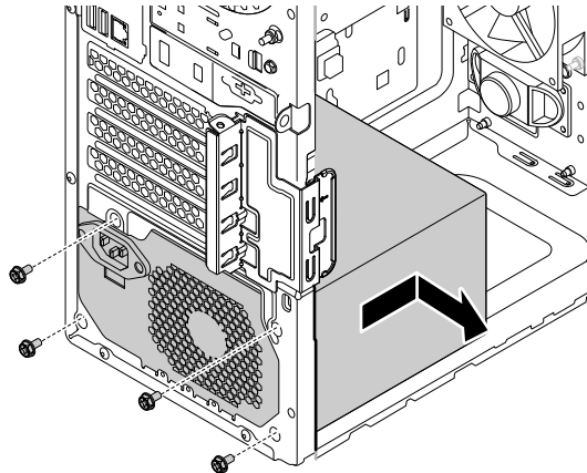
Figure 76. Removing the power supply assembly
