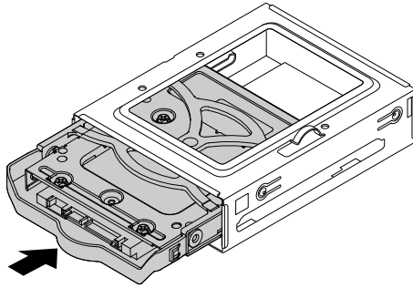
Figure 97. Installing the 2.5-inch storage drive into the type-1 storage-drive cage
