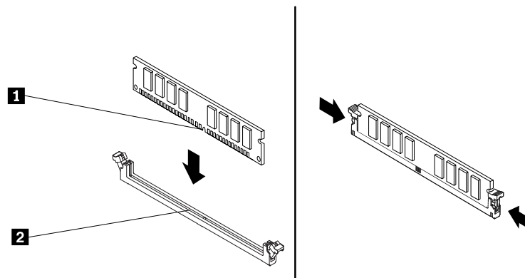
Figure 40. Installing a memory module
