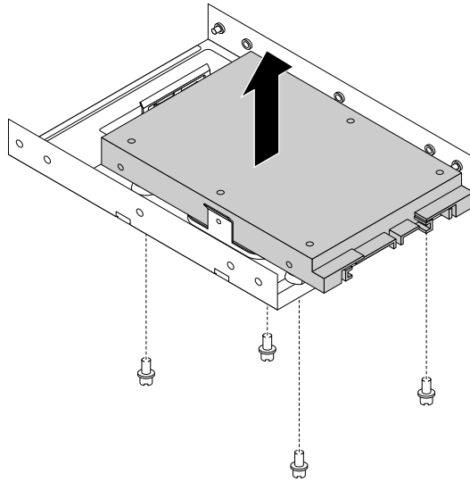
Figure 82. Removing the 2.5-inch storage drive from the storage-drive converter
