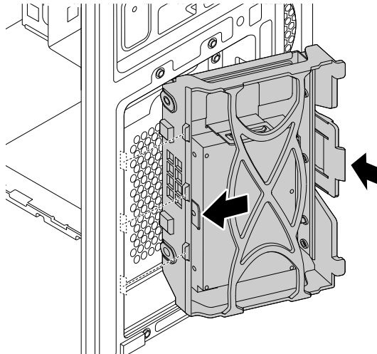
Figure 85. Installing the 2.5-inch storage drive
