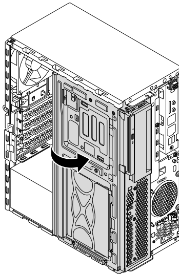
Figure 13. Pivoting the drive bay assembly outward
