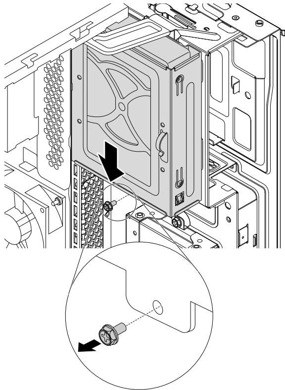
Figure 86. Removing the type-1 storage-drive cage
