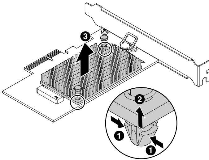
Figure 32. Removing the heat sink from the M.2 solid-state drive adapter
