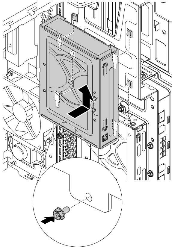
Figure 90. Installing the type-1 storage-drive cage
