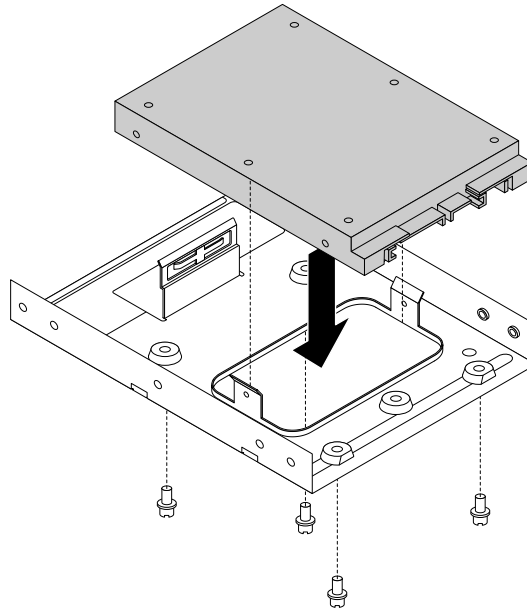
Figure 95. Installing the 2.5-inch storage drive into the storage-drive converter
