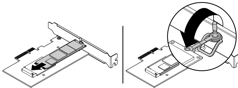
Figure 35. Installing the M.2 solid-state drive
