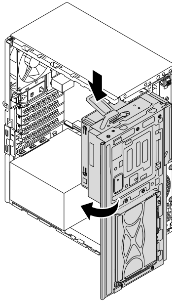
Figure 104. Pivoting the drive bay assembly downward
