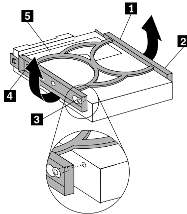
Figure 61. Installing the 3.5-inch storage drive into the bracket
