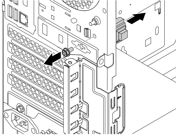
Figure 74. Removing the cover presence switch
