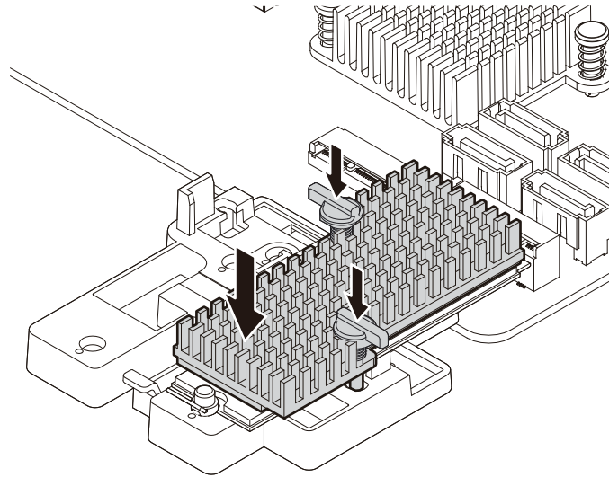
Figure 30. Installing the heat sink onto the plastic holder
