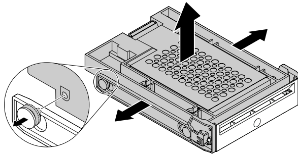
Figure 52. Removing the 2.5-inch storage drive from the bracket
