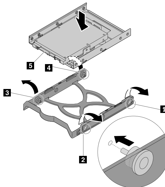
Figure 96. Installing the 2.5-inch storage drive into the bracket
