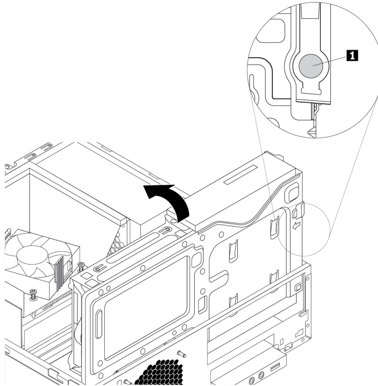
Figure 96. Pivoting the drive bay assembly downward
