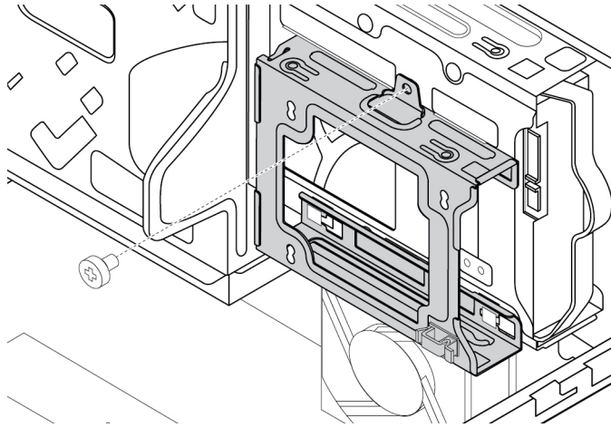
Figure 93. Installing the screw to secure the secondary hard disk drive cage
