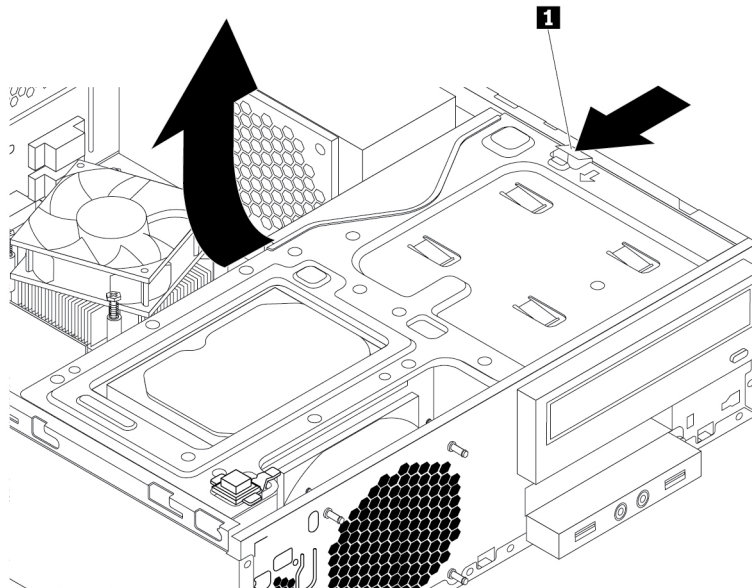
Figure 80. Pivoting the drive bay assembly upward
