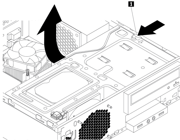
Figure 27. Pivoting the drive bay assembly upward
