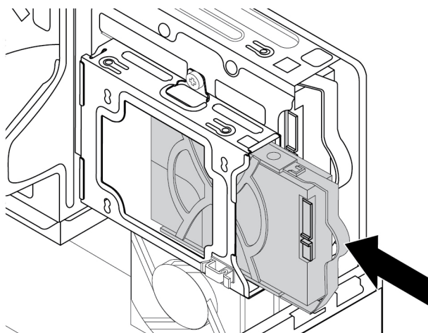
Figure 95. Installing the secondary hard disk drive
