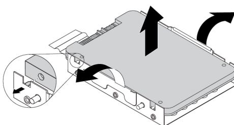
Figure 40. Removing the storage drive from the metal bracket
