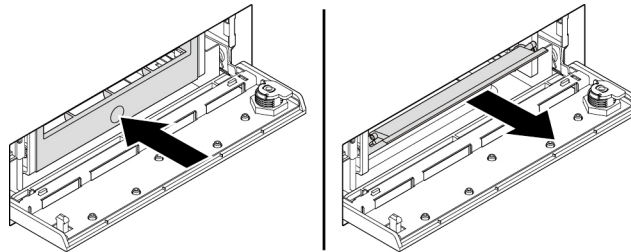
Figure 37. Removing the bracket from the front-access storage enclosure
