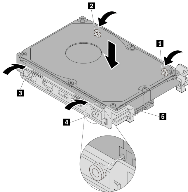
Figure 53. Installing the new 3.5-inch internal storage drive into the bracket
