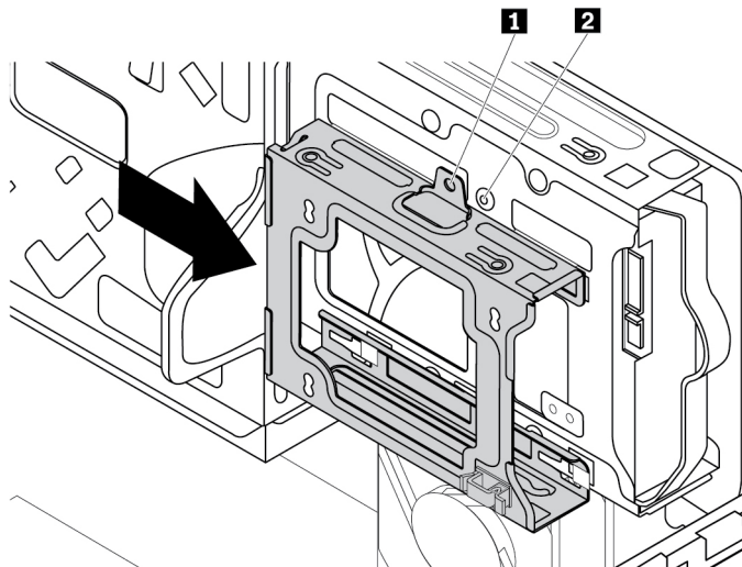
Figure 92. Installing the secondary hard-disk-drive cage
