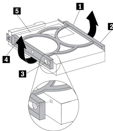
Figure 94. Installing the hard disk drive into the bracket
