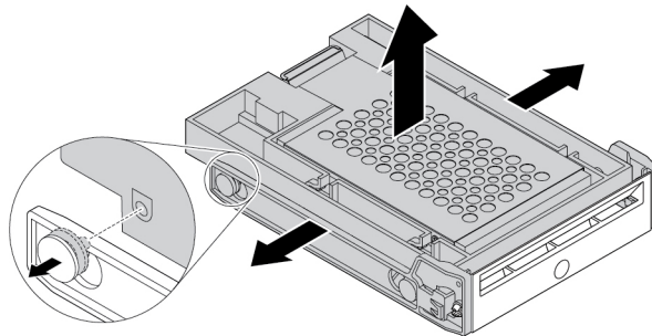
Figure 38. Removing the 2.5-inch storage drive from the bracket
