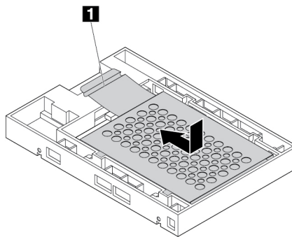
Figure 43. Installing the metal bracket into the plastic frame of the converter
