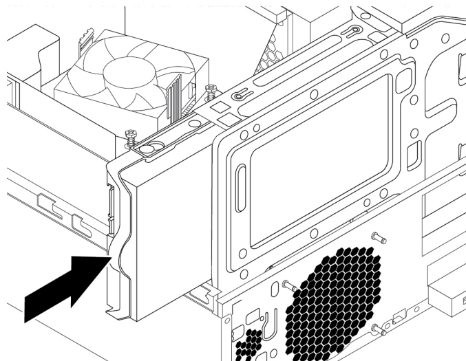
Figure 88. Installing the primary hard disk drive
