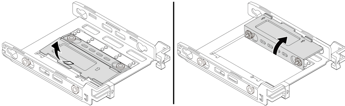
Figure 64. Folding the bracket
