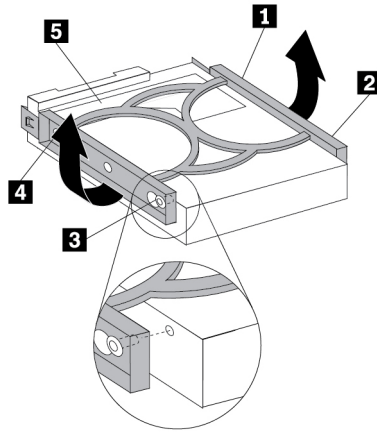
Figure 87. Installing the hard disk drive into the bracket
