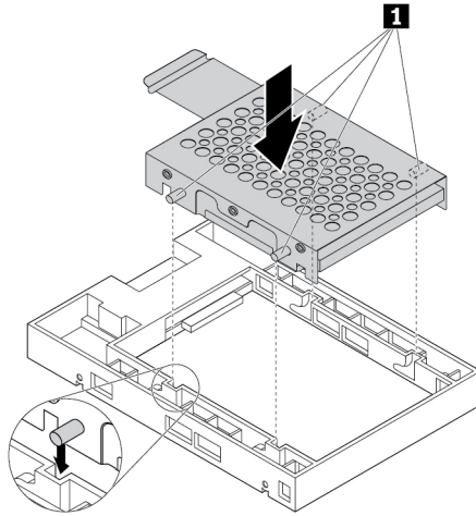
Figure 42. Inserting the metal bracket into the plastic frame of the converter
