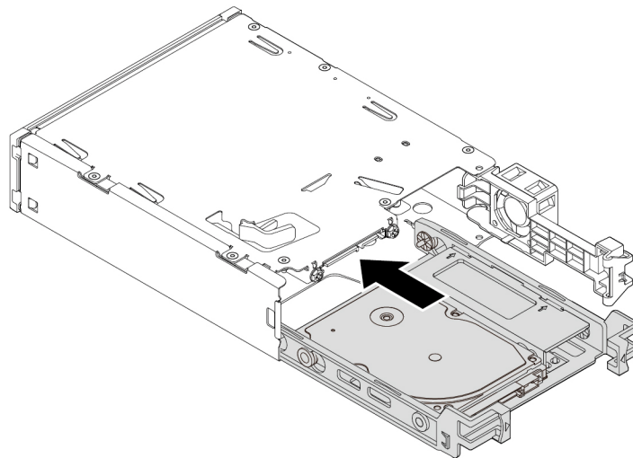
Figure 60. Sliding the new 2.5-inch internal storage drive into the kit
