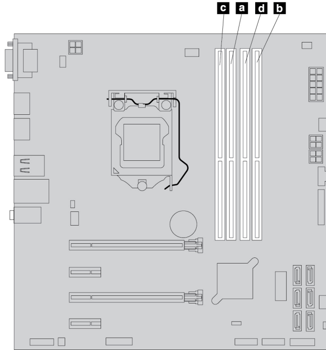
Figure 23. Memory module installation order
