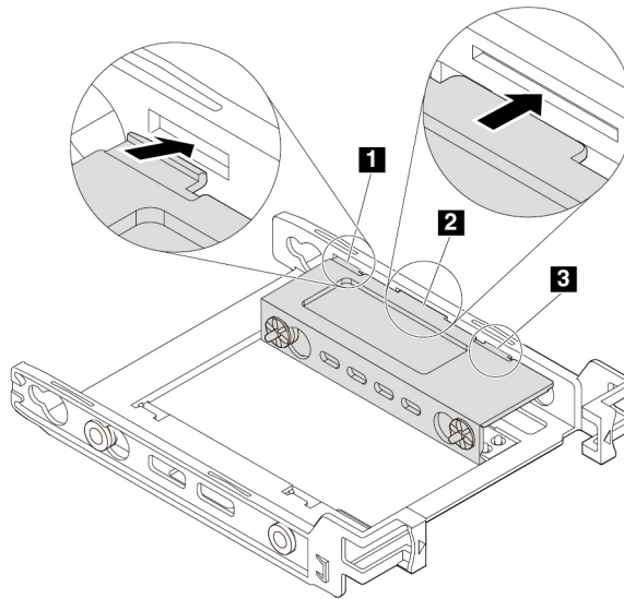
Figure 65. Inserting tabs 1 and 3 into the corresponding slots
