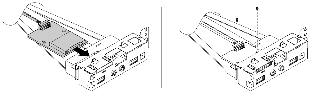
Figure 14. Installing the new card reader
