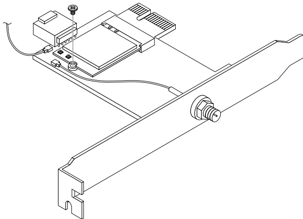
Figure 110. Installing a screw to secure the Wi-Fi card module
