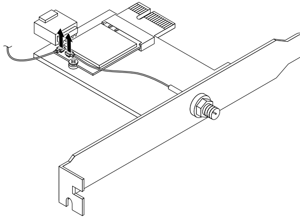
Figure 104. Disconnecting the Wi-Fi antenna cables
