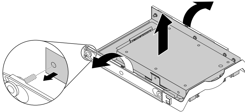
Figure 84. Removing the storage converter from the 3.5-inch hard-disk-drive bracket
