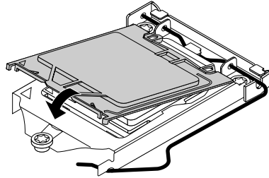
Figure 73. Installing the microprocessor socket cover
