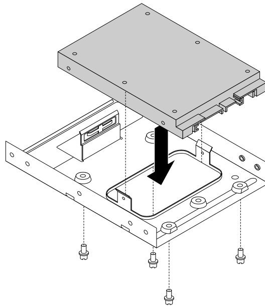
Figure 82. Installing the solid-state drive into the storage converter
