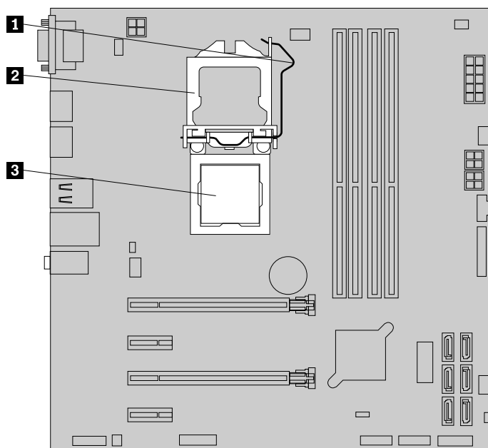
Figure 68. Accessing the microprocessor
