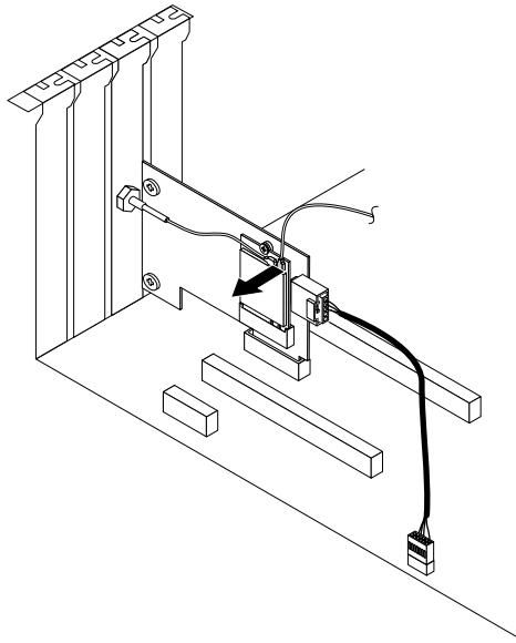
Figure 98. Disconnecting the front Wi-Fi antenna cable
