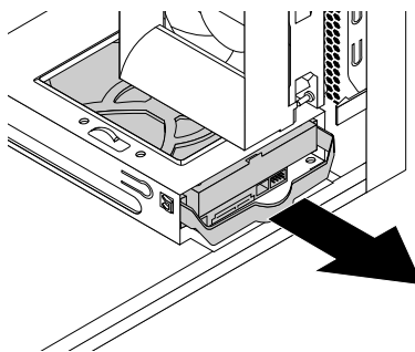
Figure 91. Removing the secondary hard disk drive
