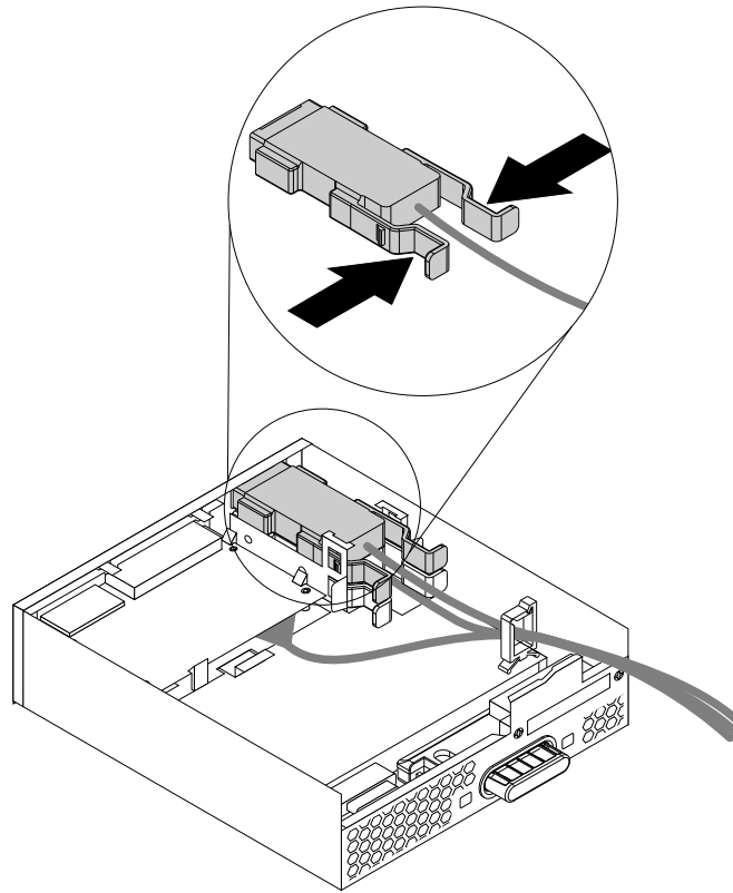
Figure 49. Removing the eSATA connector or IEEE 1394 connector from the flex module
