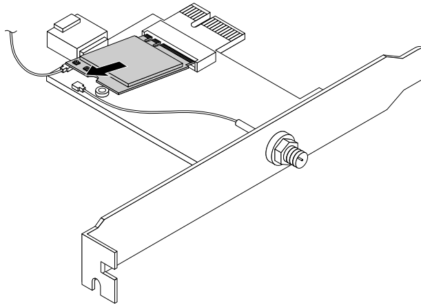
Figure 106. Removing the Wi-Fi card module
