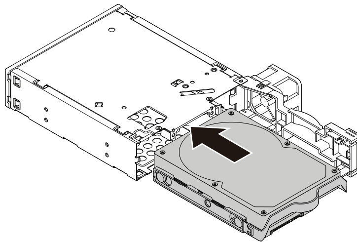
Figure 62. Installing the hard disk drive into the enclosure
