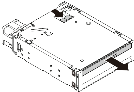
Figure 57. Removing the slim optical drive from the enclosure
