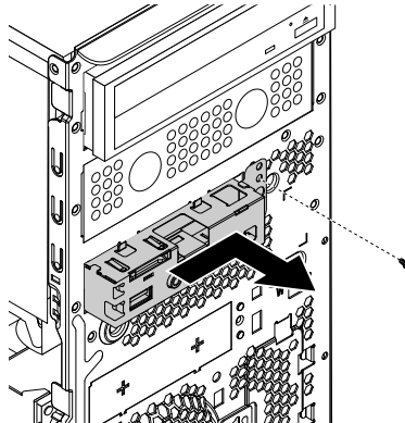
Figure 66. Removing the front audio and USB assembly
