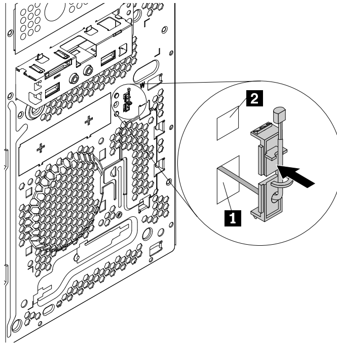
Figure 77. Installing the thermal sensor
