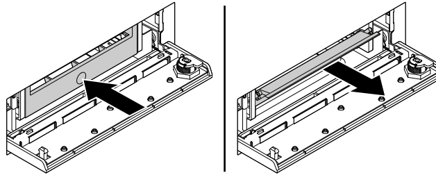
Figure 53. Removing the hard disk drive from the front-access storage enclosure
