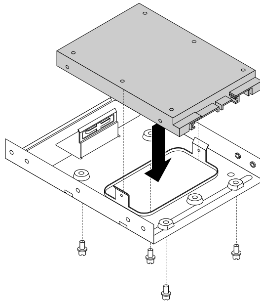
Figure 86. Installing the new solid-state drive into the storage converter
