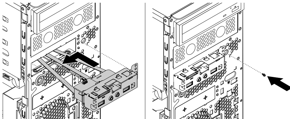
Figure 67. Installing the front audio and USB assembly
