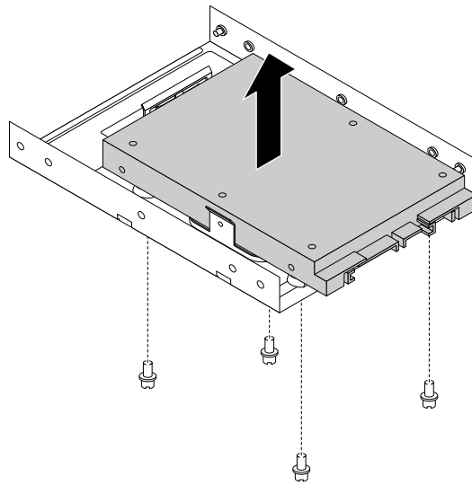
Figure 85. Removing the solid-state drive from the storage converter
