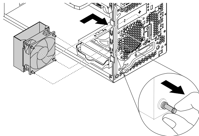
Figure 95. Installing the front fan assembly
