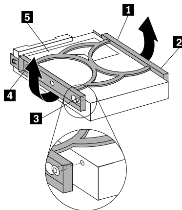
Figure 89. Installing the hard disk drive into the bracket
