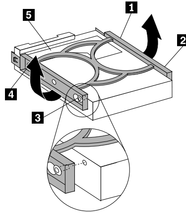
Figure 92. Installing the hard disk drive into the bracket
