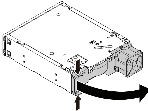
Figure 59. Opening the enclosure from the rear
