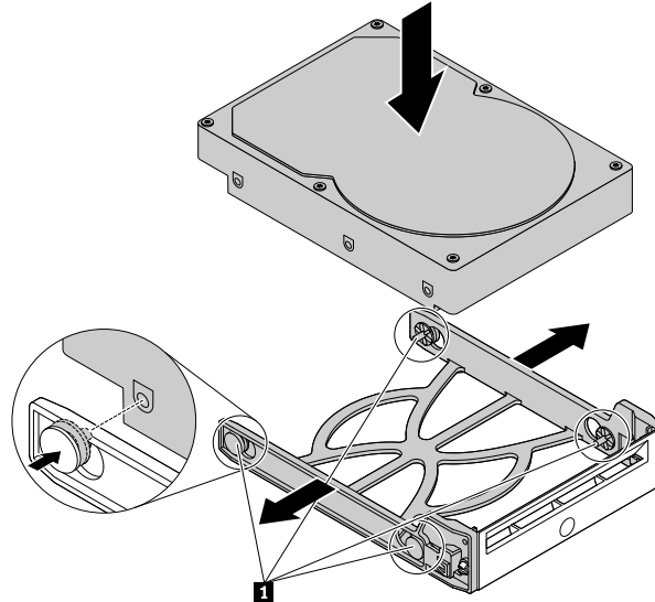
Figure 55. Installing the hard disk drive into the bracket
