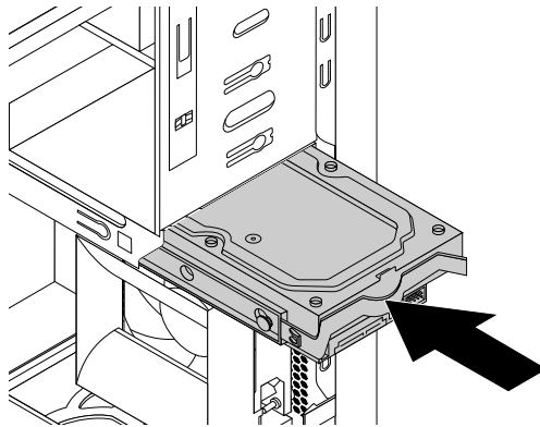
Figure 90. Installing the primary hard disk drive
