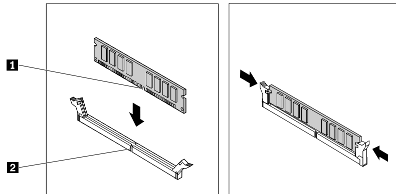
Figure 29. Installing a memory module
