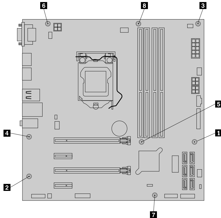
Figure 71. Removing the eight screws that secure the system board
