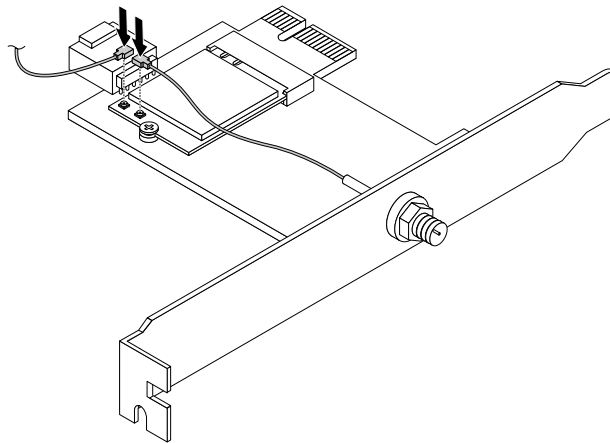
Figure 111. Installing the Wi-Fi antenna cables
