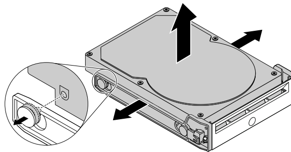
Figure 54. Removing the hard disk drive from the bracket
