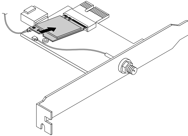
Figure 109. Installing the Wi-Fi card module
