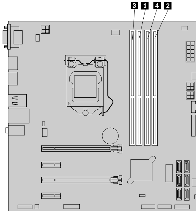
Figure 26. Memory module installation—order
