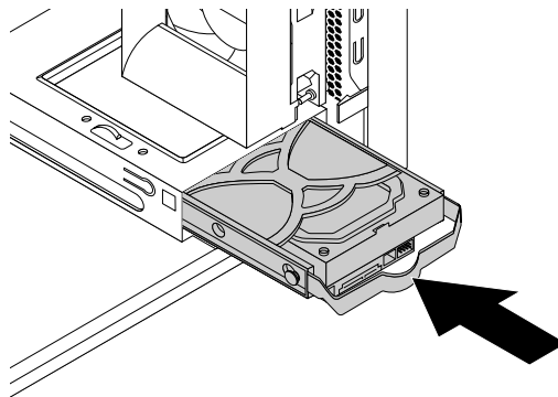
Figure 93. Installing the secondary hard disk drive
