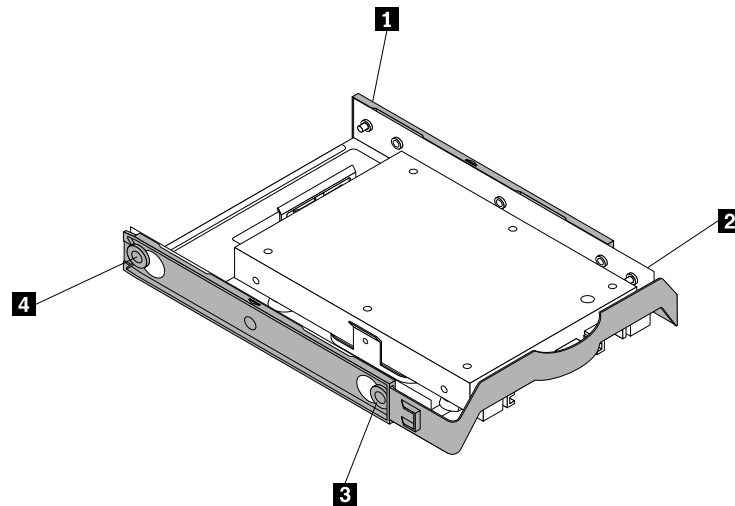
Figure 83. Installing the storage converter together with the solid-state drive into the hard-disk-drive bracket
