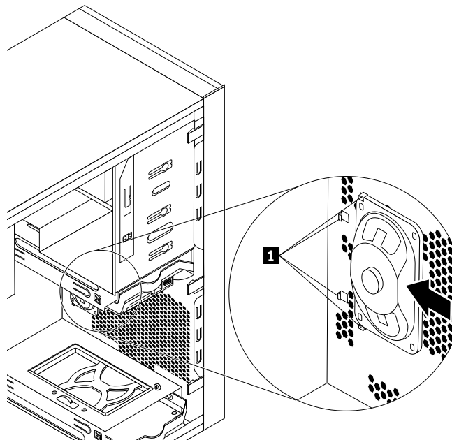
Figure 75. Installing the internal speaker
