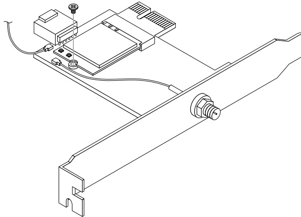
Figure 105. Removing the screw that secures the Wi-Fi card module
