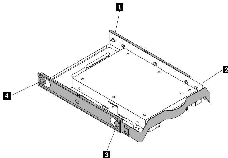
Figure 87. Installing the storage converter with the new solid-state drive into the hard-disk-drive bracket
