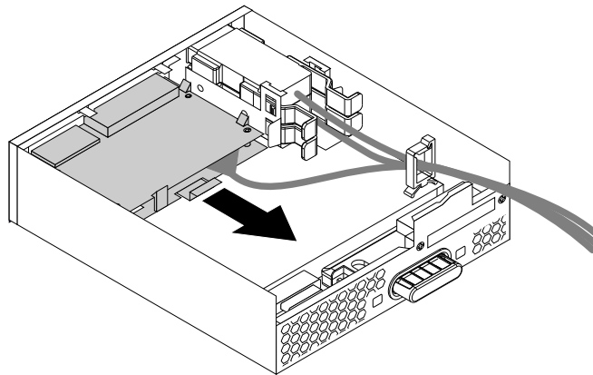
Figure 43. Removing the card reader from the flex module
