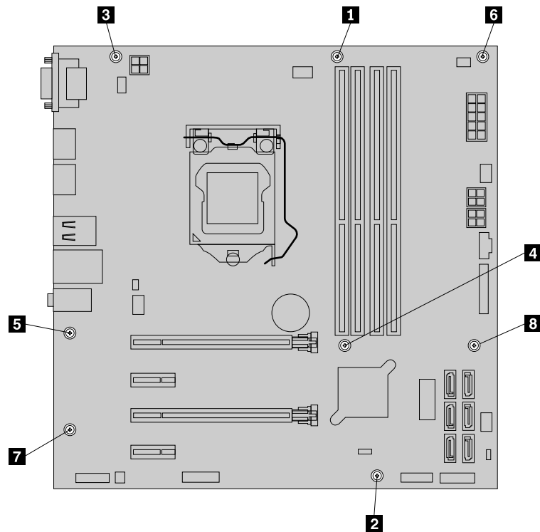
Figure 72. Installing the eight screws to secure the system board
