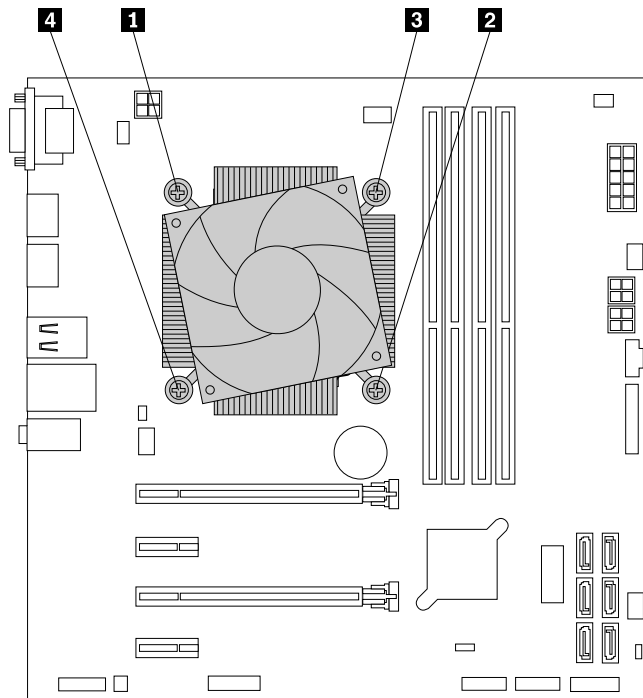
Figure 81. Removing the heat sink and fan assembly
