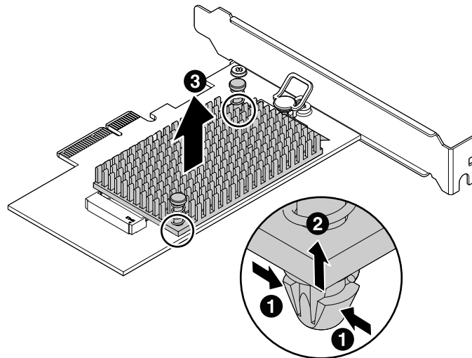
Figure 21. Removing the heat sink from the M.2 solid-state drive adapter
