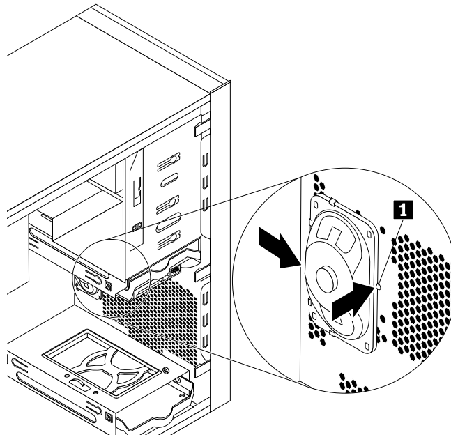
Figure 74. Removing the old internal speaker
