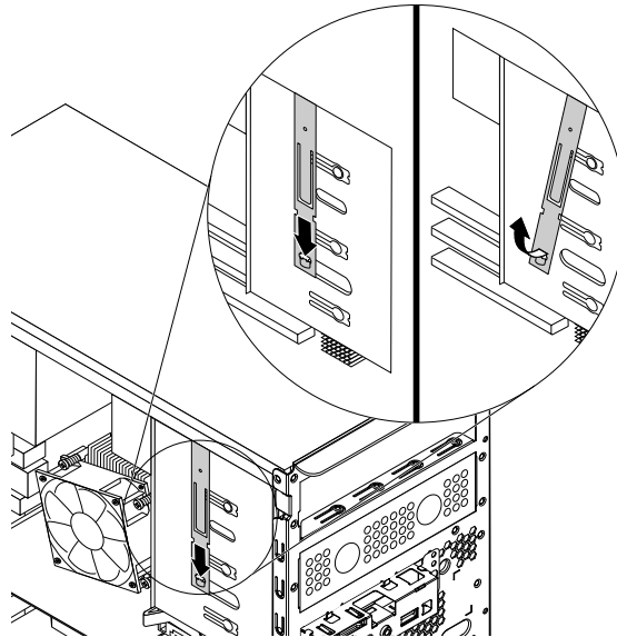
Figure 30. Removing the optical drive retainer from the computer
