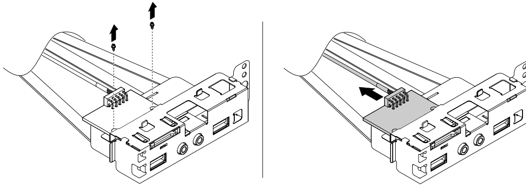
Figure 13. Removing the card reader
