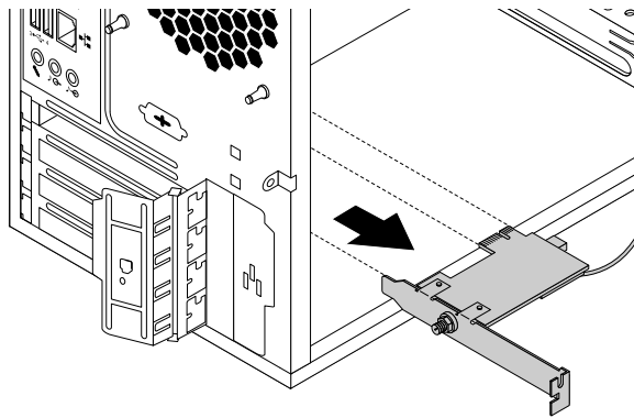
Figure 103. Removing the Wi-Fi adapter card
