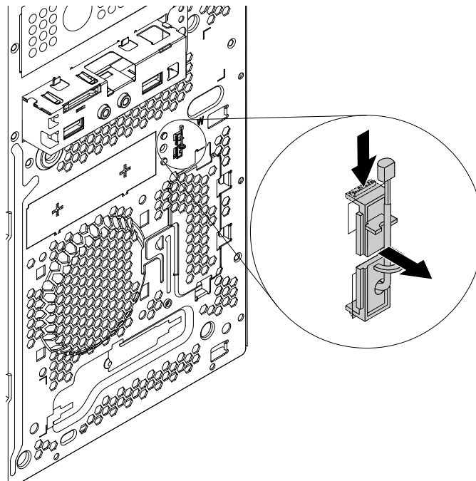
Figure 76. Removing the thermal sensor
