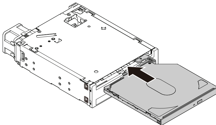
Figure 58. Installing the slim optical drive in the enclosure
