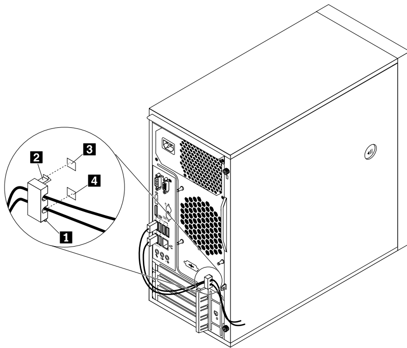
Figure 10. Installing a cable lock
