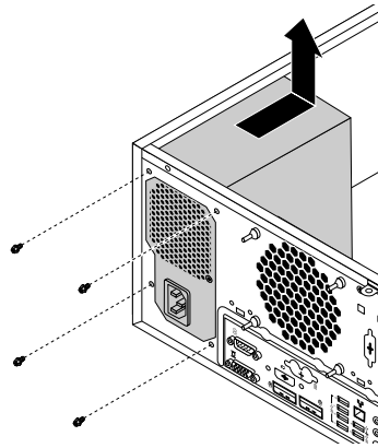
Figure 33. Removing the screws that secure the power supply assembly
