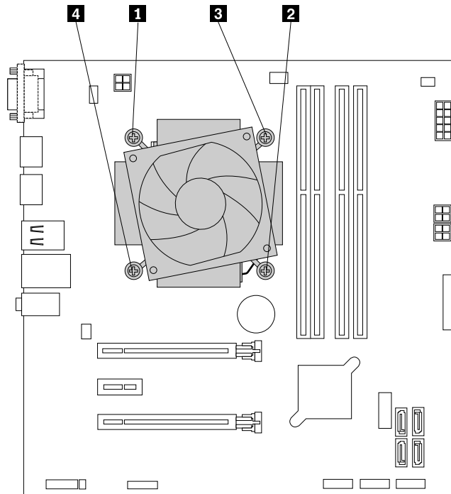
Figure 34. Removing the heat sink and fan assembly
