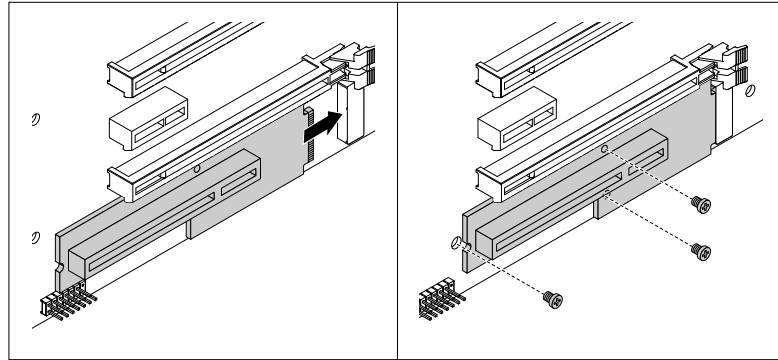
Figure 41. Installing a PCI adapter card
