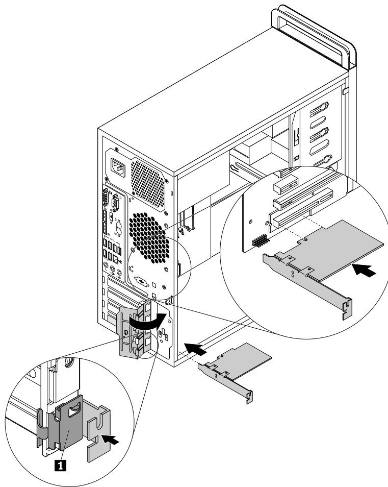
Figure 39. Installing the PCI card
