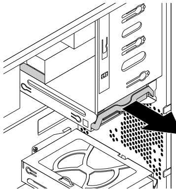
Figure 19. Removing the 3.5-inch storage drive bracket
