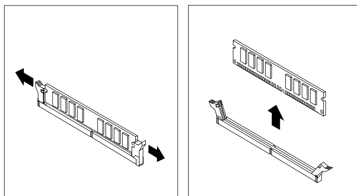
Figure 35. Removing a memory module
