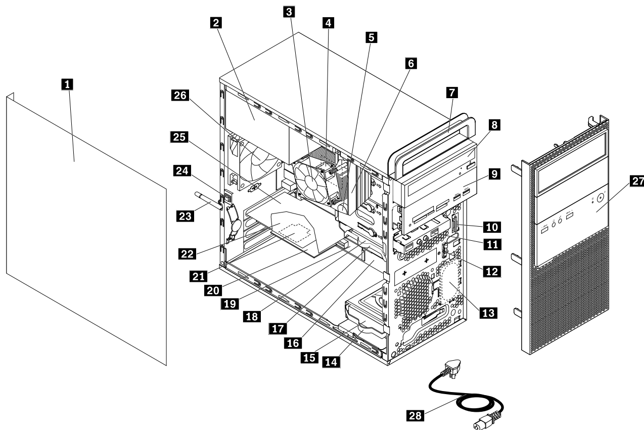
Figure 3. Computer components
