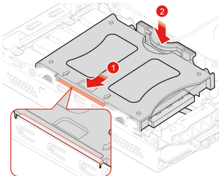
Figure 20. Installing the storage drive bracket
