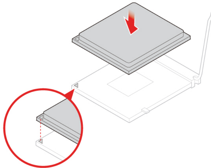
Figure 35. Installing the microprocessor
