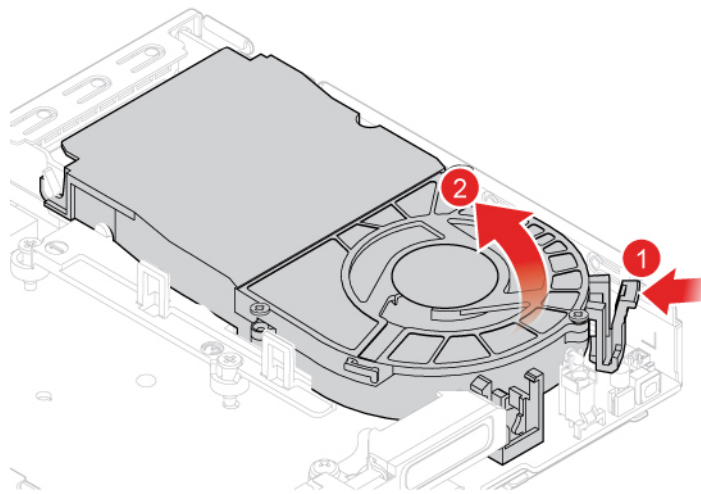
Figure 25. Removing the system fan
