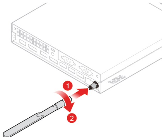
Figure 57. Installing the antenna cover to secure the rear Wi-Fi antenna cable
