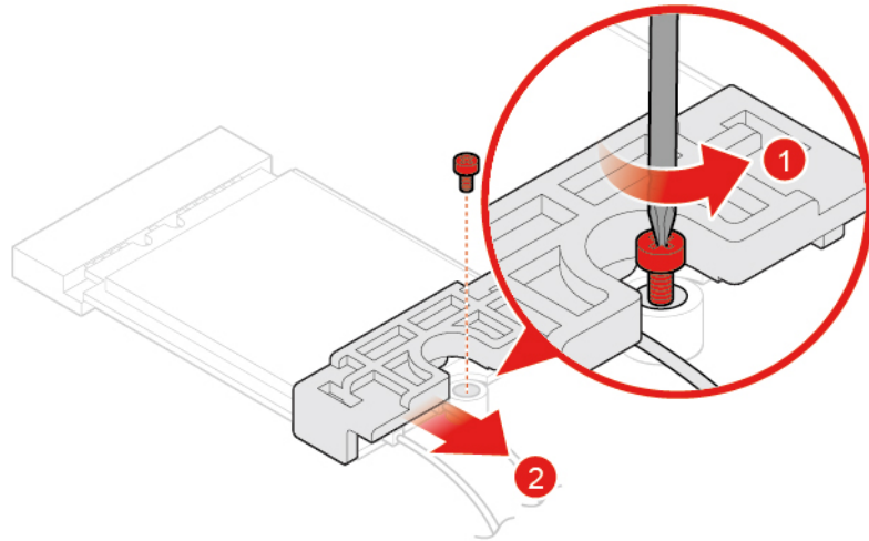
Figure 37. Removing the Wi-Fi card shield
