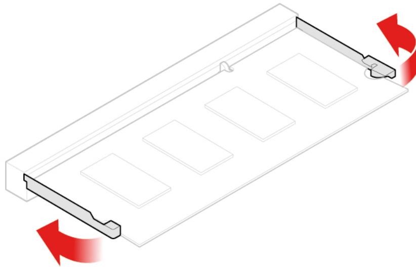
Figure 63. Opening the memory module retainer
