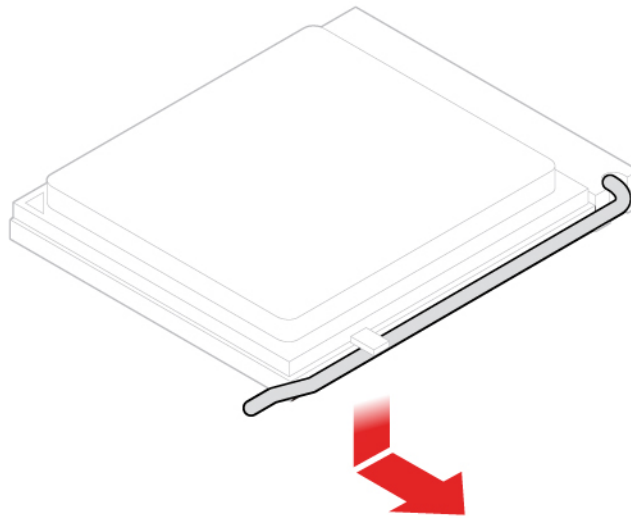
Figure 33. Unlocking the microprocessor socket retainer
