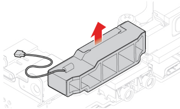
Figure 50. Removing the front Wi-Fi antenna
