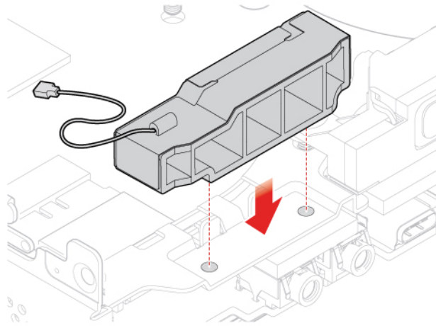
Figure 51. Installing the front Wi-Fi antenna
