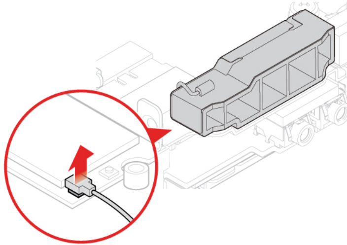
Figure 49. Disconnecting the front Wi-Fi antenna cable from the Wi-Fi card
