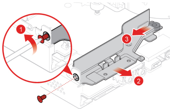
Figure 59. Removing the antenna bracket
