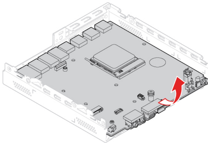
Figure 72. Removing the system board
