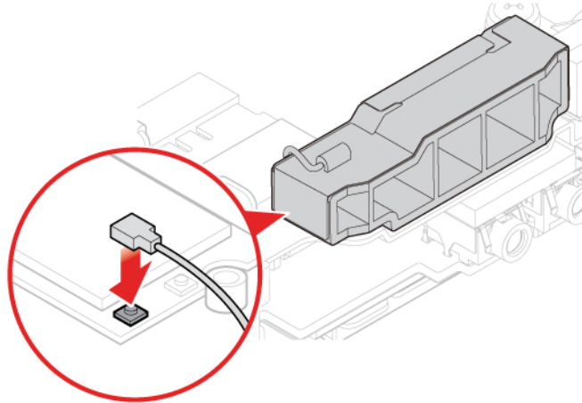
Figure 52. Connecting the front Wi-Fi antenna cable to the Wi-Fi card
