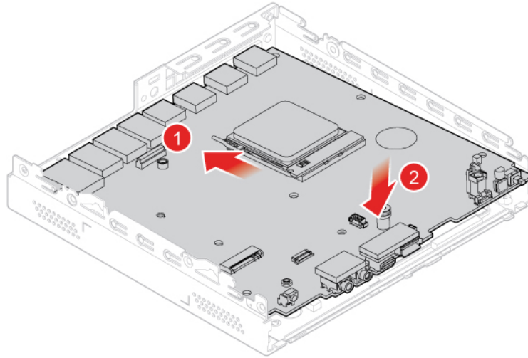
Figure 73. Installing the system board
