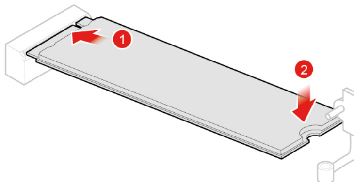
Figure 69. Installing the M.2 solid-state drive
