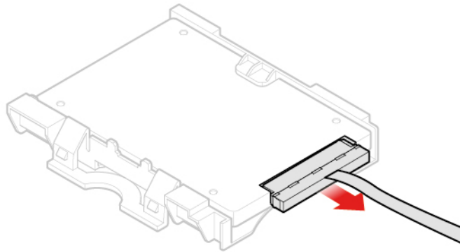
Figure 21. Removing the storage drive cable
