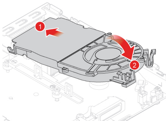
Figure 26. Installing the system fan
