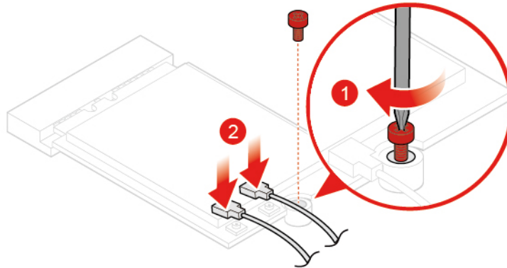
Figure 41. Connecting the Wi-Fi antennas
