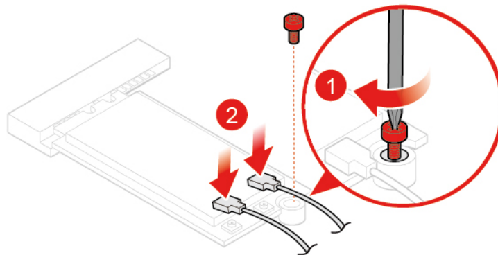
Figure 47. Connecting the Wi-Fi antennas
