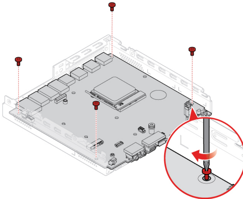
Figure 74. Installing the screws to secure the system board
