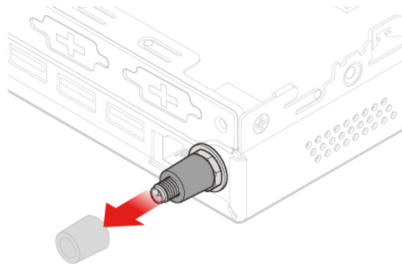
Figure 54. Removing the antenna cover that secures the rear Wi-Fi antenna cable
