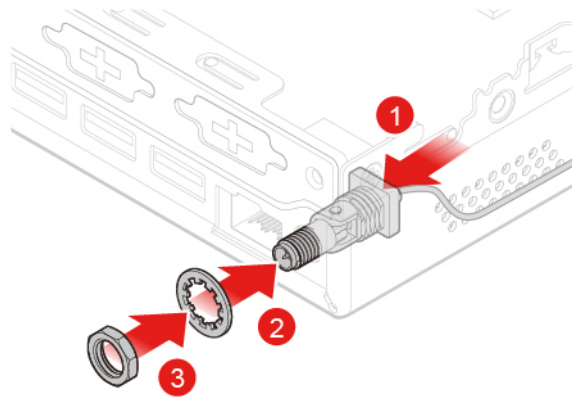
Figure 56. Installing the rear Wi-Fi antenna cable
