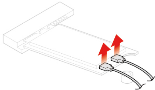
Figure 44. Disconnecting the Wi-Fi antennas
