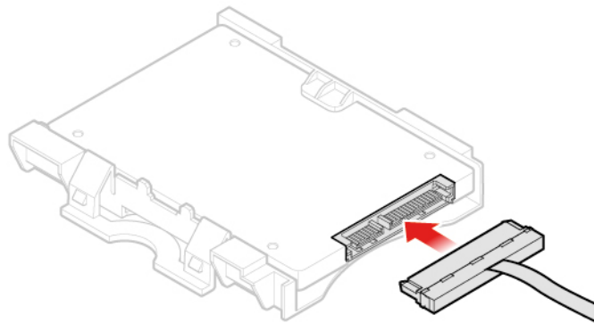
Figure 22. Installing the storage drive cable
