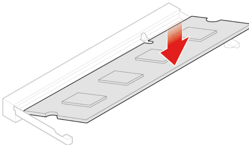
Figure 66. Closing the memory module retainer
