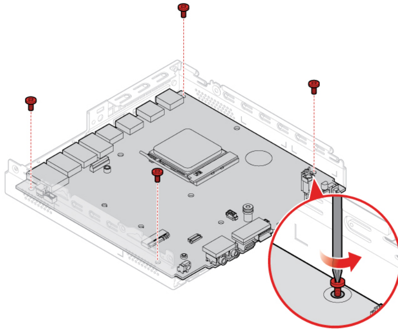
Figure 71. Removing the screws that secure the system board
