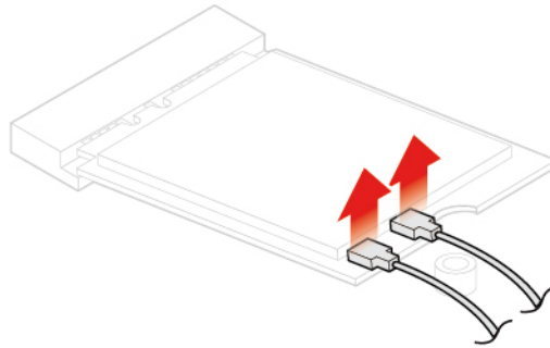
Figure 38. Disconnecting the Wi-Fi antennas
