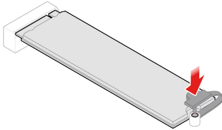
Figure 70. Locking the M.2 solid-state drive clip
