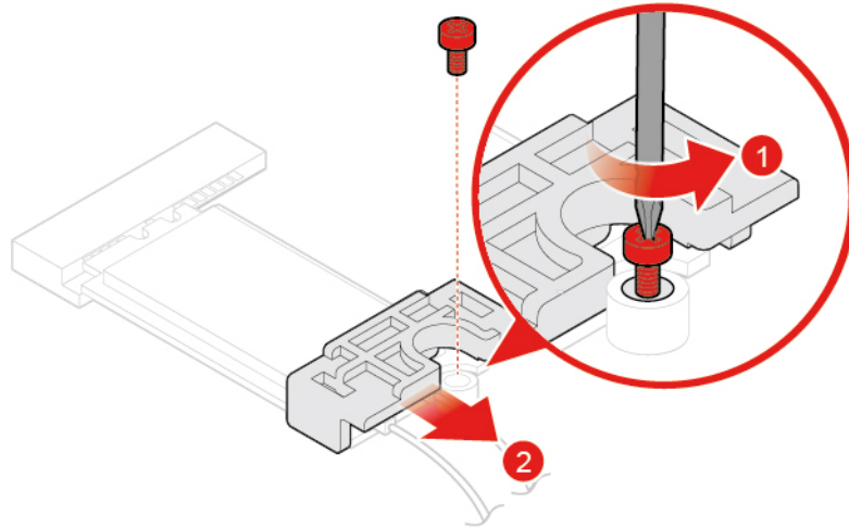
Figure 43. Removing the Wi-Fi card shield
