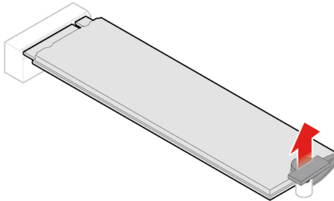
Figure 67. Unlocking the M.2 solid-state drive clip
