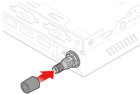
Figure 56. Installing the rear Wi-Fi antenna cable
