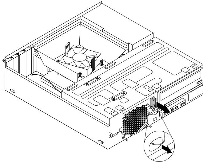
Figure 57. Removing the front WiFi antenna
