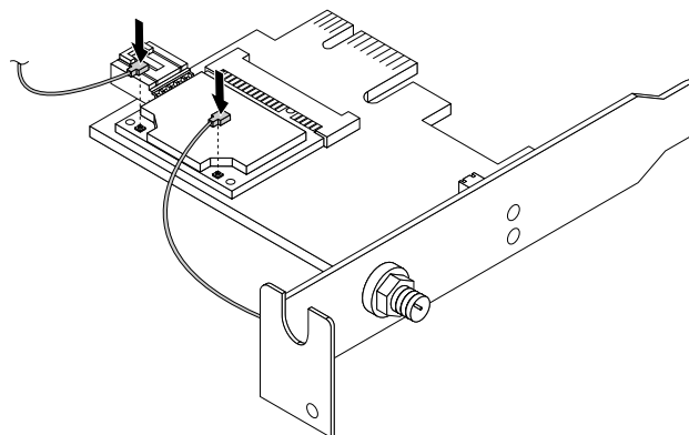
Figure 51. Connecting the WiFi antenna cables
