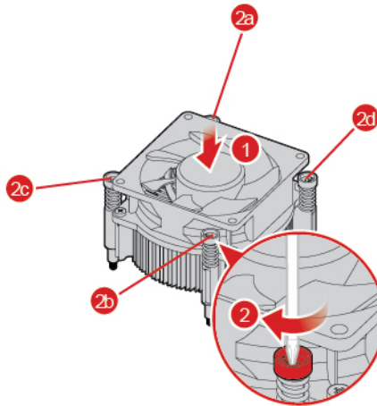
Figure 48. Installing the heat sink and fan assembly
