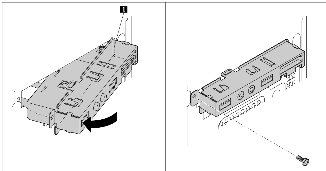
Figure 32. Installing the front audio and USB 3.0 assembly
