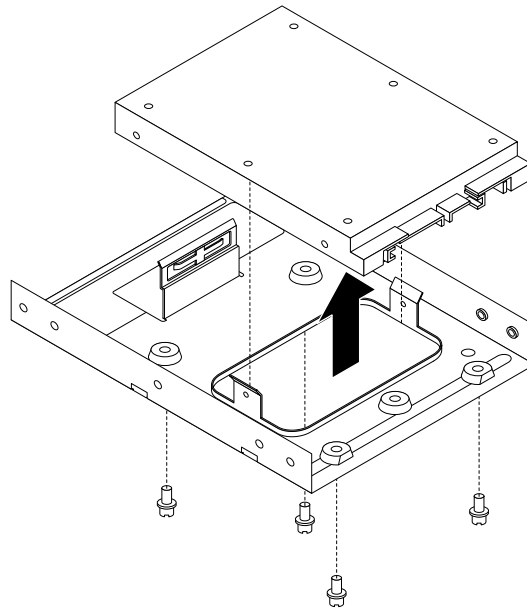
Figure 12. Removing the 2.5-inch storage drive from the storage converter
