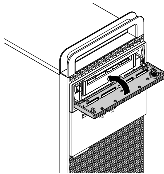
Figure 19. Securing the 3.5-inch storage drive bracket
