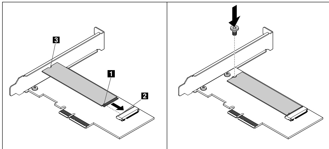
Figure 21. Installing the M.2 solid-state drive
