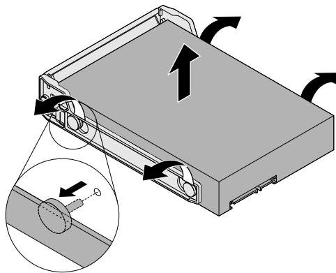
Figure 16. Removing the 3.5-inch storage drive from the bracket
