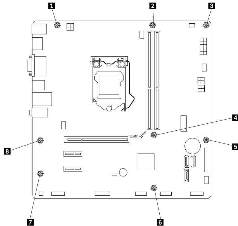
Figure 59. Removing the system board
