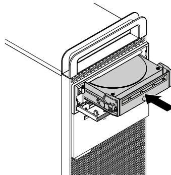
Figure 18. Installing the 3.5-inch storage drive bracket into the front-access storage enclosure
