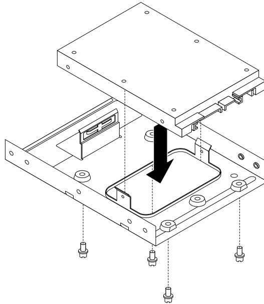
Figure 13. Installing the 2.5-inch storage drive into the storage converter
