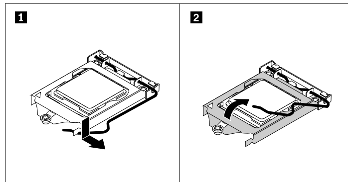
Figure 56. Accessing the microprocessor
