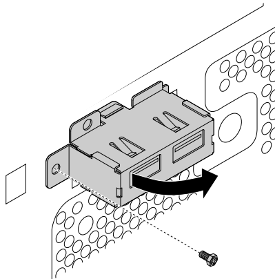
Figure 33. Removing the USB 2.0 assembly bracket
