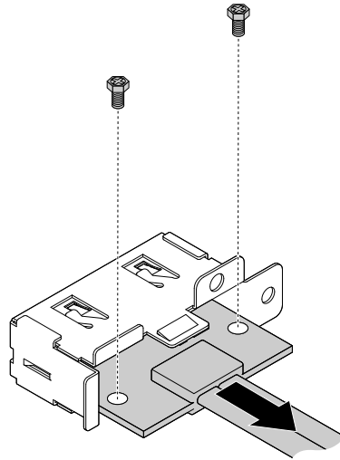
Figure 34. Removing the USB 2.0 assembly from the bracket
