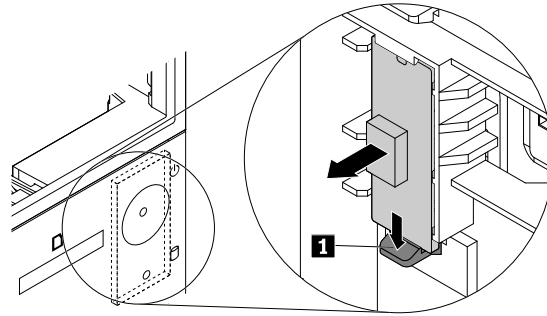
Figure 24. Removing the power button board from the front bezel
