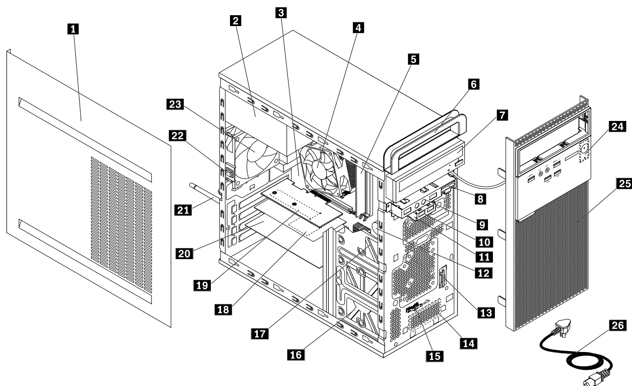
Figure 3. Computer components
