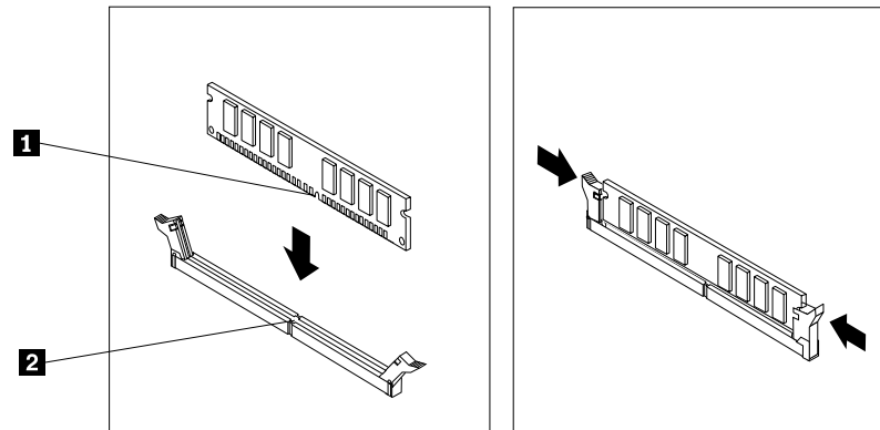
Figure 52. Installing a memory module
