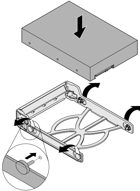
Figure 17. Installing the 3.5-inch storage drive into the bracket
