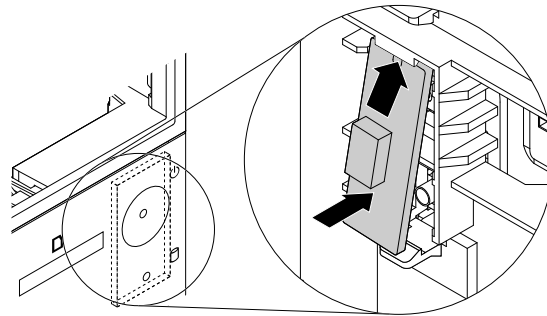
Figure 25. Installing the power button board to the front bezel
