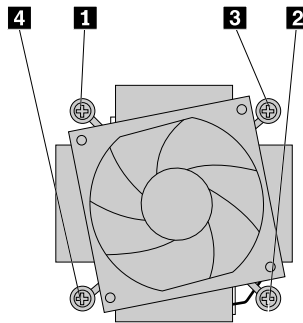
Figure 55. Removing the heat sink and fan assembly
