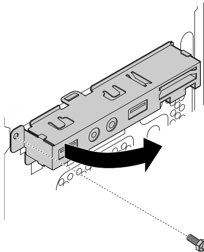
Figure 30. Removing the front audio and USB 3.0 assembly
