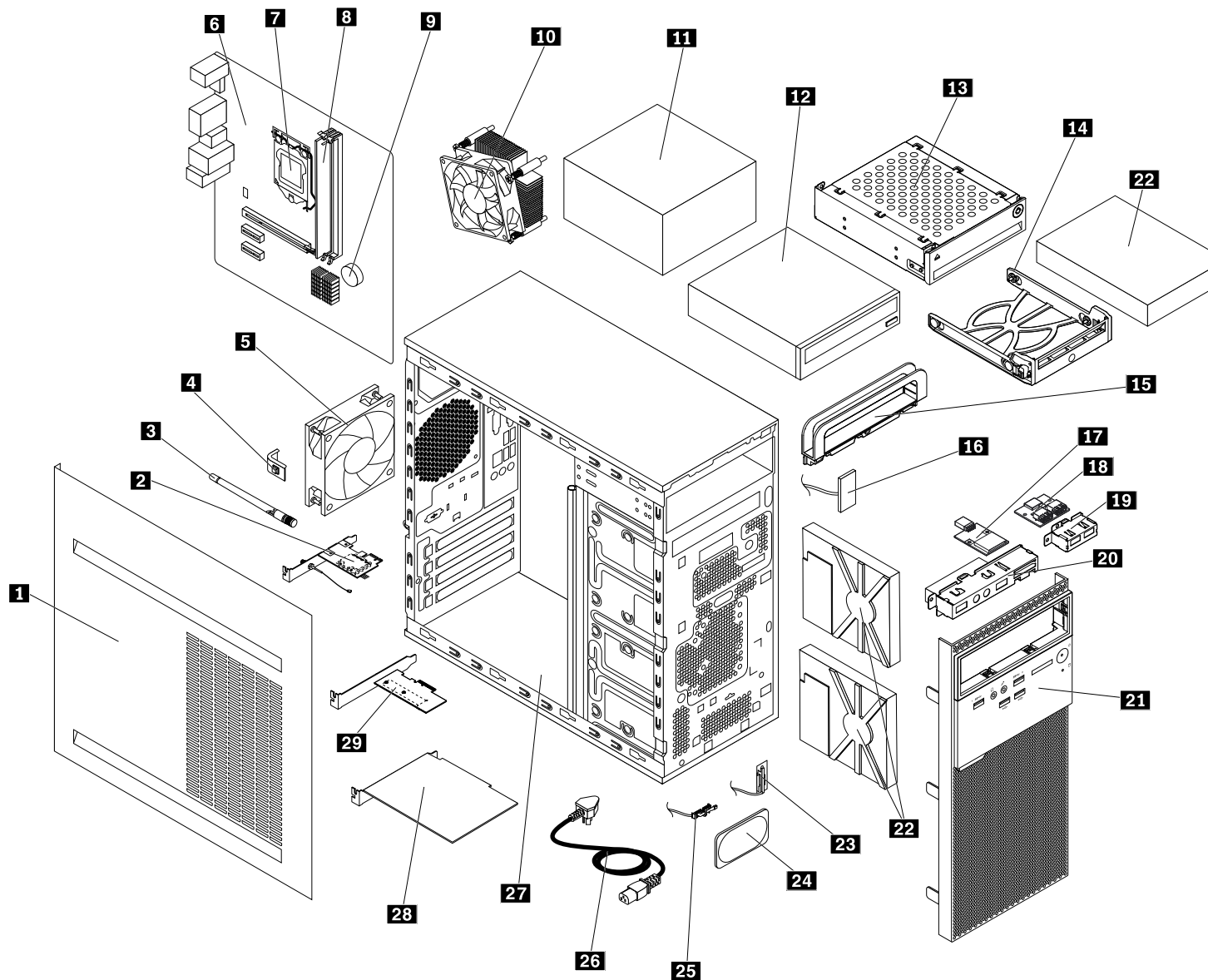
Figure 4. Major FRUs and CRUs
