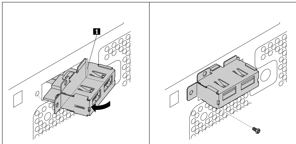
Figure 35. Installing the USB 2.0 assembly bracket
