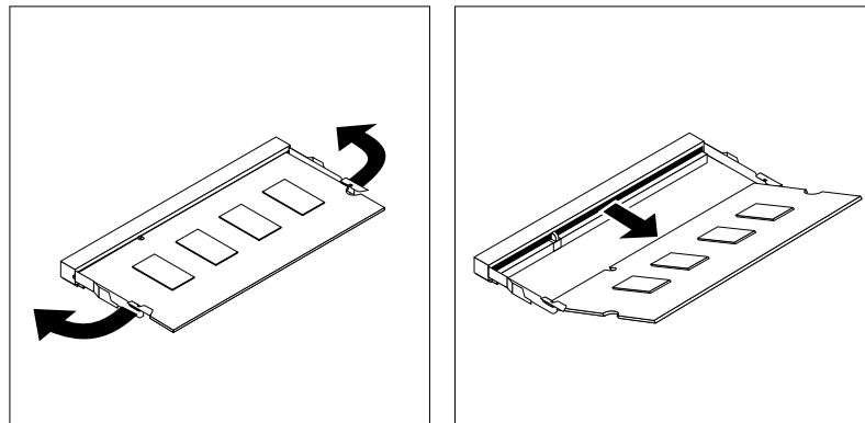
Figure 46. Removing the memory module
