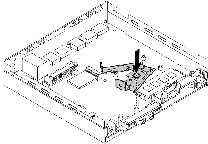
Figure 81. Installing the antenna bracket
