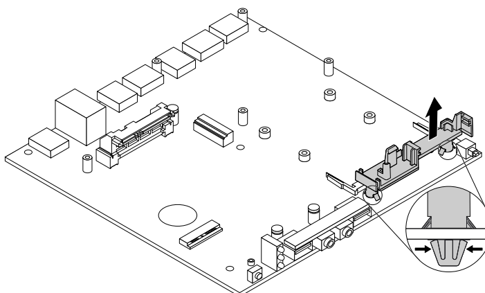
Figure 84. Removing the internal speaker holder
