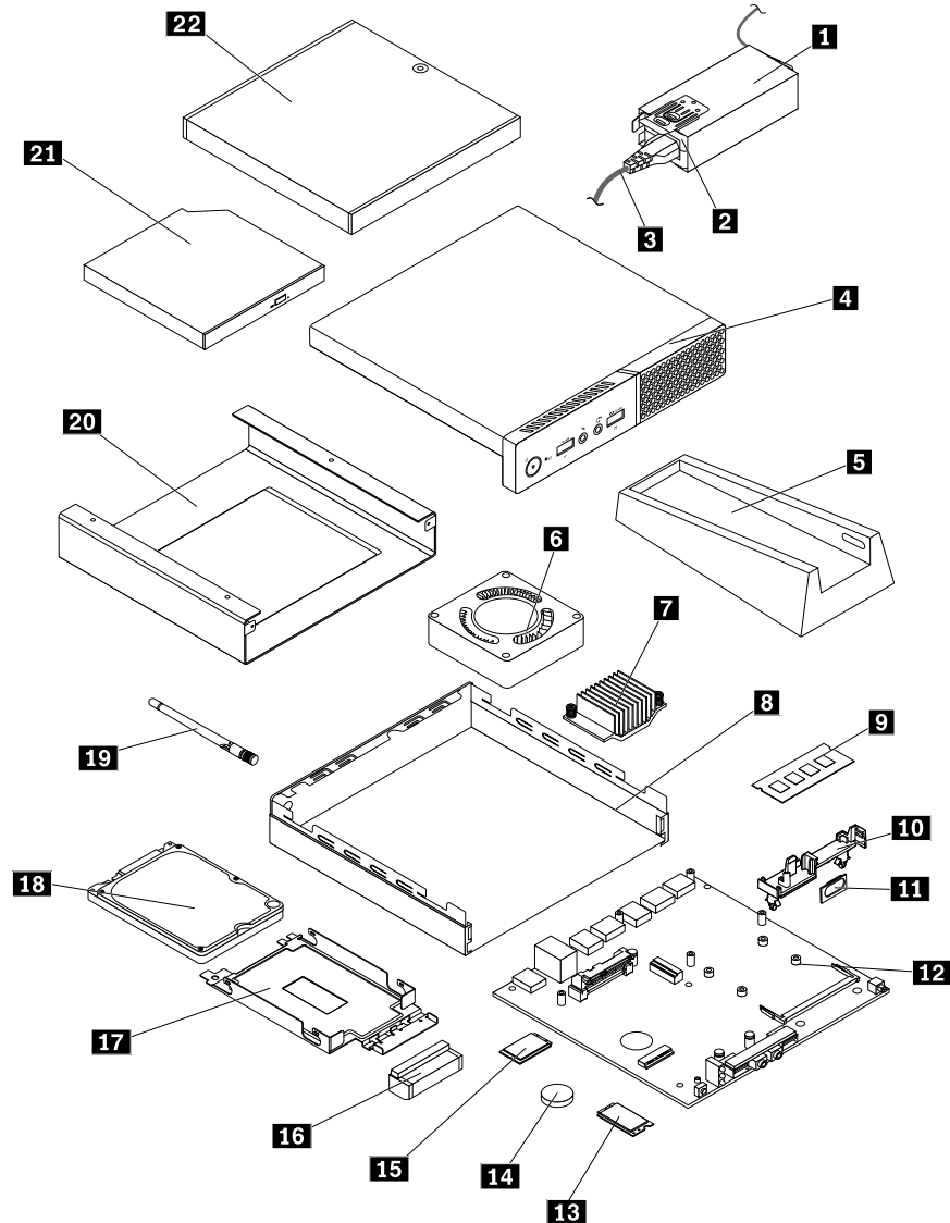
Figure 5. Major FRUs and CRUs
