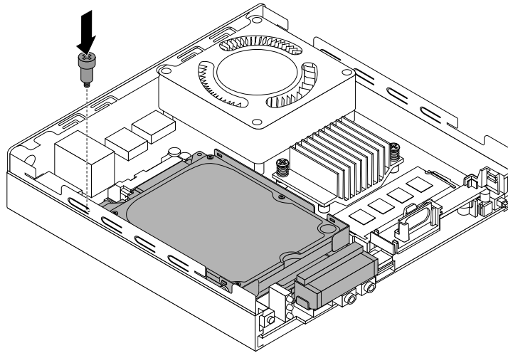
Figure 58. Installing the storage drive bracket screw
