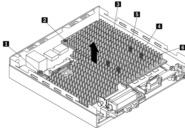
Figure 45. Removing the heat sink
