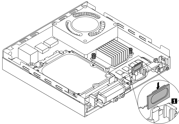
Figure 50. Installing the internal speaker (for 10G8, 10G9, 10GA, 10GB, 10GC, 10GD, 10GE, and 10GF)
