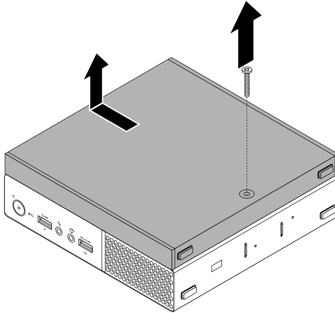
Figure 20. Removing the external optical drive box
