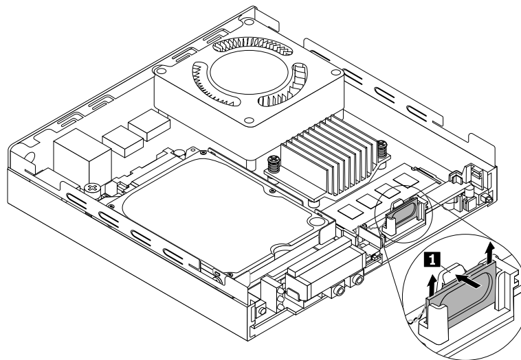
Figure 48. Removing the internal speaker (for 10G8, 10G9, 10GA, 10GB, 10GC, 10GD, 10GE, and 10GF)
