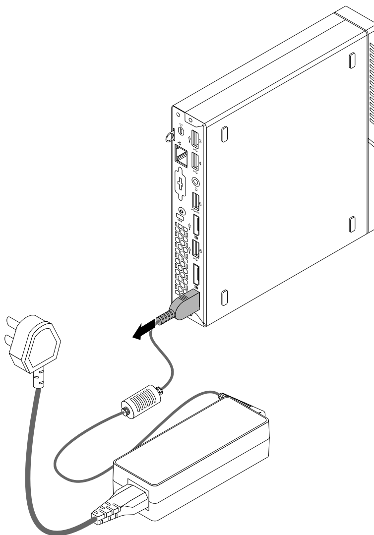
Figure 12. Removing the power adapter
