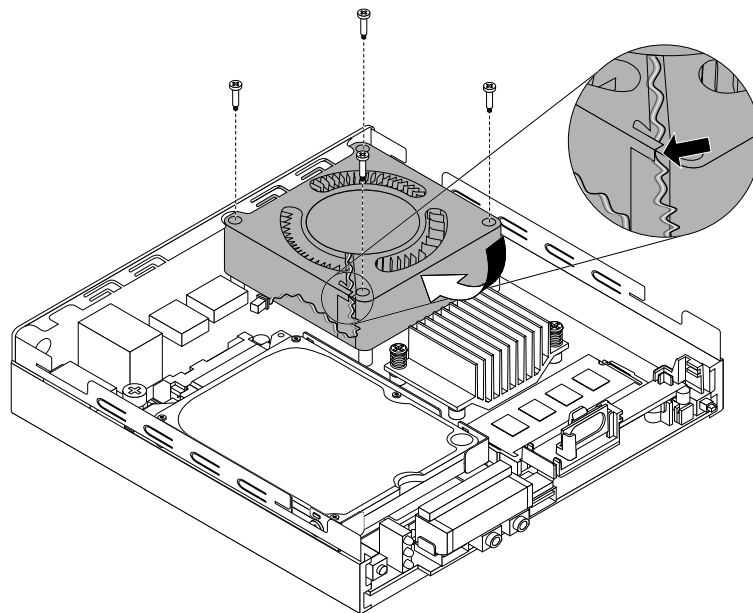
Figure 43. Installing the system fan
