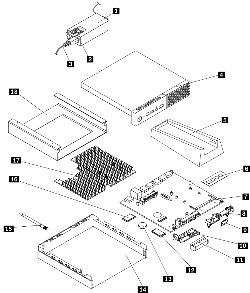
Figure 6. Major FRUs and CRUs
