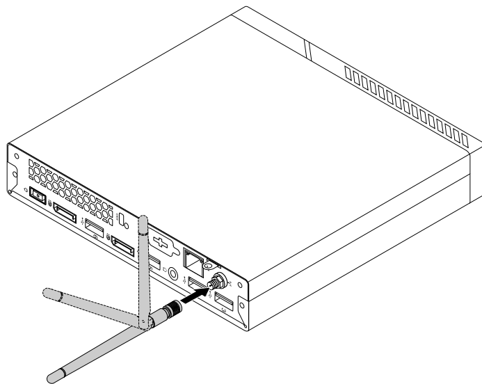
Figure 77. Installing the rear Wi-Fi antenna
