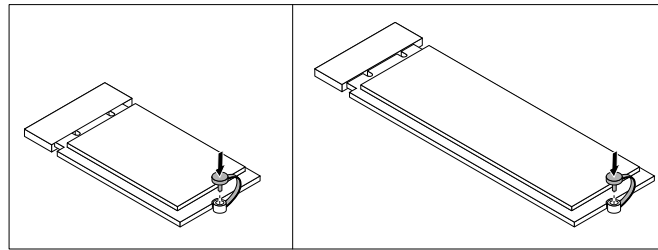
Figure 62. Installing the M.2 storage drive screw
