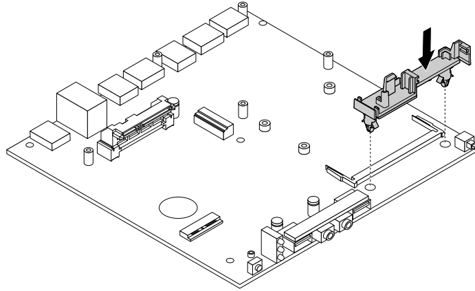
Figure 85. Installing the internal speaker holder
