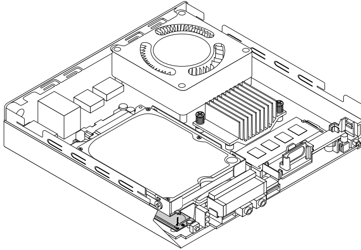
Figure 74. Installing the front Wi-Fi antenna cable (for 10G8, 10G9, 10GA, 10GB, 10GC, 10GD, 10GE, and 10GF)
