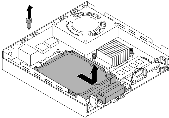
Figure 54. Removing the storage drive bracket
