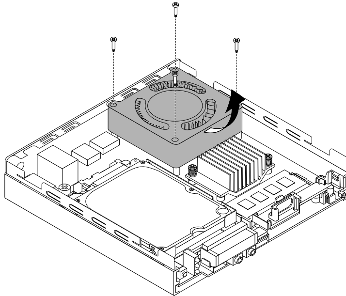
Figure 42. Removing the system fan
