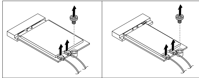
Figure 65. Removing the Wi-Fi card cables
