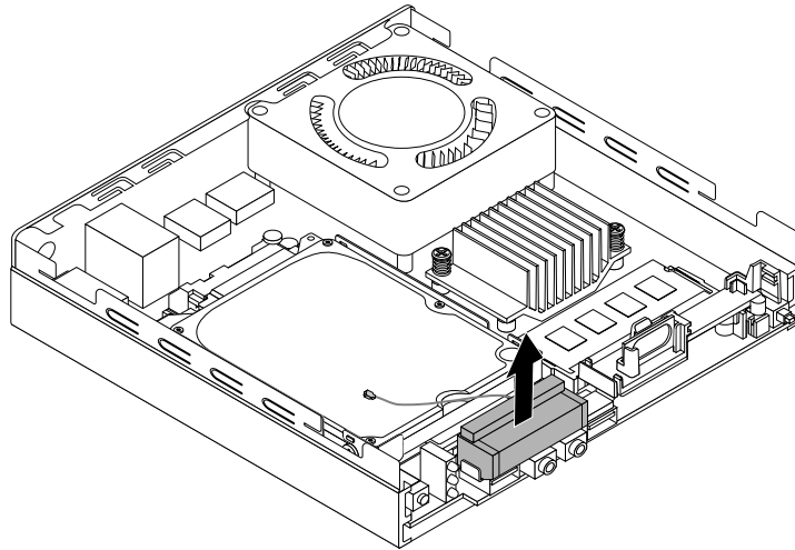
Figure 69. Removing the front Wi-Fi antenna (for 10G8, 10G9, 10GA, 10GB, 10GC, 10GD, 10GE, and 10GF)
