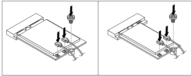
Figure 68. Connecting the Wi-Fi antenna cables
