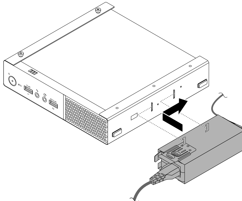
Figure 37. Installing the power adapter bracket
