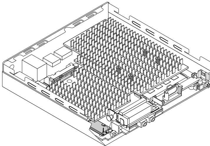
Figure 75. Installing the front Wi-Fi antenna cable (for 10KG, 10KH, 10KJ, and 10KK)
