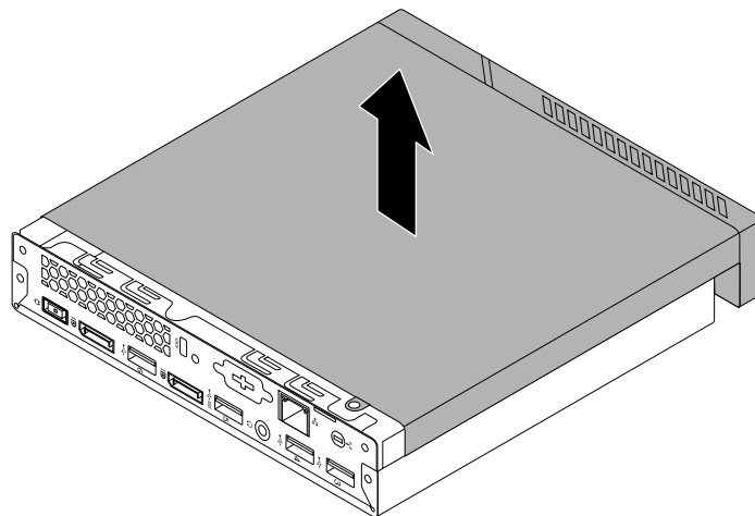
Figure 41. Removing the computer cover
