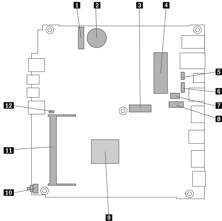
Figure 7. Parts on the system board
