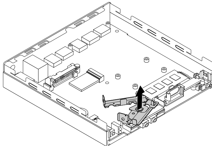
Figure 80. Removing the antenna bracket
