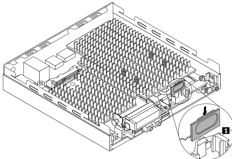
Figure 51. Installing the internal speaker (for 10KG, 10KH, 10KJ, and 10KK)
