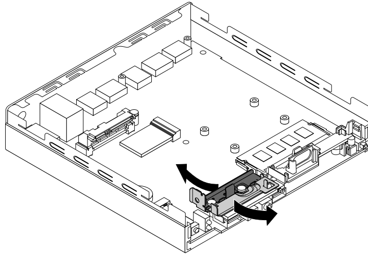
Figure 79. Opening and pivoting the antenna bracket
