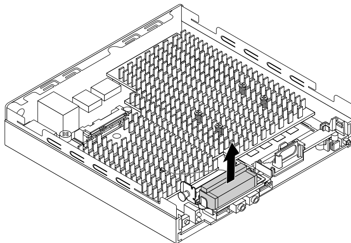
Figure 70. Removing the front Wi-Fi antenna (for 10KG, 10KH, 10KJ, and 10KK)
