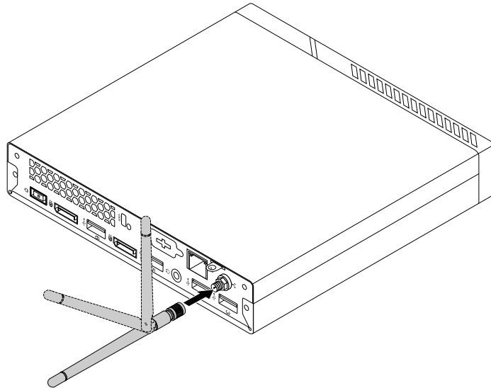
Figure 76. Removing the rear Wi-Fi antenna
