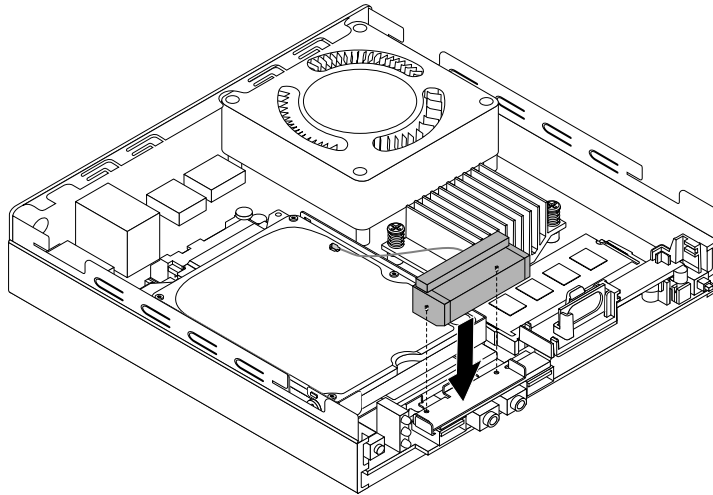
Figure 72. Sticking the front Wi-Fi antenna (for 10G8, 10G9, 10GA, 10GB, 10GC, 10GD, 10GE, and 10GF)
