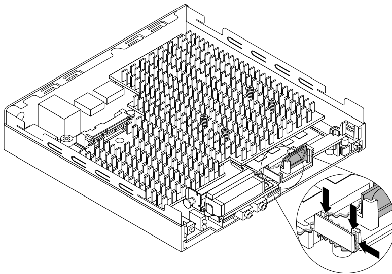
Figure 53. Securing the internal speaker cable (for 10KG, 10KH, 10KJ, and 10KK)
