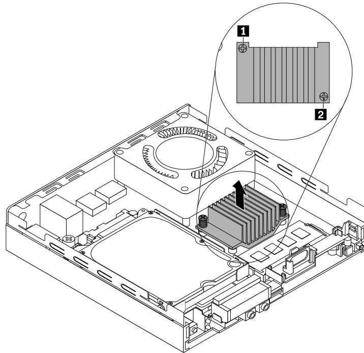
Figure 44. Removing the heat sink
