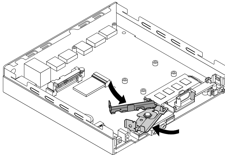
Figure 82. Pivoting and closing the antenna bracket
