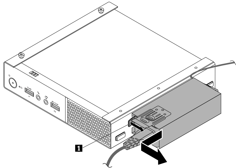
Figure 36. Removing the power adapter bracket
