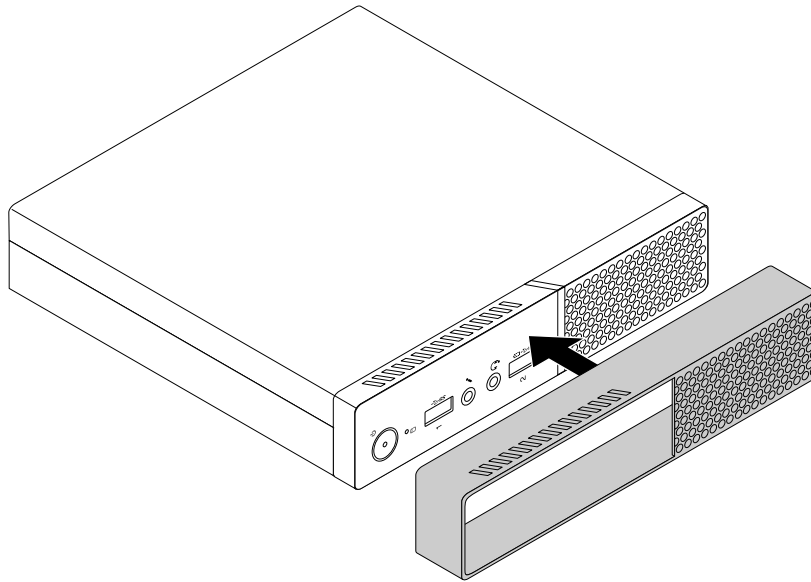
Figure 87. Installing the dust shield
