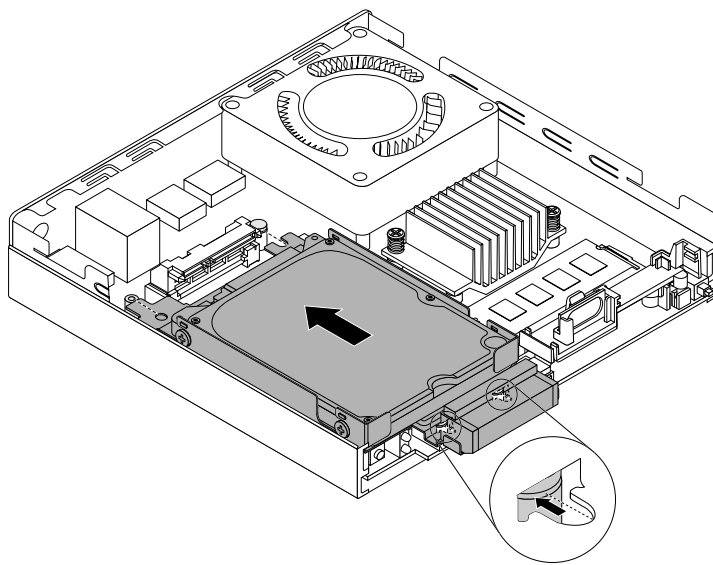
Figure 57. Installing the storage drive bracket
