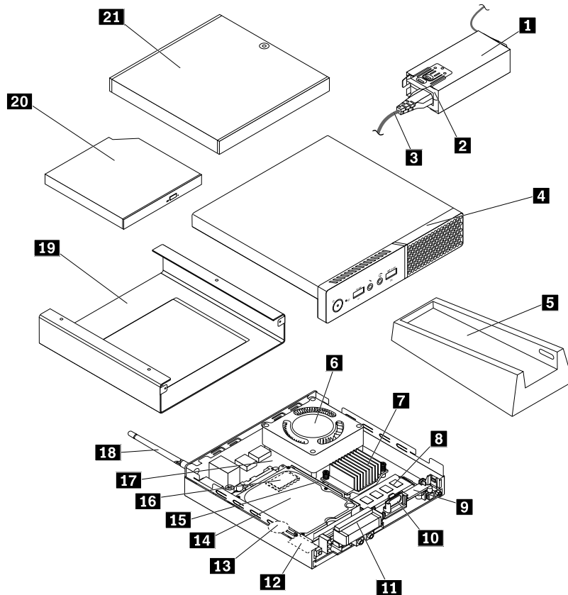
Figure 3. Computer components
