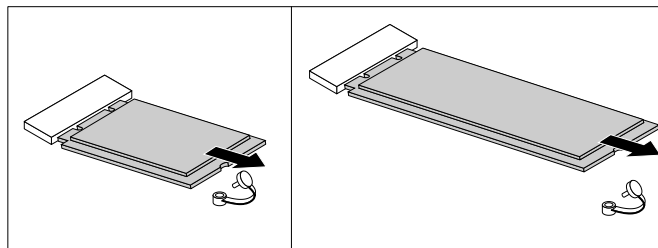
Figure 60. Removing the M.2 storage drive
