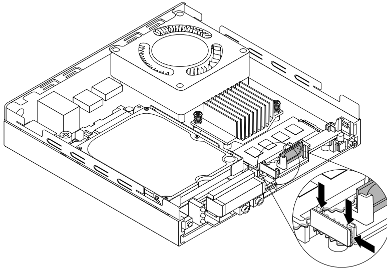
Figure 52. Securing the internal speaker cable (for 10G8, 10G9, 10GA, 10GB, 10GC, 10GD, 10GE, and 10GF)
