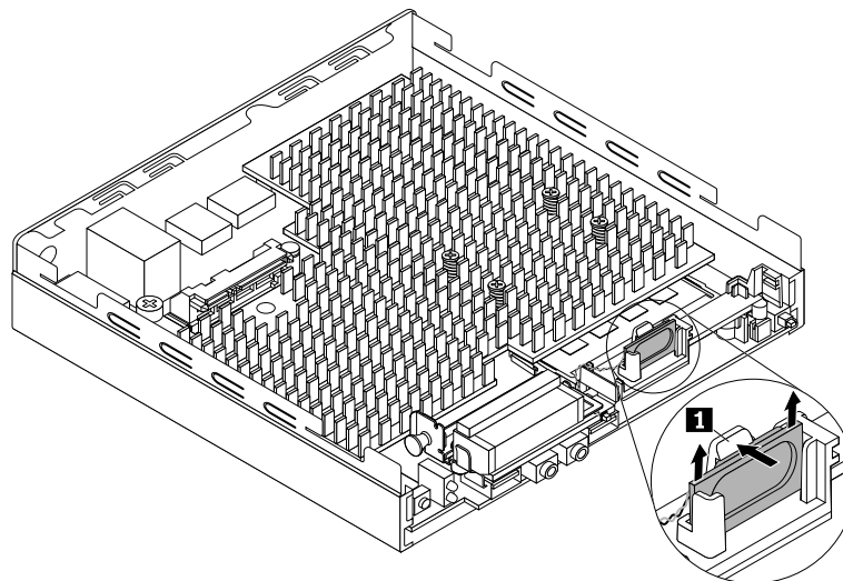
Figure 49. Removing the internal speaker (for 10KG, 10KH, 10KJ, and 10KK)
