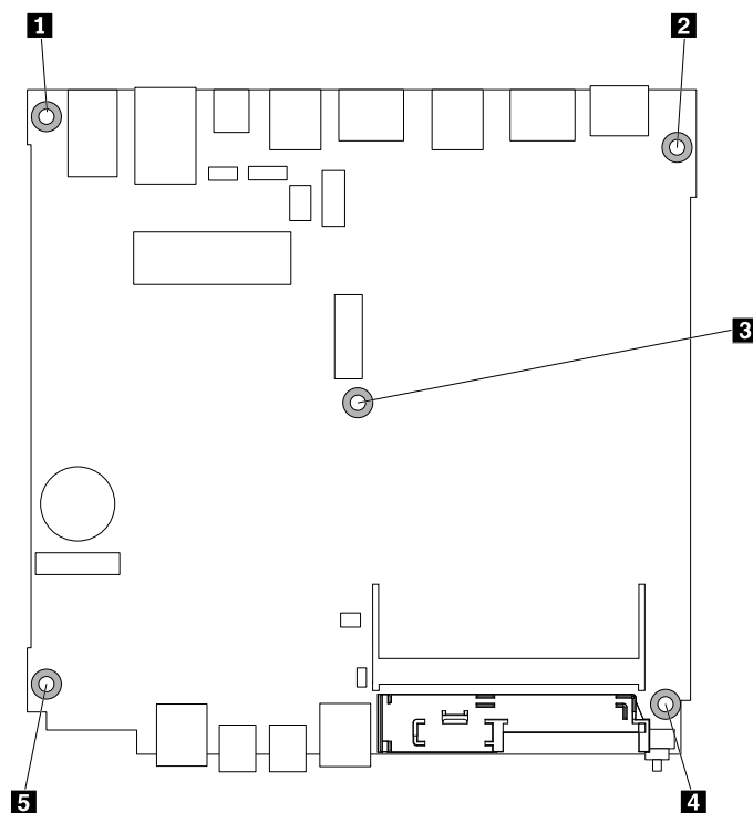
Figure 83. Removing the five screws that secure the system board
