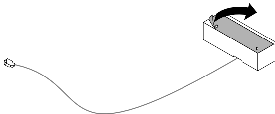
Figure 71. Peeling off the paper that protects the sticker
