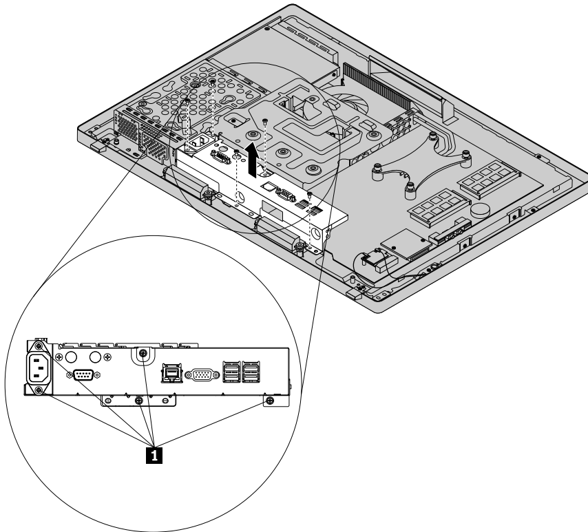
Figure 22. Removing the power cord connector
