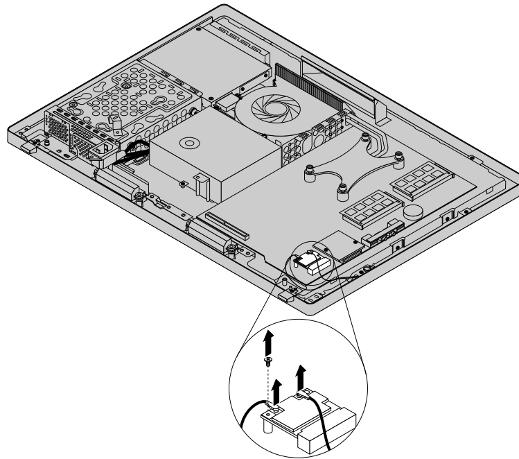
Figure 48. Removing the screw that secures the Wi-Fi card to the system board
