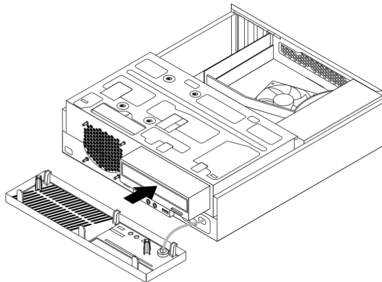
Figure 30. Installing a new optical drive
