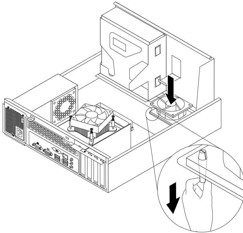
Figure 38. Installing the front fan assembly
