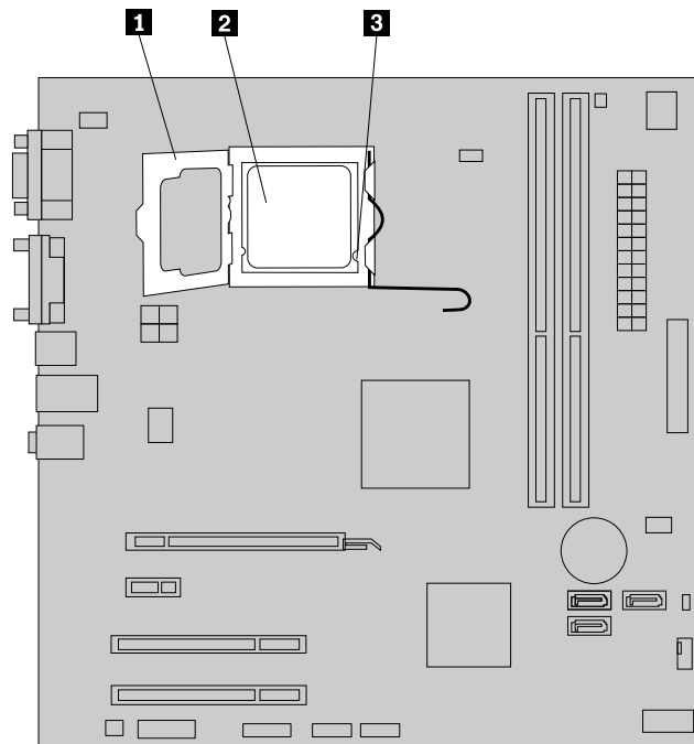
Figure 21. Accessing the microprocessor
