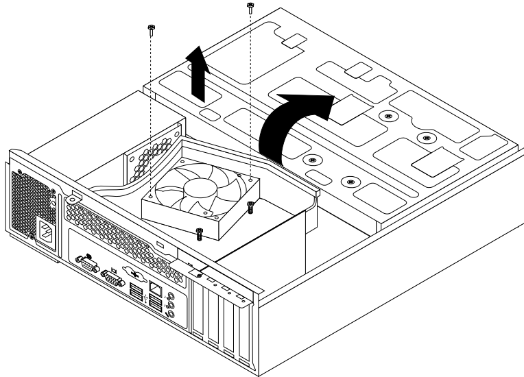
Figure 23. Removing the heat sink fan duct
