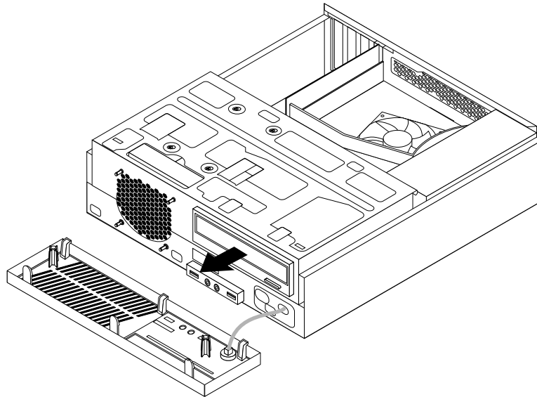
Figure 29. Removing the optical drive
