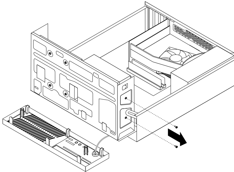
Figure 27. Removing the optical drive screws
