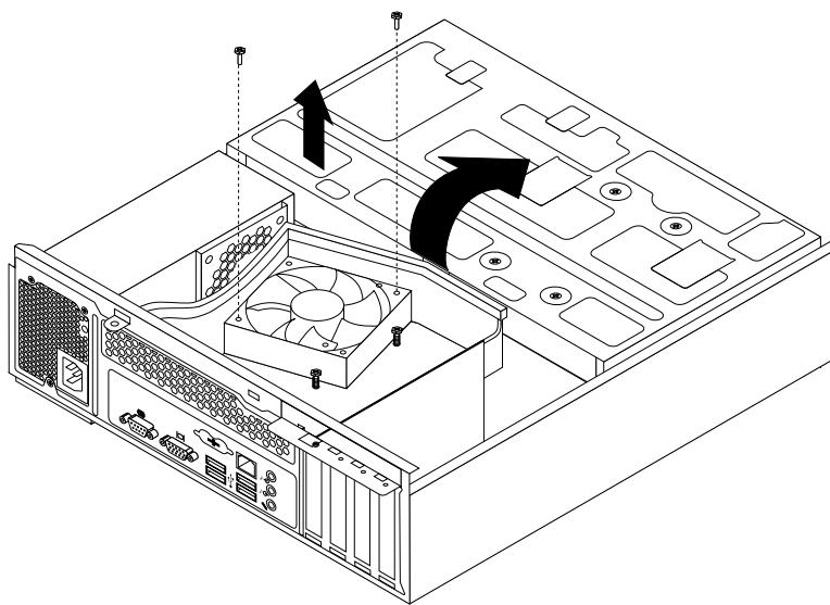
Figure 18. Removing the heat sink fan duct
