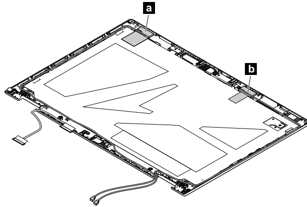
b Wireless-LAN main antenna (gray)
