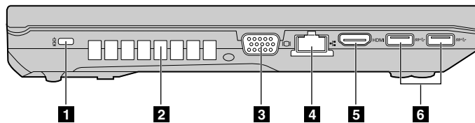
Figure 4. Lenovo ZhaoYang K49 left-side view
