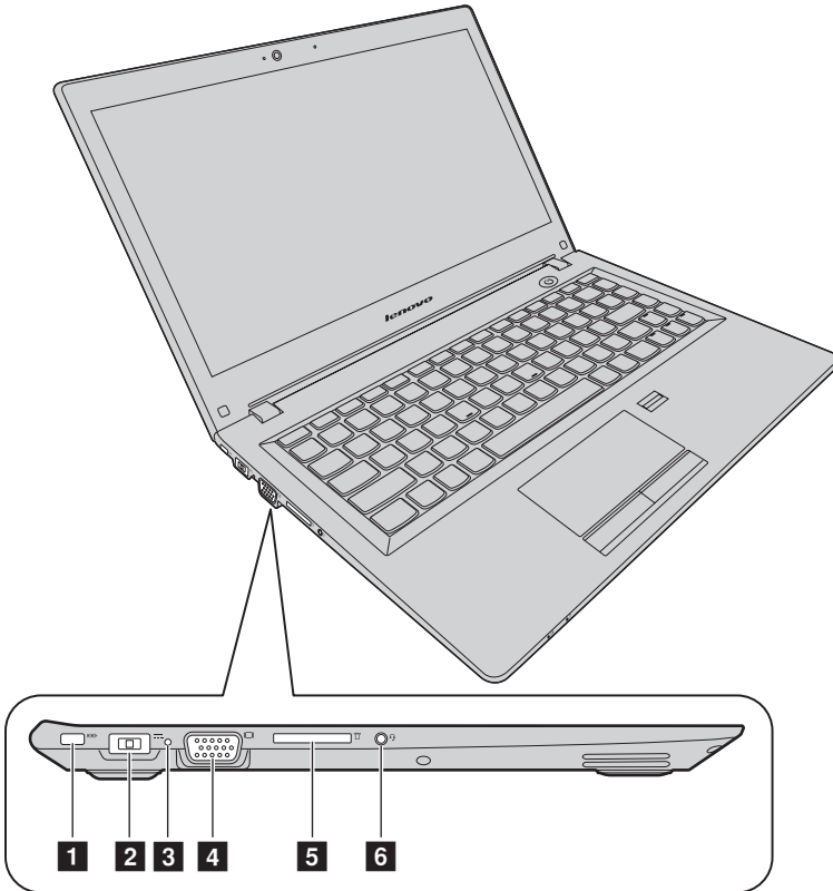
Figure 2. Left-side view
