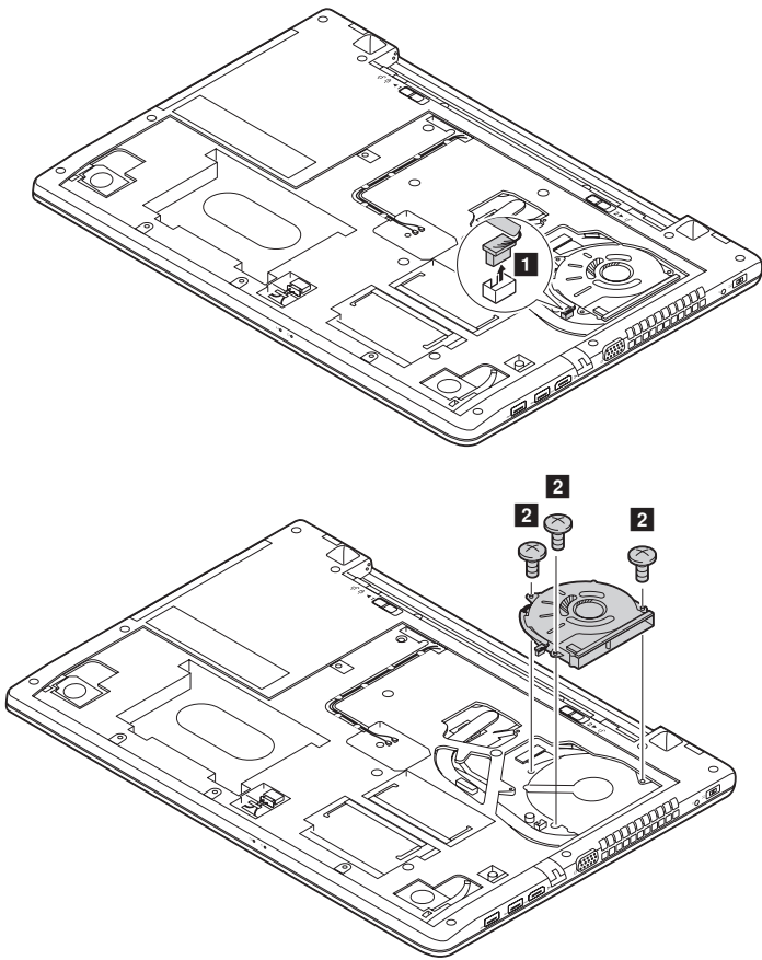
Figure 8. Removal steps of fan assembly
