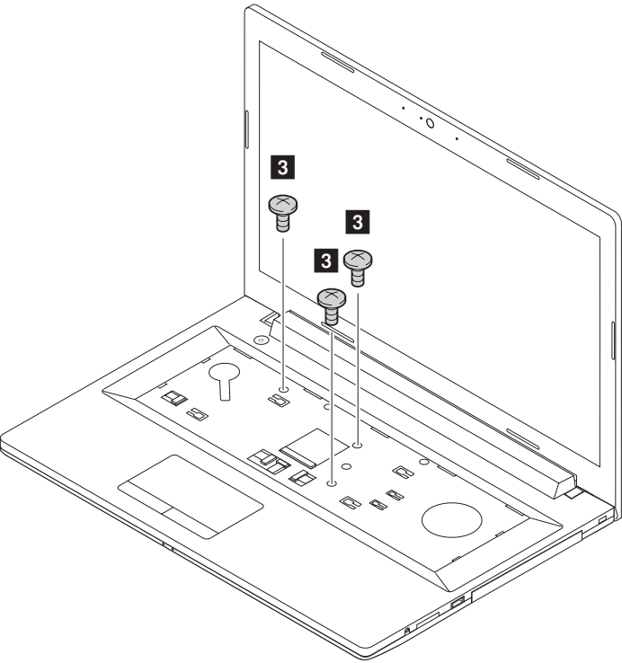
Figure 10. Removal steps of keyboard bezel (continued)
