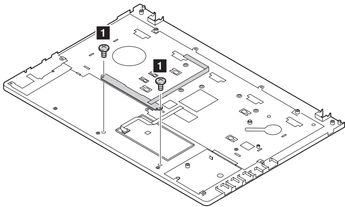
Figure 14. Removal steps of base cover and LED board (continued)
