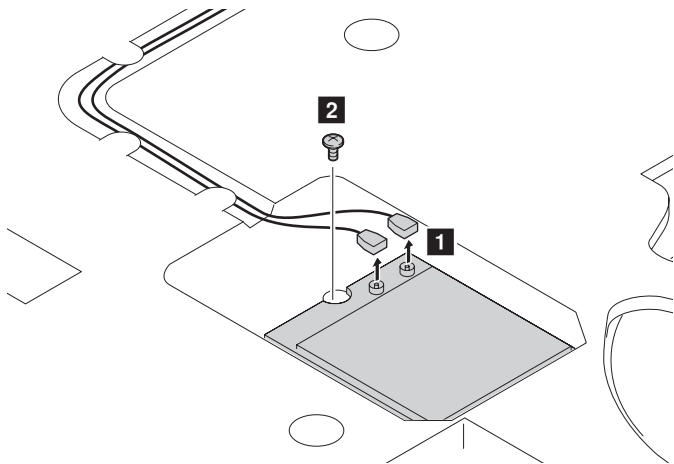
Figure 6. Removal steps of PCI Express Mini Card for wireless LAN/WAN Disconnect the two wireless LAN cables (black, white) 1 , and then remove the screw 2 .
