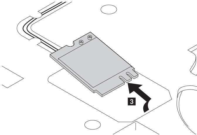
Figure 6. Removal steps of PCI Express Mini Card for wireless LAN/WAN (continued)
