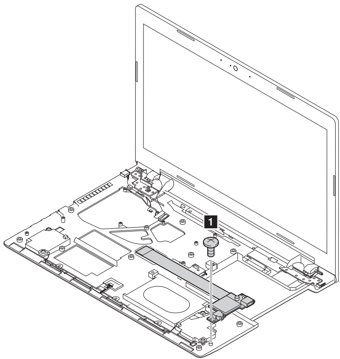
Figure 14. Removal steps of base cover and LED board Loosen the screw 1 , then remove the USB and audio board.
