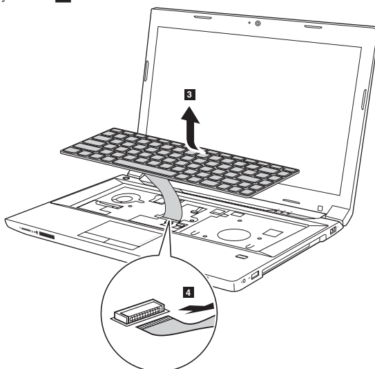
Figure 8. Removal steps of keyboard (continued)
