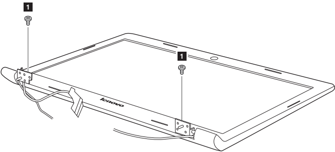
Figure 15. Removal steps of LCD front bezel
