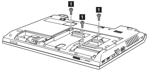
Figure 8. Removal steps of keyboard Remove screws 1 .
