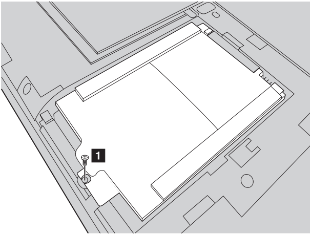
Figure 4. Removal steps of hard disk drive
