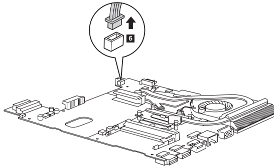
Figure 10. Removal steps of system board (continued)
