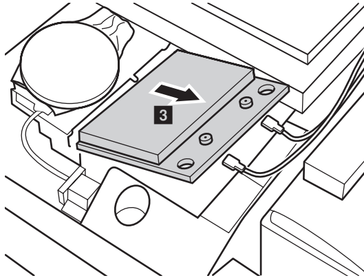
Figure 7. Removal steps of Mini PCI Express Card for wireless LAN/WAN (continued)
