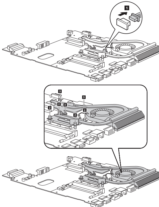
Figure 12. Removal steps of fan assembly and heat sink assembly
