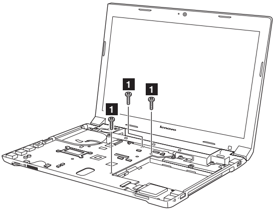
Figure 10. Removal steps of system board
