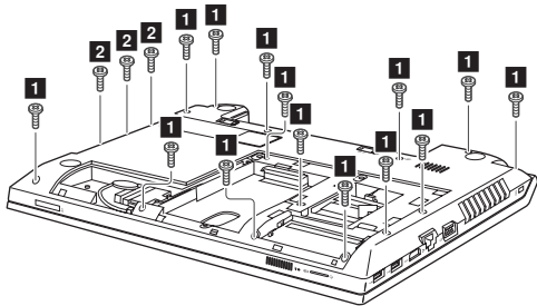
Figure 9. Removal steps of keyboard bezel
