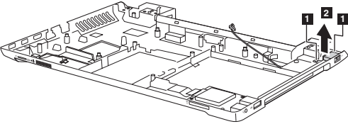
Figure 14. Removal steps of base cover, power assembly and IO board (continued) Remove two screws 1 . Remove the power assembly in the direction shown by arrow 2 .
