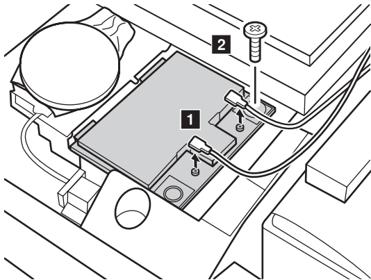
Figure 7. Removal steps of Mini PCI Express Card for wireless LAN/WAN Disconnect the two wireless LAN cables (black, white) 1 , and then remove the screw 2 .
