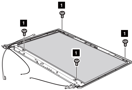
Figure 16. Removal steps of LCD panel
