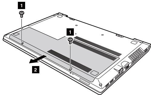
Figure 3. Removal steps of bottom slot cover
