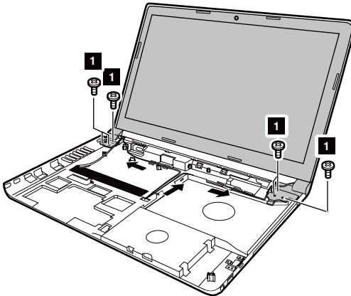
Figure 14. Removal steps of LCD unit and base cover
