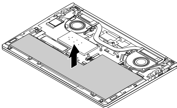
Figure 7. Take out the battery pack
