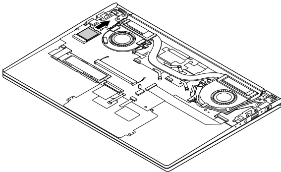
Figure 14. Remove the wireless module
