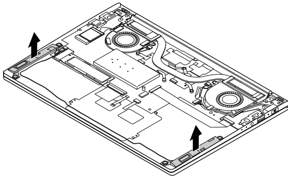
Figure 16. Remove speakers
