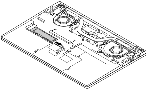
Figure 11. Remove by pulling the solid-state drive
