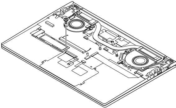
Figure 10. Remove 1 screw
