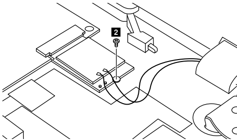
Figure 13. Remove 1 screw
