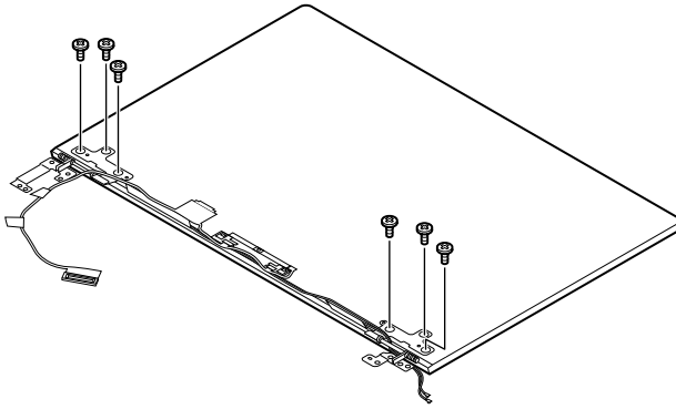
Figure 33. Remove 6 screws
