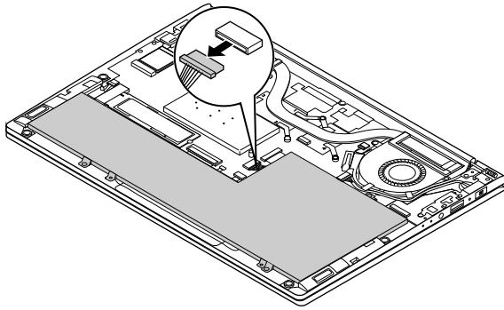
Figure 5. Disconnect the cable
