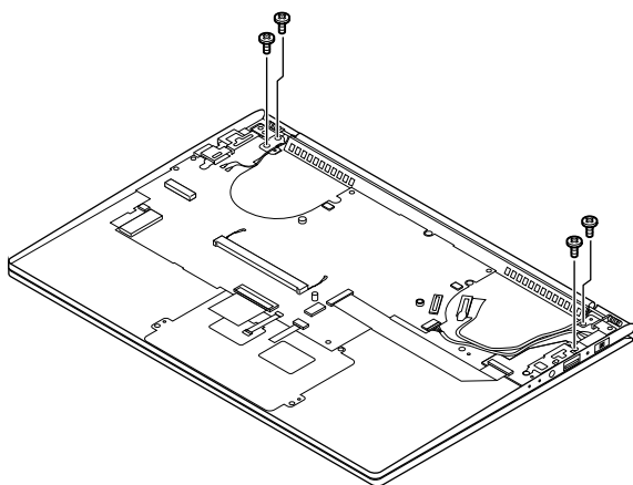
Figure 18. Remove 4 screws
