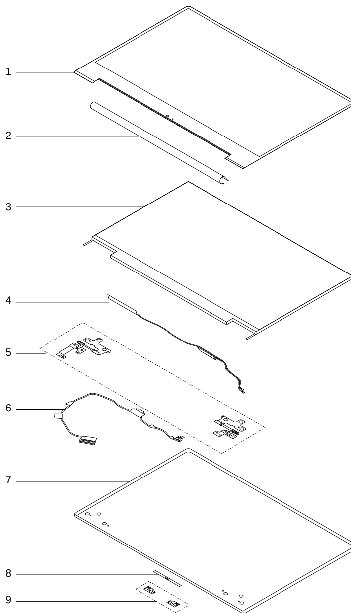
Figure 2. LCD module — exploded view
