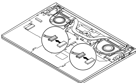
Figure 19. Disconnect two plugs
