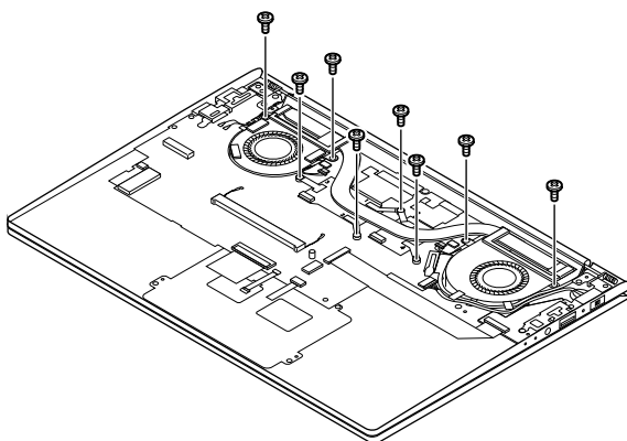
Figure 20. Remove screws
