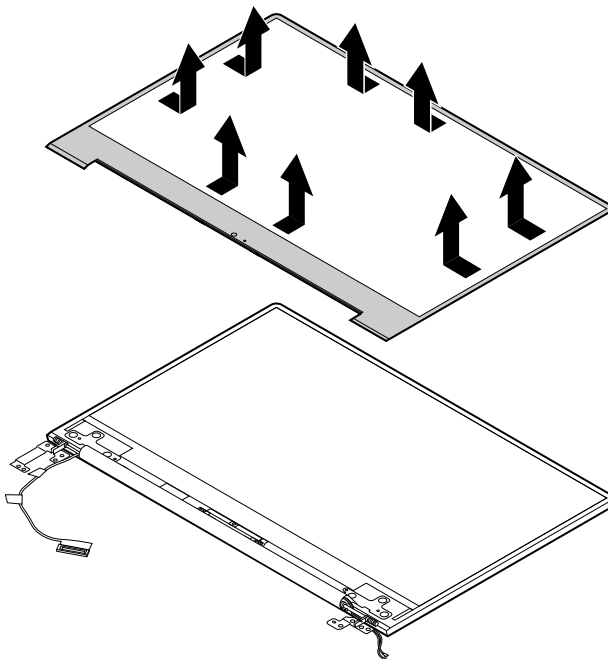
Figure 29. Pull the inner sides of the LCD bezel
