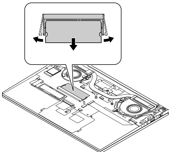
Figure 9. Remove the RAM module
