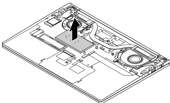
Figure 8. Remove EMI shield
