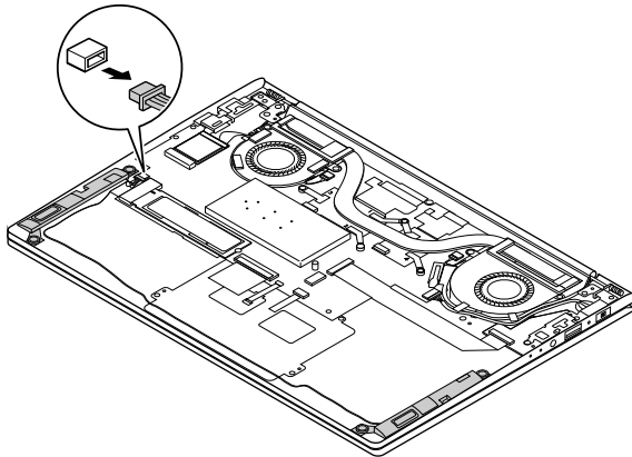
Figure 15. Disconnect the cable
