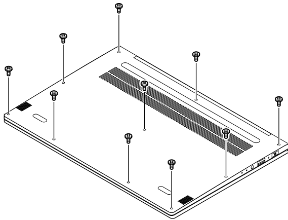
Figure 3. Remove 10 screws
