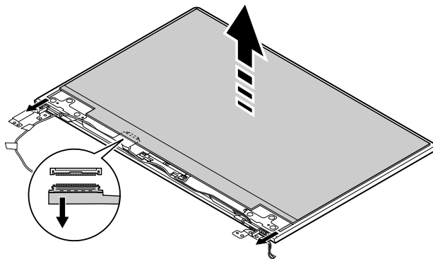
Figure 32. Remove 4 screws and lift up the LCD panel
