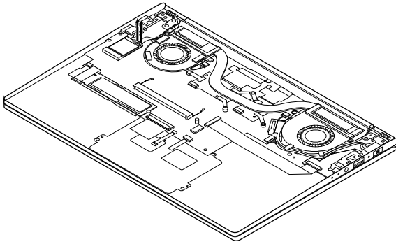
Figure 12. Disconnect antenna cables
