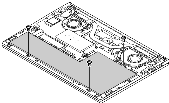
Figure 6. Remove screws and take out the battery pack
