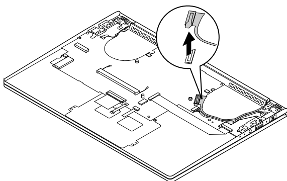
Figure 17. Disconnect the LCD cable
