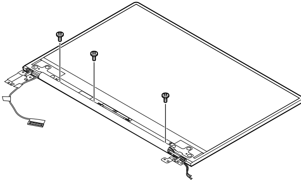
Figure 30. Pull the inner sides of the LCD bezel
