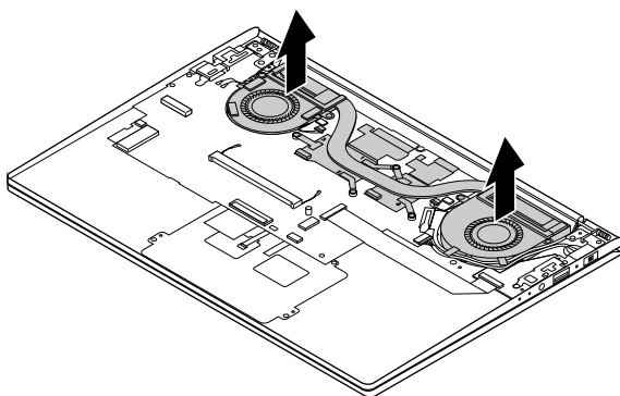
Figure 21. Remove the heat sink
