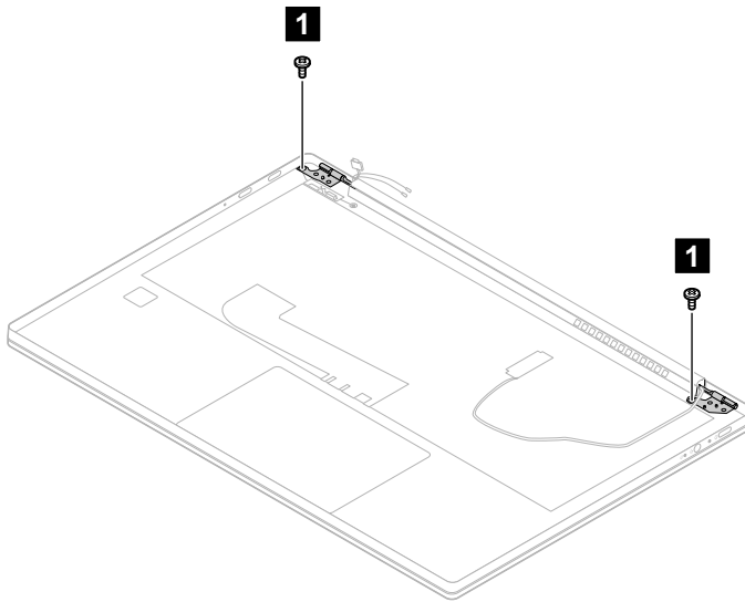
Figure 29. Remove the 2 screws
