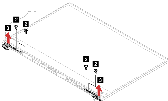
Figure 33. Remove the 4 screws and hinges
