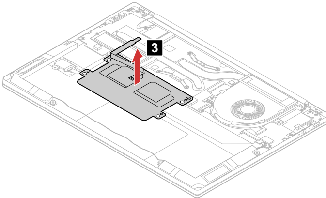
Figure 22. Remove the touchpad
