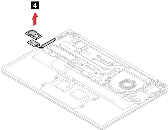
Figure 19. Remove the fingerprint board and bracket
