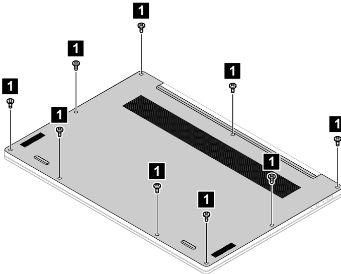
Figure 1. Remove the 9 screws
