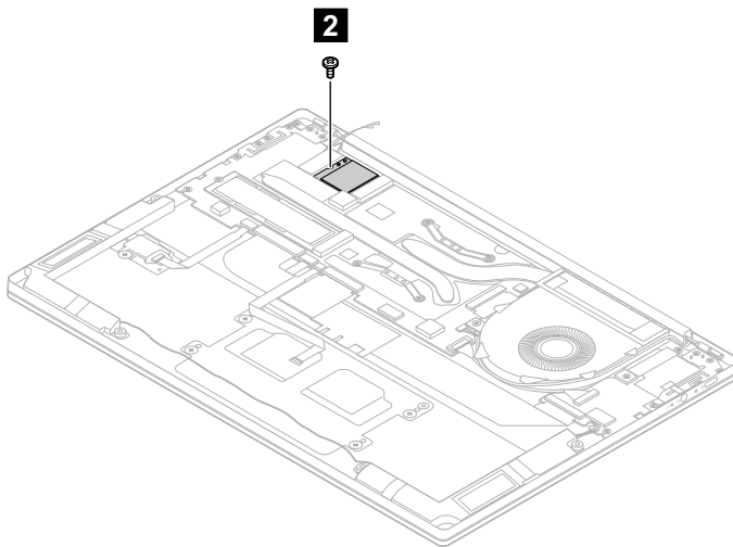
Figure 8. Remove 1 screw
