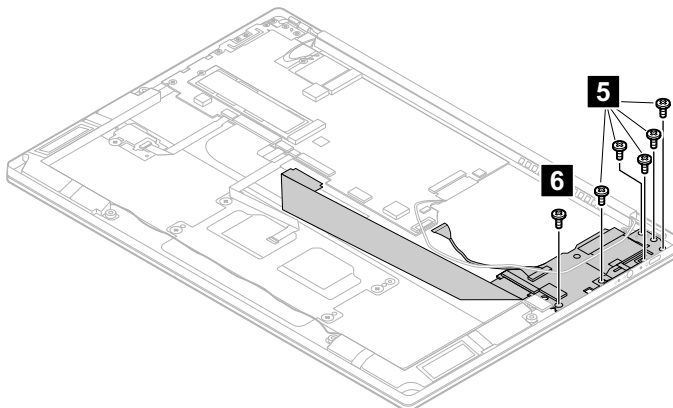
Figure 24. Remove the screws
