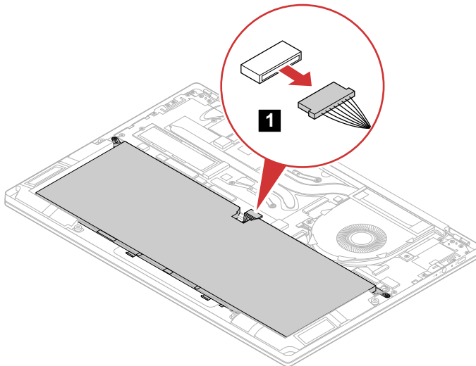
Figure 4. Detach the battery pack connector
