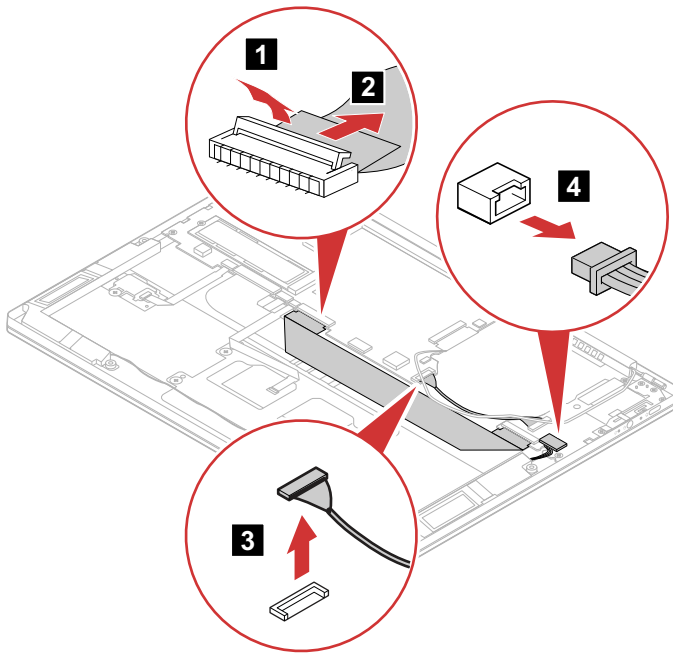
Figure 23. Detach the connectors
