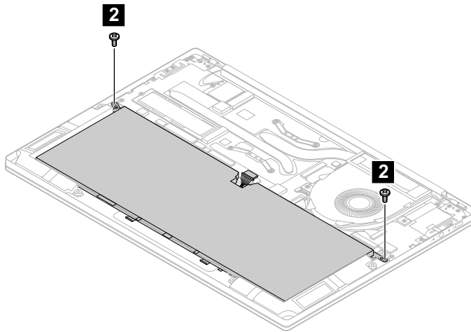
Figure 5. Remove the 2 screws
