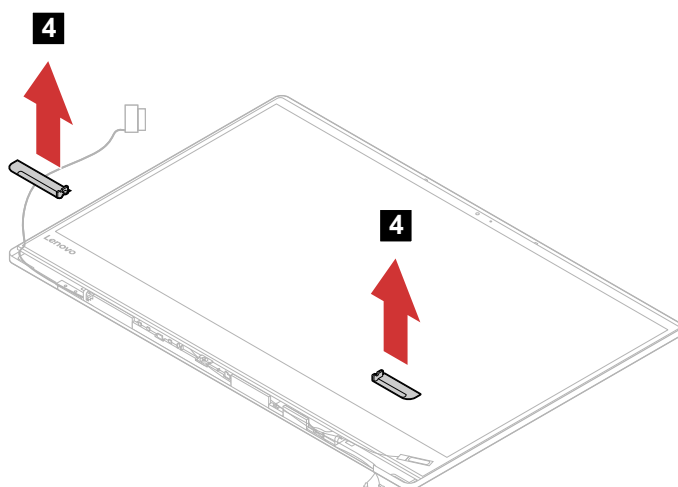
Figure 34. Remove the hinge covers
