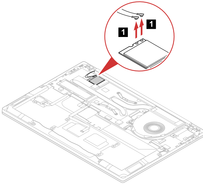
Figure 7. Detach the connectors
