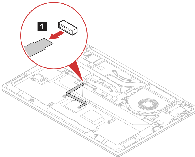
Figure 20. Detach the touchpad connector
