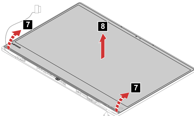
Figure 37. Remove the LCD panel
