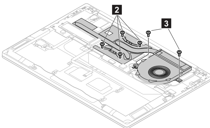
Figure 11. Loosen and remove the screws
