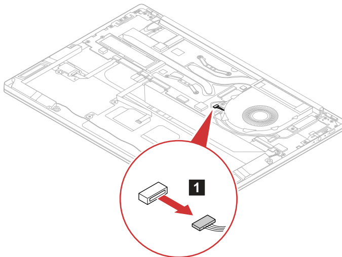
Figure 10. Detach the fan connector
