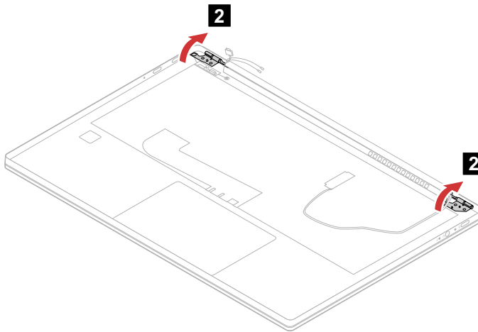
Figure 30. Open the hinges
