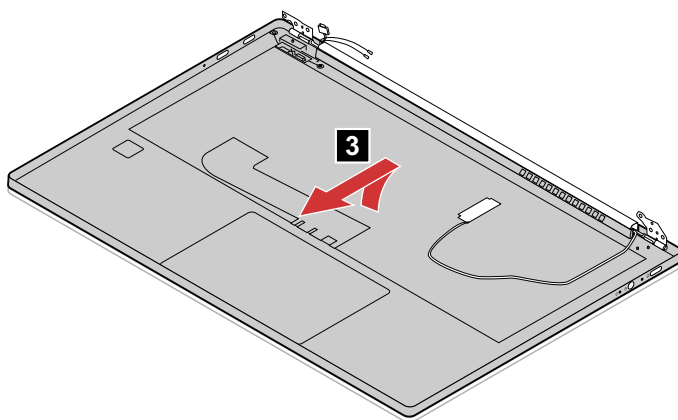
Figure 31. Remove the upper case
