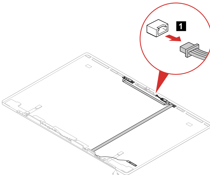
Figure 39. Detach the camera cable connector
