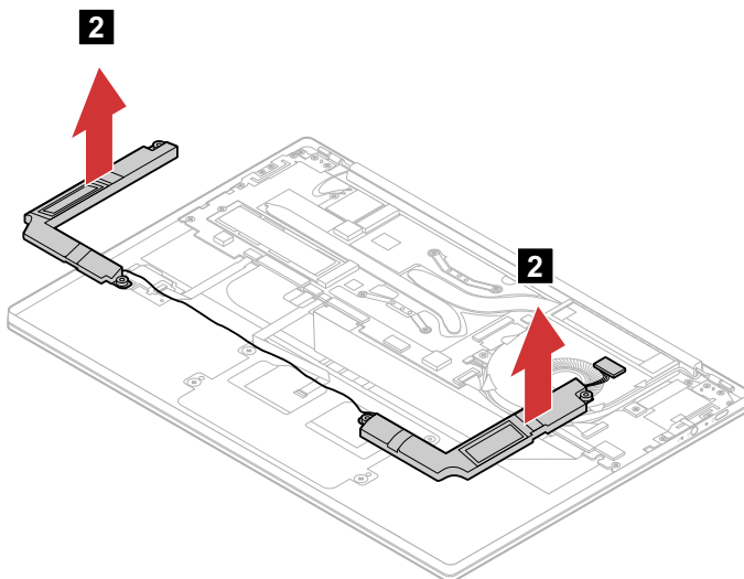
Figure 16. Remove the speakers
