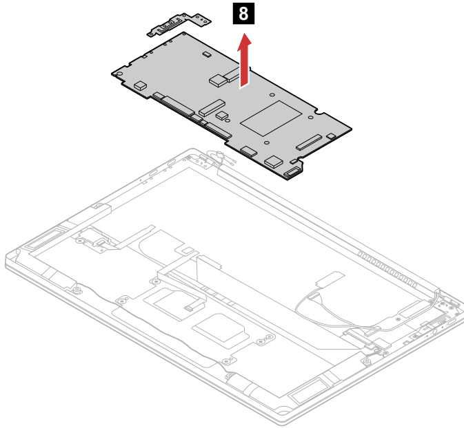
Figure 28. Remove the system board and bracket
