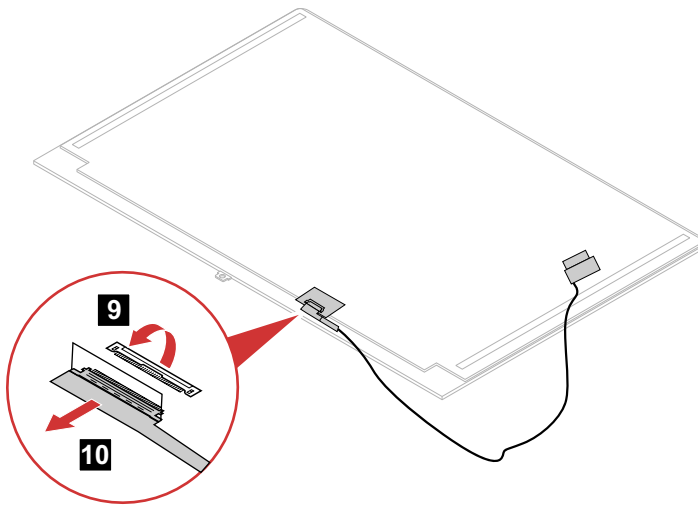
Figure 38. Remove the EDP cable
