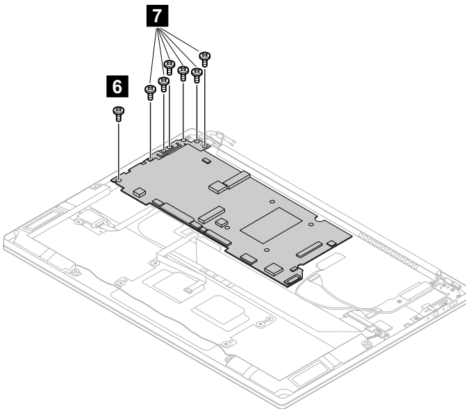
Figure 27. Remove the 7 screws
