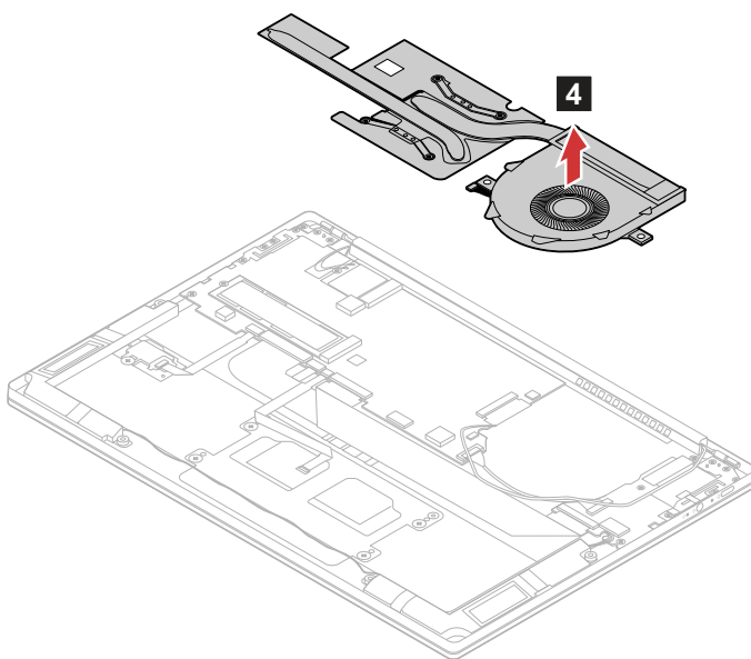
Figure 12. Remove the heat sink and fan assembly
