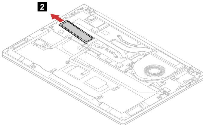
Figure 14. Remove the M.2 solid-state drive
