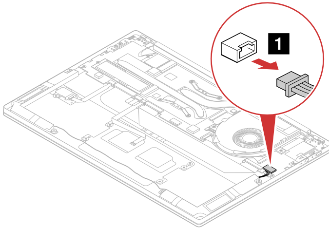
Figure 15. Detach the speaker connector
