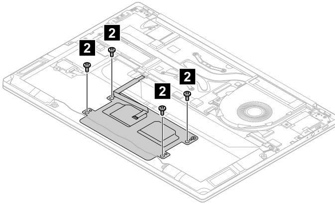
Figure 21. Remove the 4 screws
