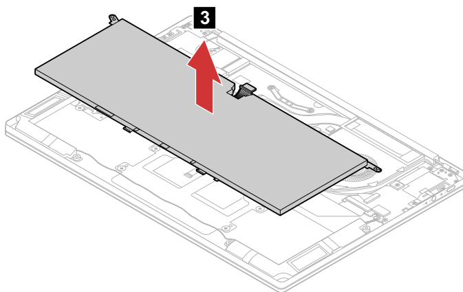
Figure 6. Remove the battery pack
