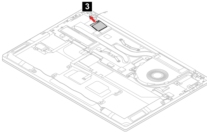
Figure 9. Remove the Wi-Fi card
