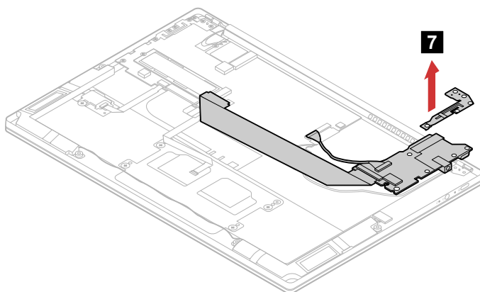
Figure 25. Remove the USB board and bracket
