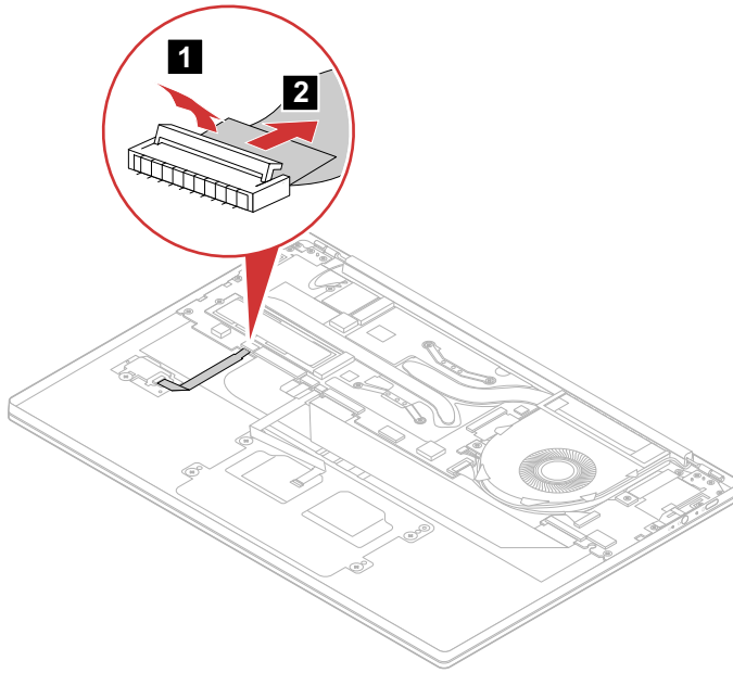
Figure 17. Detach the fingerprint cable connector
