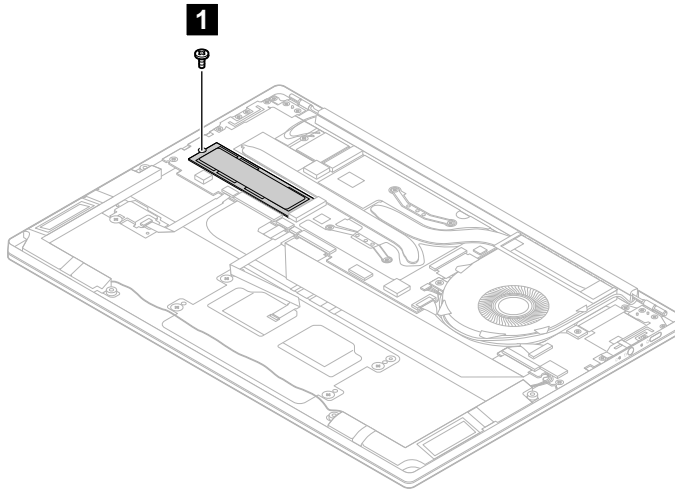
Figure 13. Remove 1 screw
