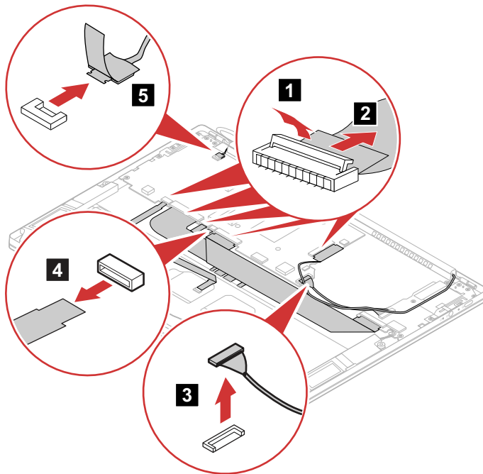
Figure 26. Detach the 8 connectors
