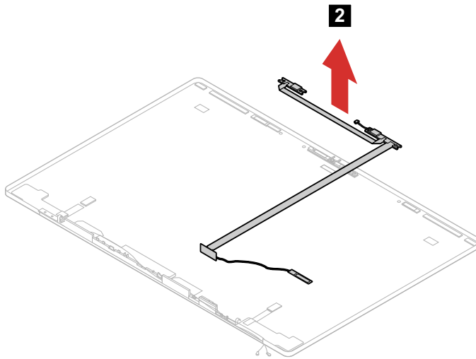
Figure 40. Remove the microphone boards and transform board
