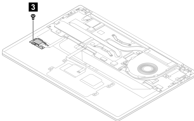
Figure 18. Remove 1 screw
