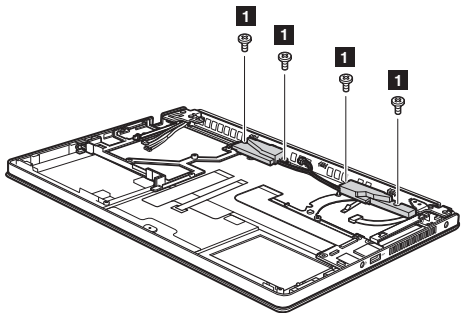
Figure 8. Removal steps of speakers and microphone
