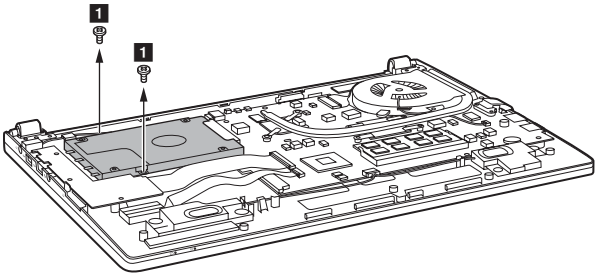
Figure 2. Removal steps of hard disk drive Remove the frame fixing screws 1 .
