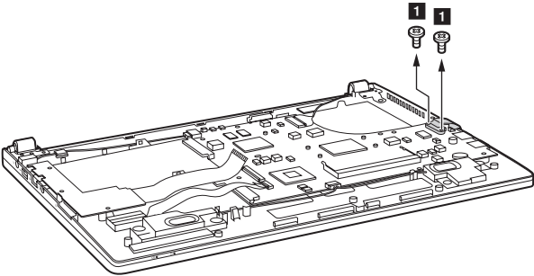
Figure 7. Removal steps of system board (continued)
