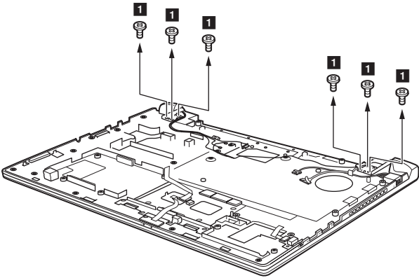
Figure 9. Removal steps of LCD unit Remove six screws 1 .
