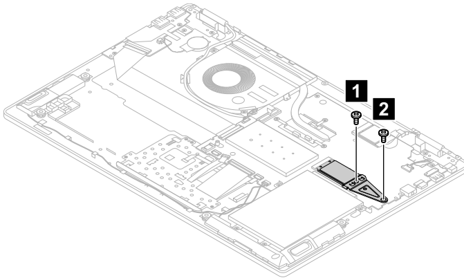
Figure 11. Remove the 2 screws (for 2242)
