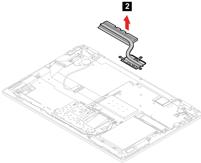
Figure 37. Remove the heat sink
