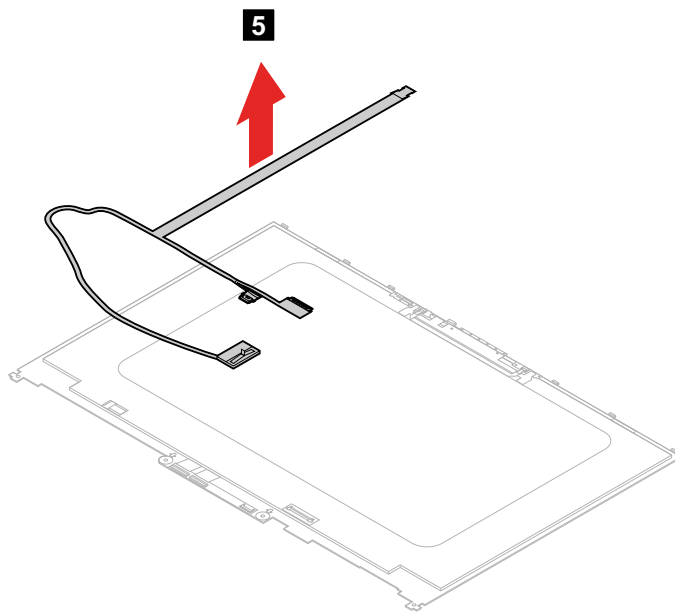
Figure 54. Remove the EDP cable
