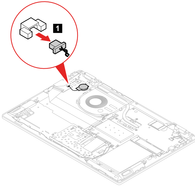
Figure 27. Detach the connector
