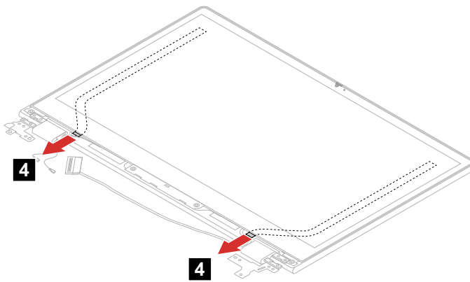
Figure 51. Pull out the removable tapes
