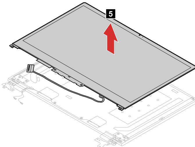
Figure 52. Remove the LCD panel
