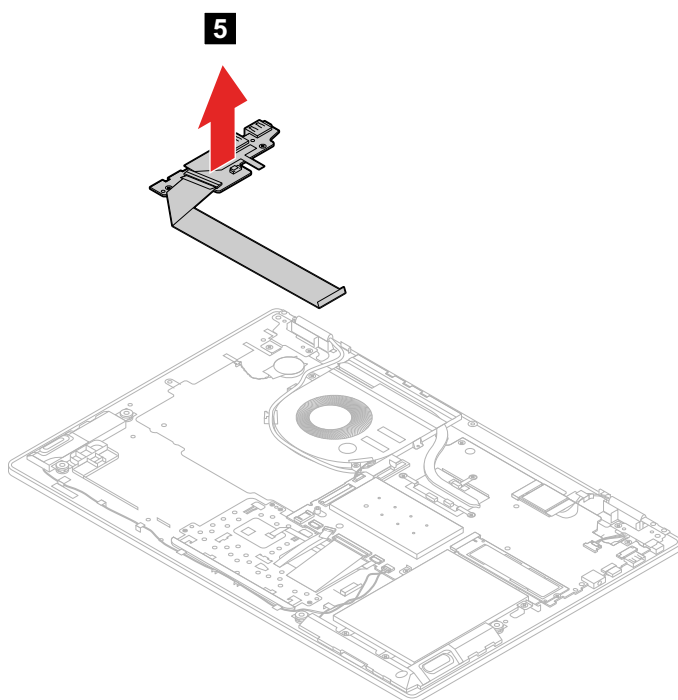
Figure 31. Remove the I/O board
