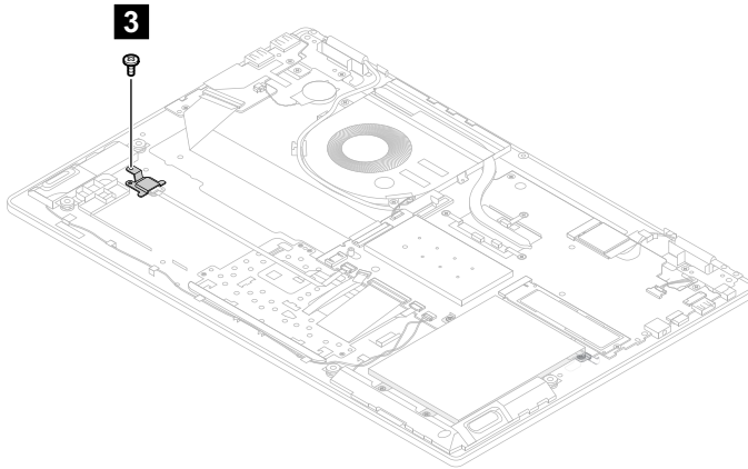
Figure 22. Remove 1 screw
