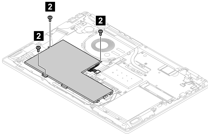
Figure 5. Remove the 3 screws
