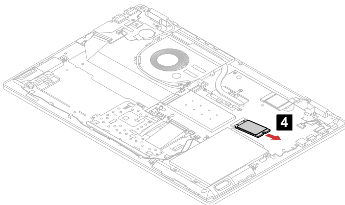
Figure 14. Remove the M.2 solid-state drive
