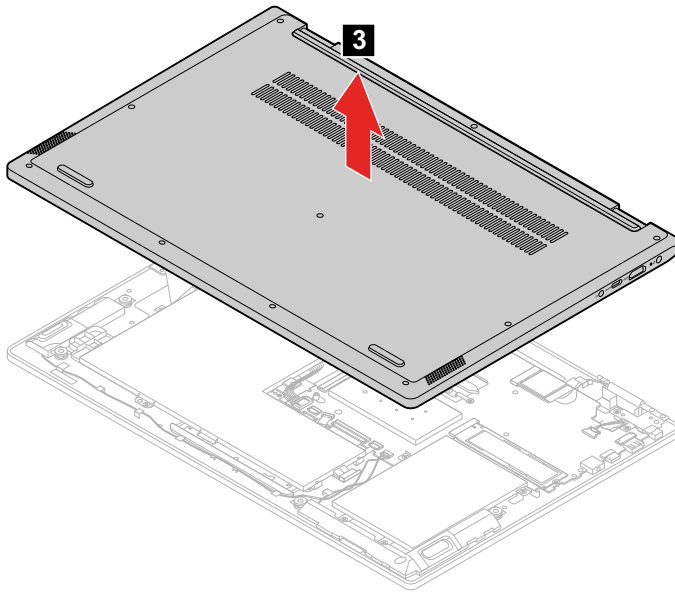
Figure 3. Remove the lower case
