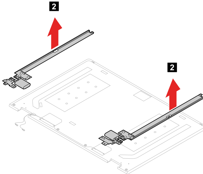
Figure 58. Remove the hinges
