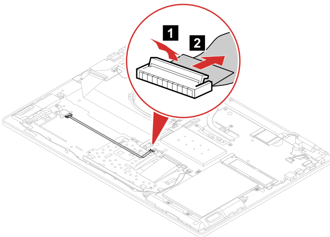
Figure 21. Detach the connector
