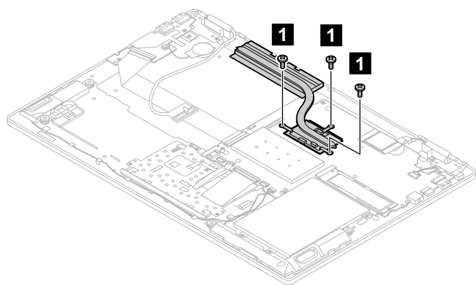
Figure 35. Remove the 3 screws (for UMA)
