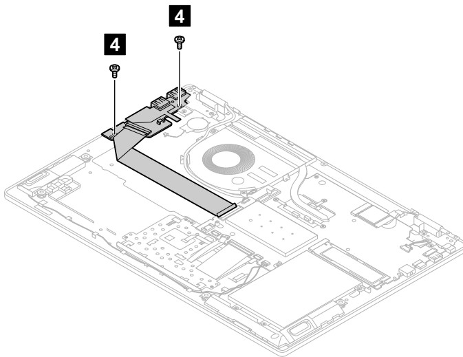
Figure 30. Remove the 2 screws
