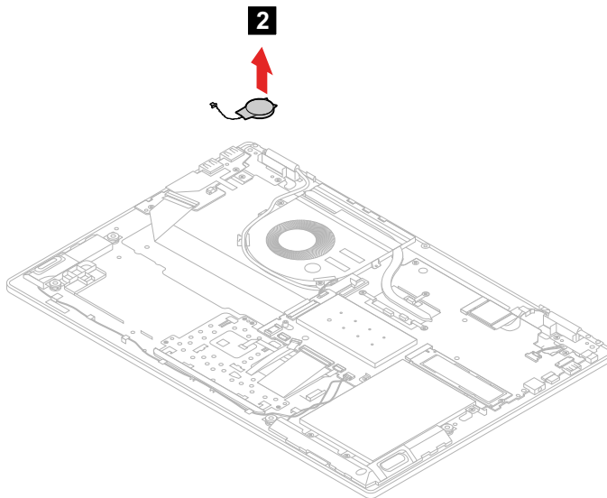
Figure 28. Remove the coin-cell battery
