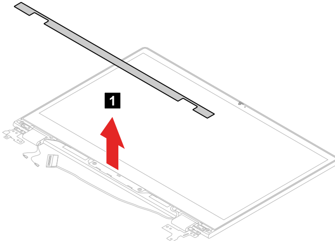
Figure 49. Remove the strip cover
