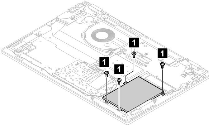
Figure 15. Remove the 4 screws
