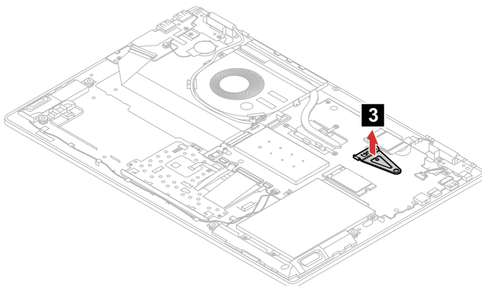
Figure 13. Remove the M.2 solid-state drive bracket
