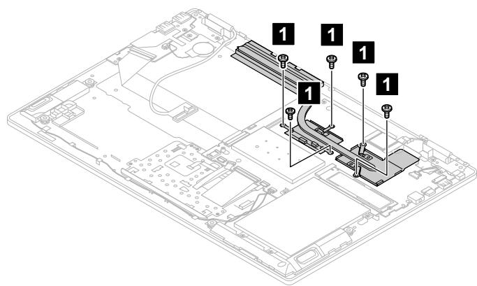
Figure 36. Remove the 5 screws (for DIS)
