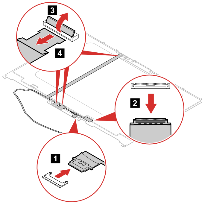
Figure 53. Detach the connectors
