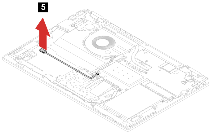
Figure 24. Remove the fingerprint board
