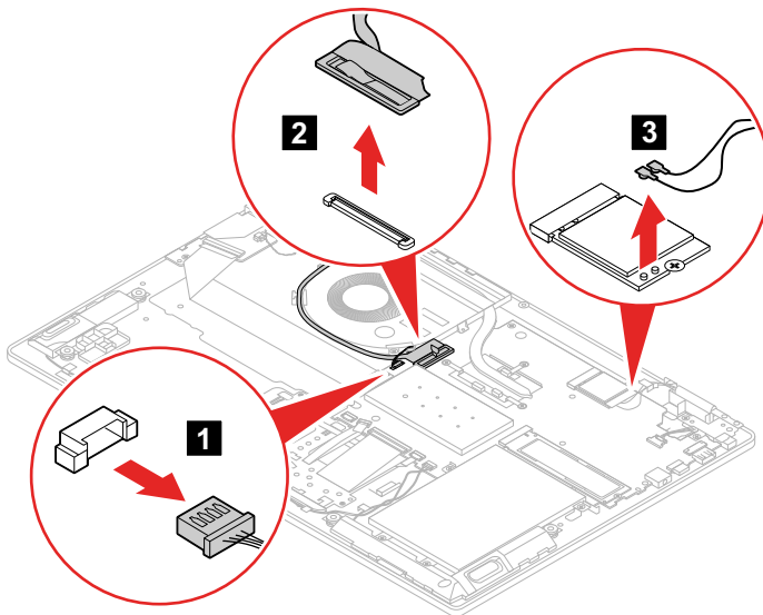
Figure 45. Detach the connectors
