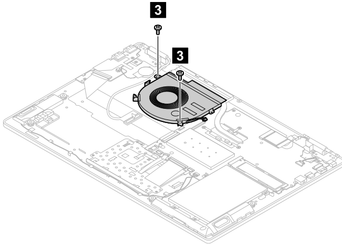
Figure 33. Remove the 2 screws
