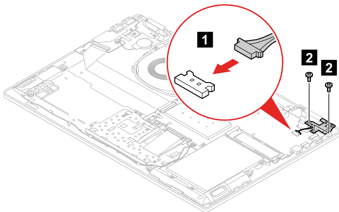
Figure 42. Detach the connector and remove the 2 screws
