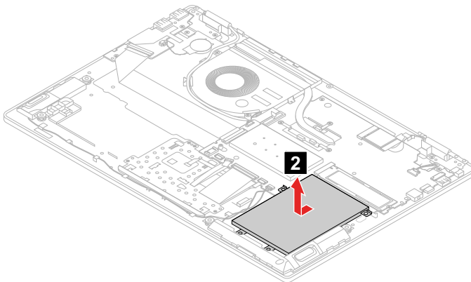
Figure 16. Remove the storage drive
