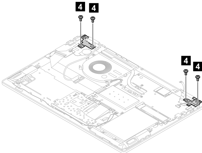
Figure 46. Remove the 4 screws
