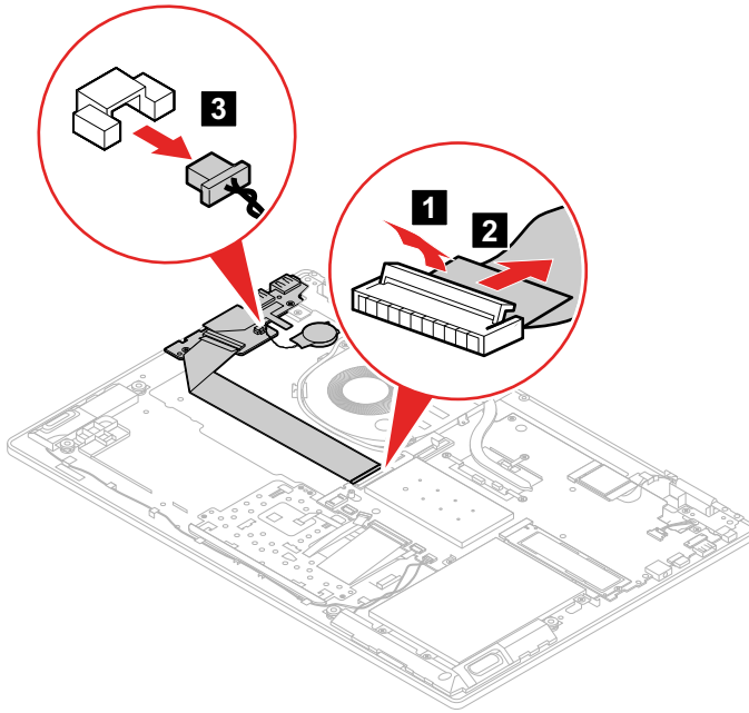
Figure 29. Detach the connectors
