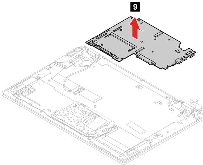
Figure 41. Remove the system board
