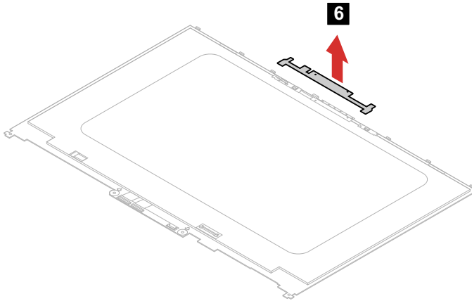
Figure 55. Peel off the conductive tape
