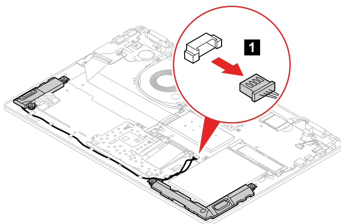
Figure 25. Detach the connector
