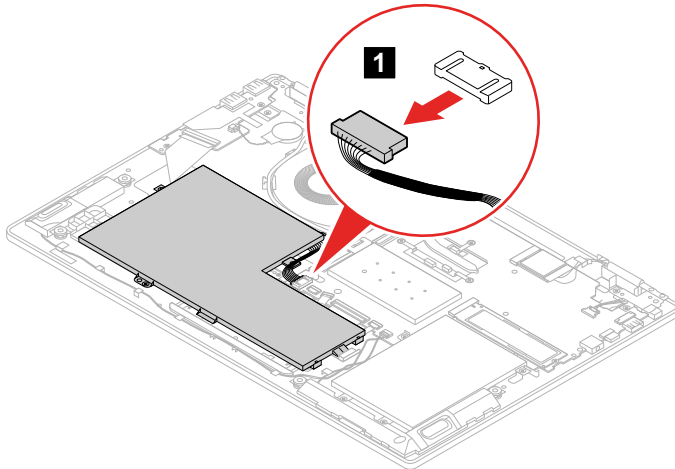
Figure 4. Detach the battery pack connector
