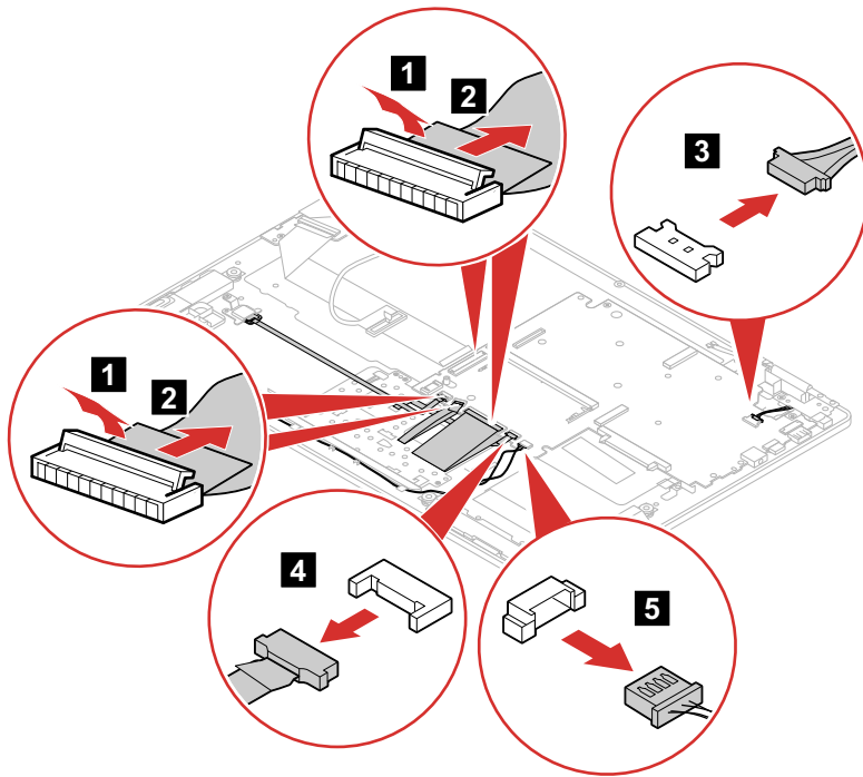
Figure 38. Detach the connectors
