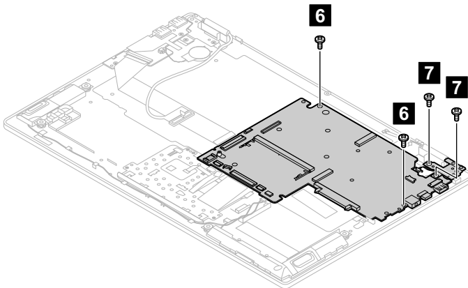
Figure 39. Remove the 4 screws
