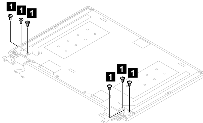
Figure 57. Remove the 6 screws
