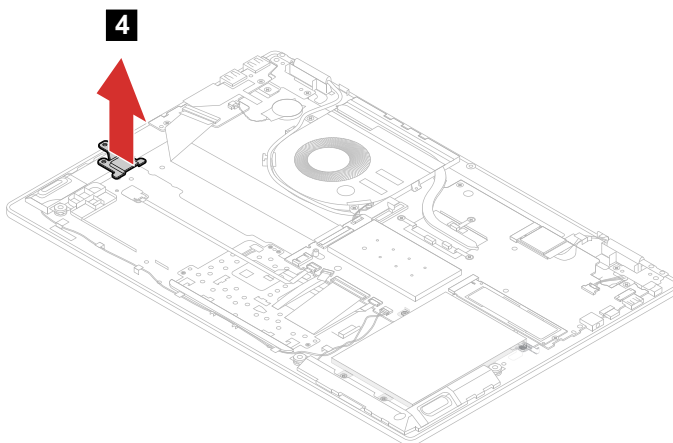
Figure 23. Remove the fingerprint board bracket
