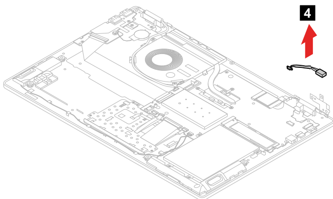
Figure 44. Remove the dc-in cable
