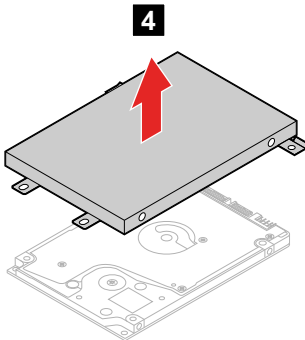
Figure 18. Remove the bracket
