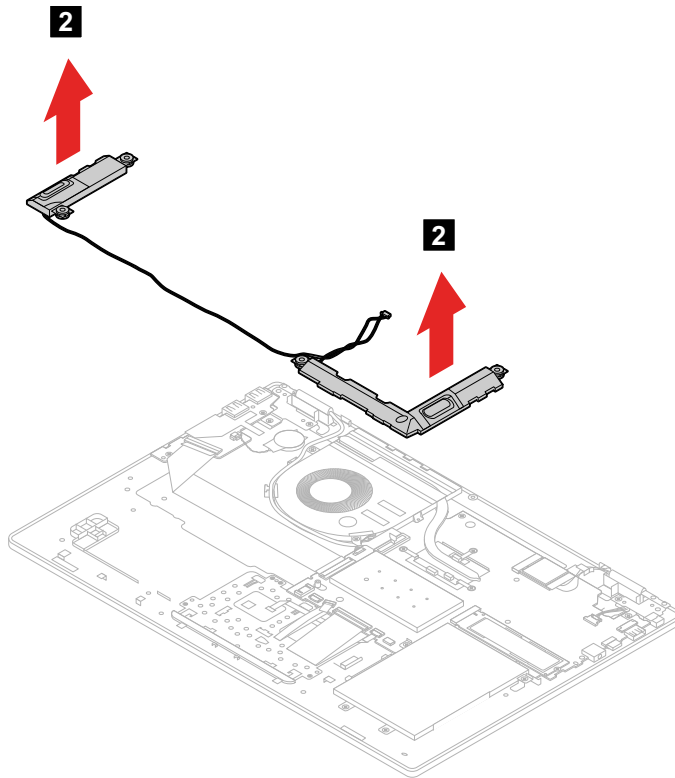
Figure 26. Remove the speakers
