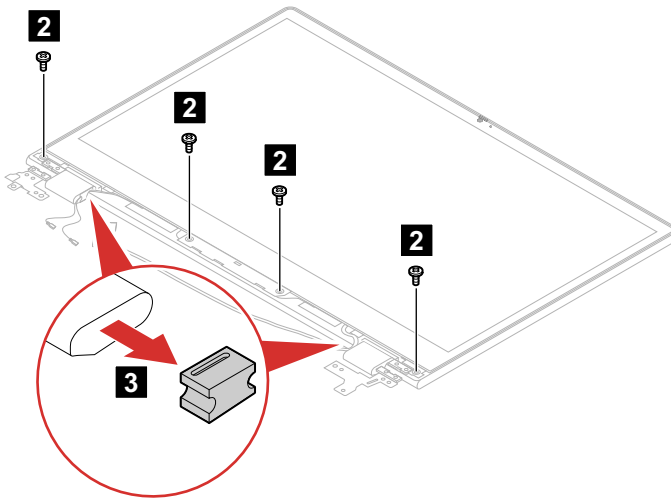
Figure 50. Remove the 4 screws and hinge rubbers
