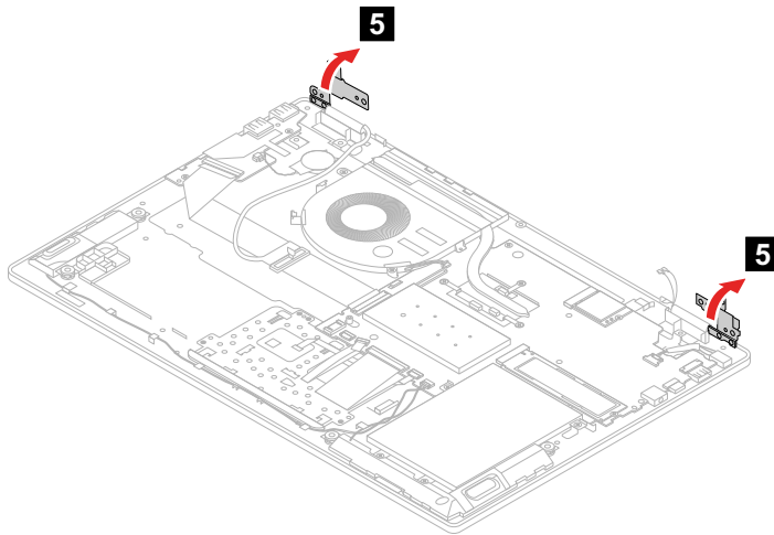
Figure 47. Open the hinges
