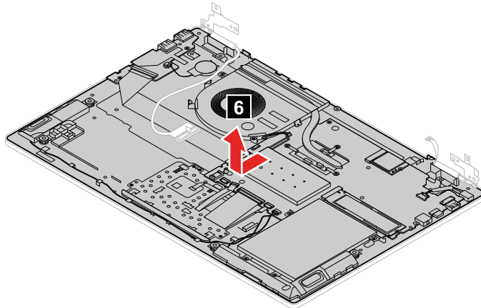
Figure 48. Remove the upper case (with keyboard)
