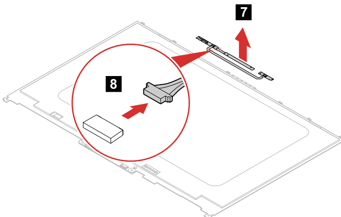
Figure 56. Remove the camera board and microphone board
