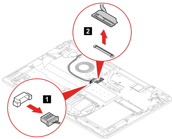
Figure 32. Detach the connectors
