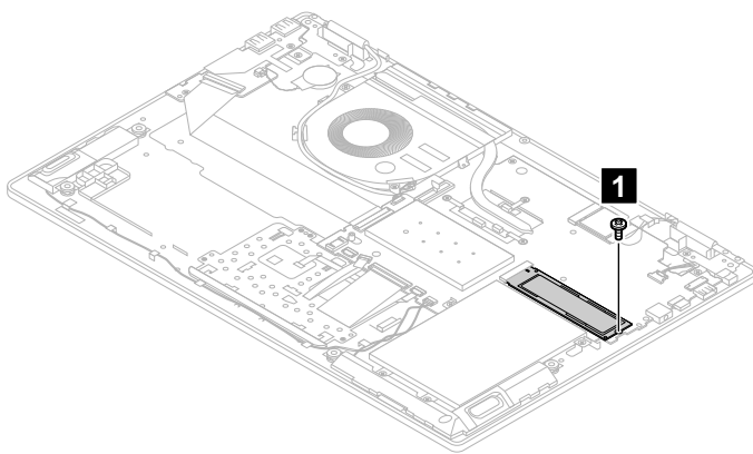
Figure 12. Remove 1 screw (for 2280)
