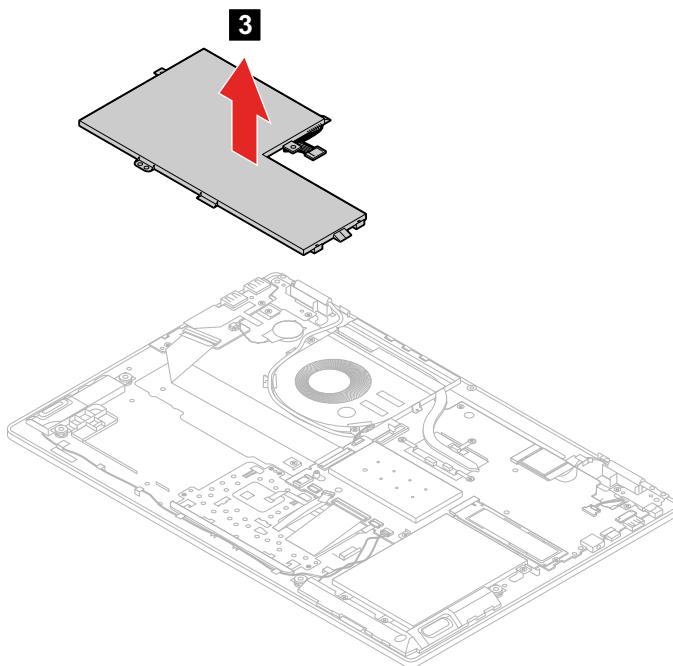
Figure 6. Remove the battery pack
