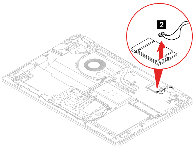
Figure 8. Detach the connectors
