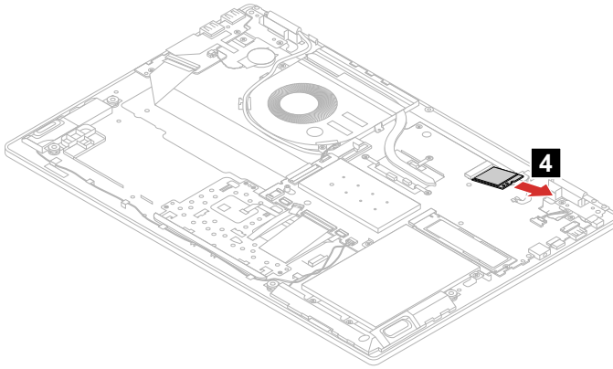
Figure 10. Remove the Wi-Fi card
