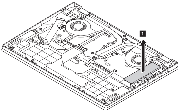
Figure 5. Removal steps of SSD card
