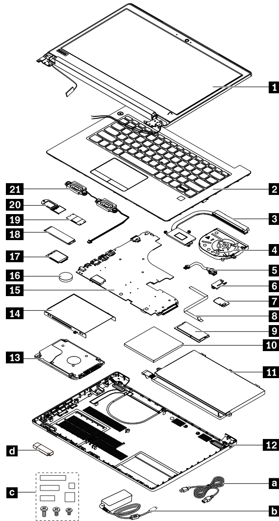
Figure 1. Lenovo E41-55 and Lenovo E41-50 exploded view
