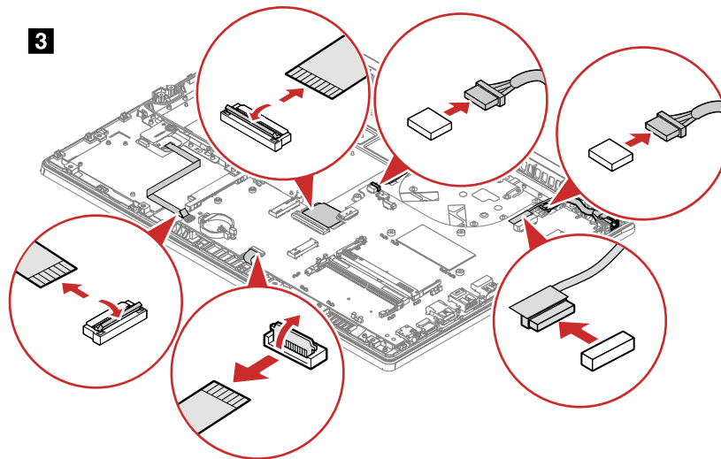
Figure 23. Detach cables and connectors
