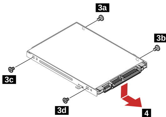
Figure 5. Remove 4 screws and remove hard disk drive bracket
