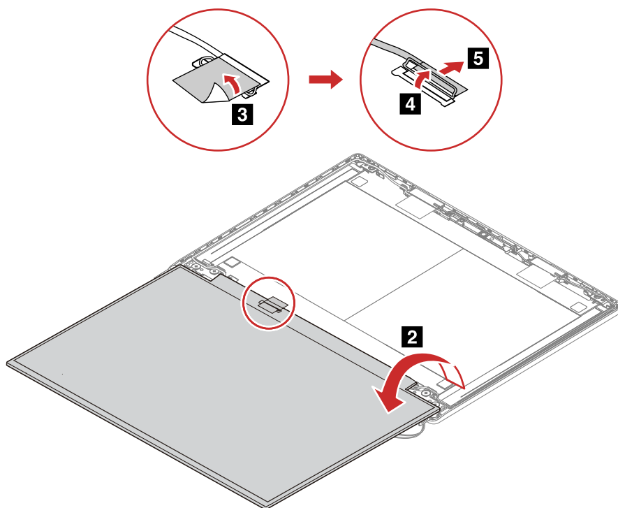
Figure 27. Turn over the LCD panel
