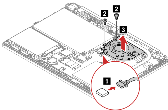
Figure 10. Detach the thermal fan connector
