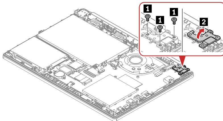
Figure 16. Remove 3 screws and lift up the hinge
