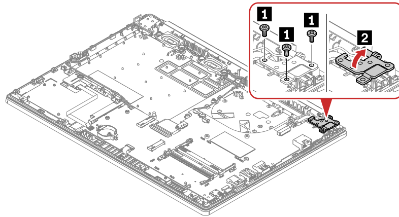
Figure 22. Remove 3 screws and lift up the hinge
