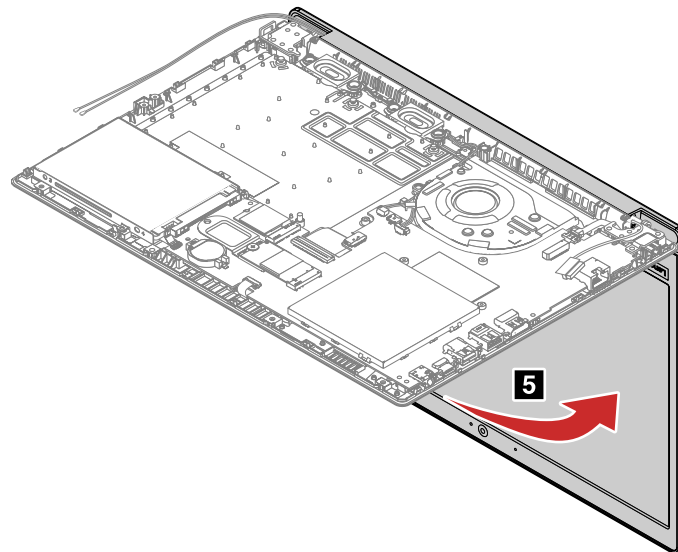
Figure 20. Pivot the LCD unit downward
