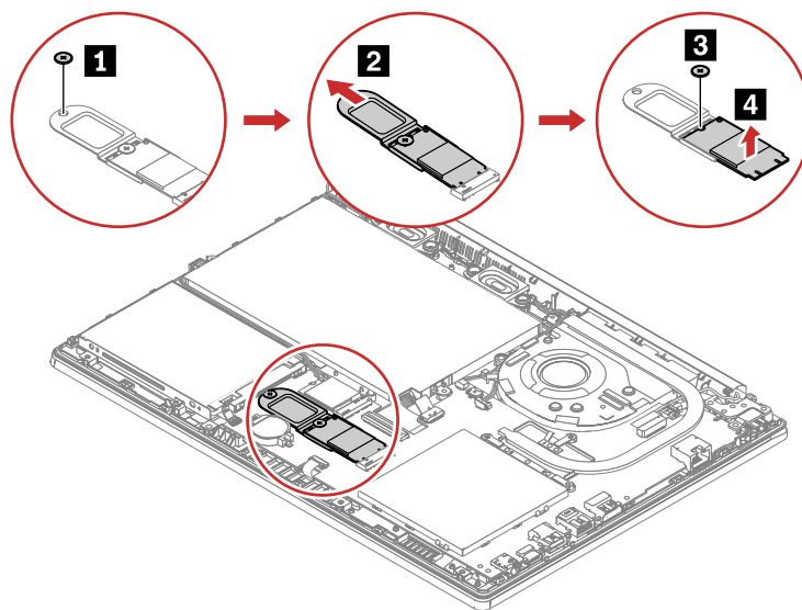
Figure 8. Remove 1 screw and remove the M.2 2242 solid-state drive
