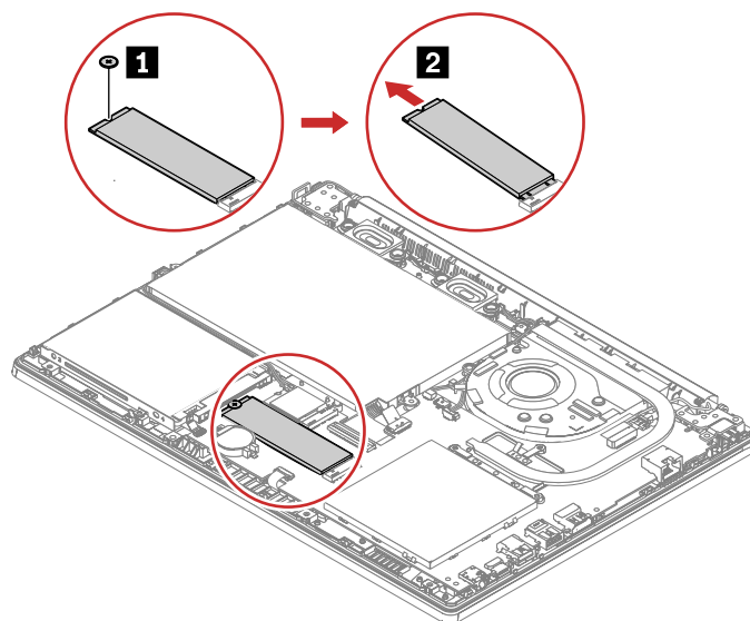
Figure 7. Remove 1 screw and remove the M.2 2280 solid-state drive
