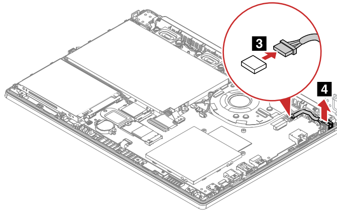
Figure 17. Unplug the DC-in cable and remove the DC-in cable
