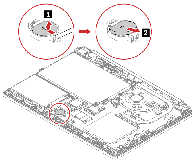
Figure 11. Pry up the CMOS battery
