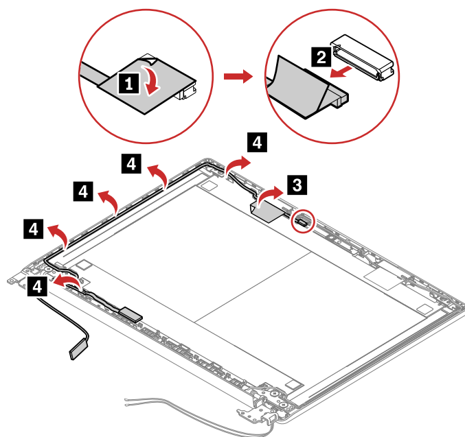
Figure 30. Peel off the sticker, detach the connector and remove the camera cable
