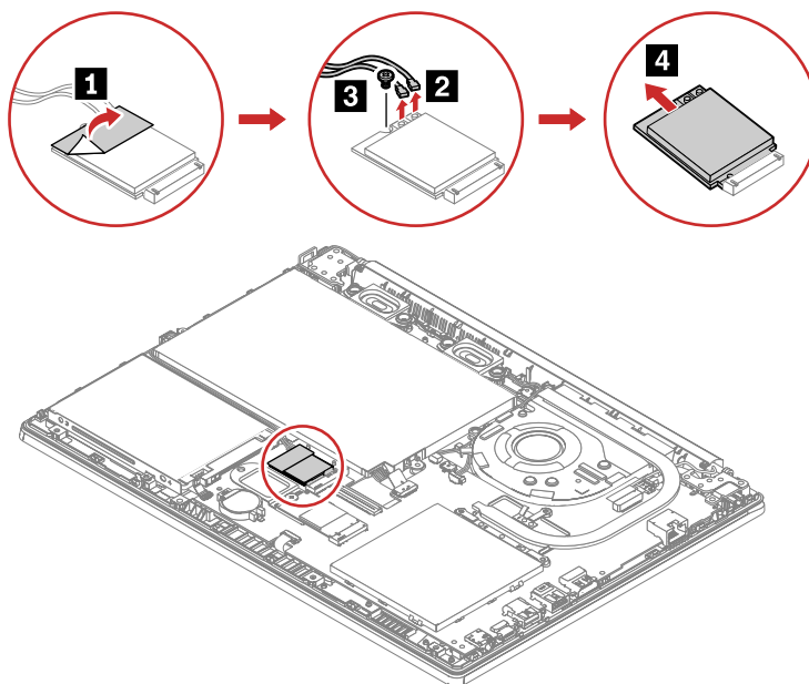
Figure 14. Remove the mylar, detach the cable and remove the Wireless WAN card
