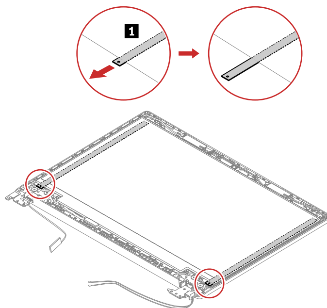
Figure 26. Pull the elastic tapes of LCD bezel
