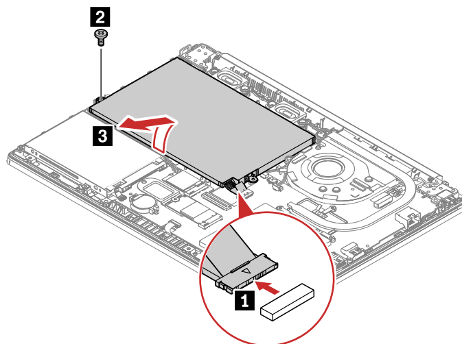
Figure 12. Detach the connector, remove a screw and remove the built-in battery
