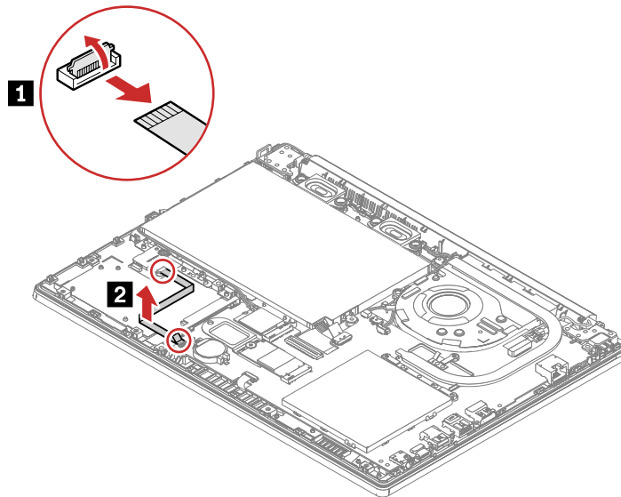
Figure 13. Detach fingerprint reader cable and remove fingerprint reader
