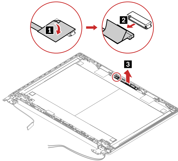
Figure 31. Remove the camera board
