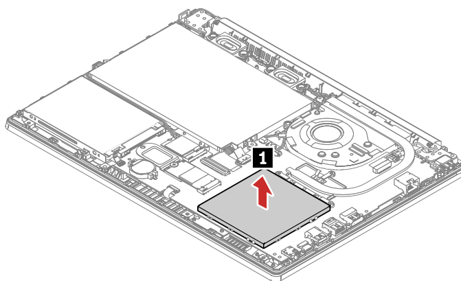
Figure 6. Remove memory module bracket
