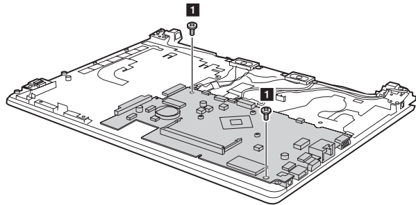
Figure 9. Removal steps of system board (continued)
