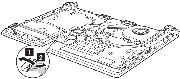
Figure 5. Removal steps of hard disk drive
