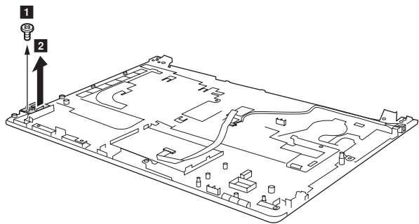
Figure 11. Speakers, base cover, IO board, and DC-IN (continued)
