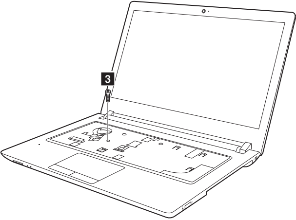
Figure 3. Removal steps of base cover (continued)
