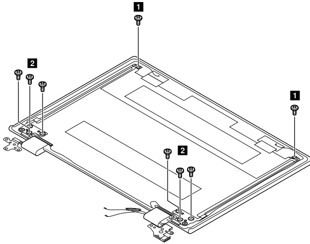
Figure 42. Remove 8 screws
