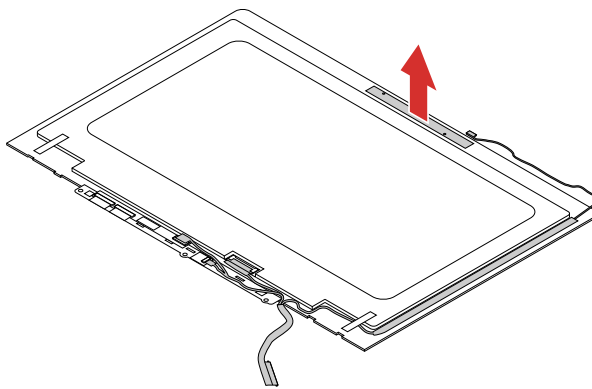
Figure 39. Remove the front camera
