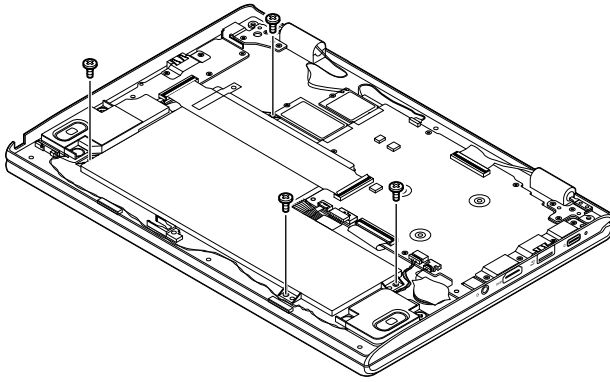
Figure 7. Remove 4 screws
