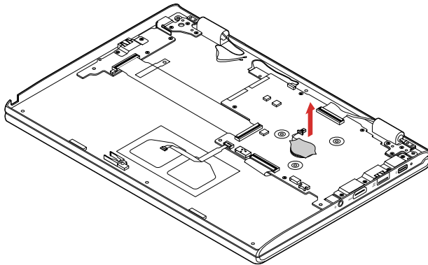
Figure 20. Remove the RTC battery
