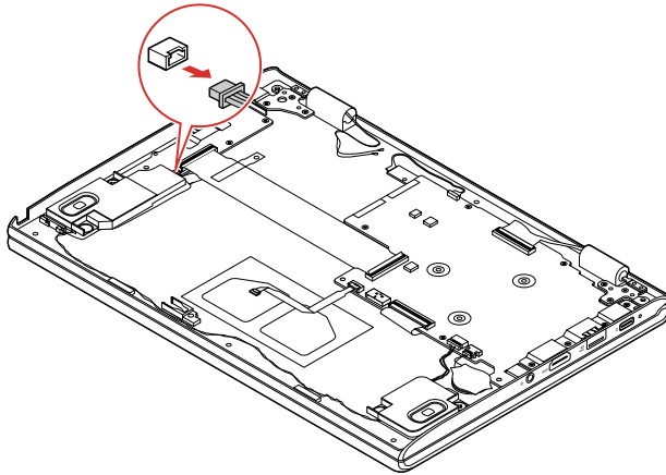
Figure 14. Detach the connector
