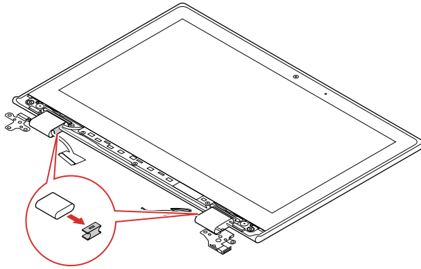
Figure 35. Remove the hinge rubbers
