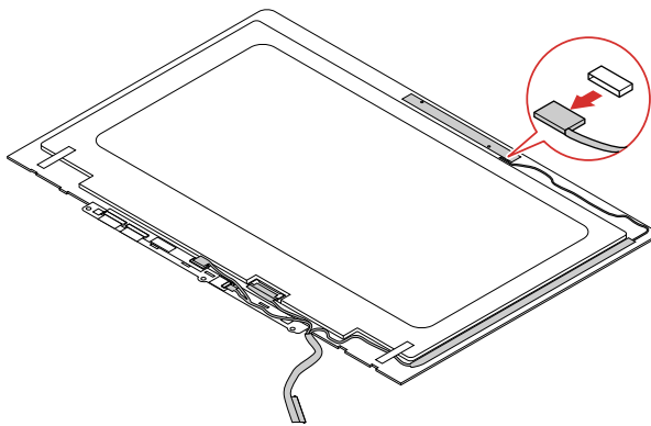
Figure 38. Detach the connector
