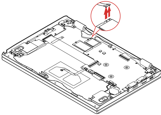
Figure 9. Detach the connectors
