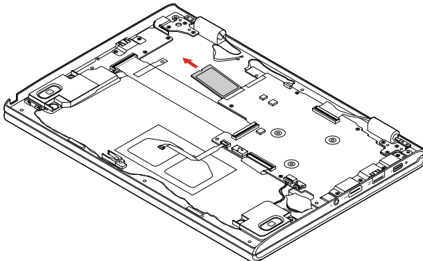
Figure 13. Remove the M.2 solid-state drive
