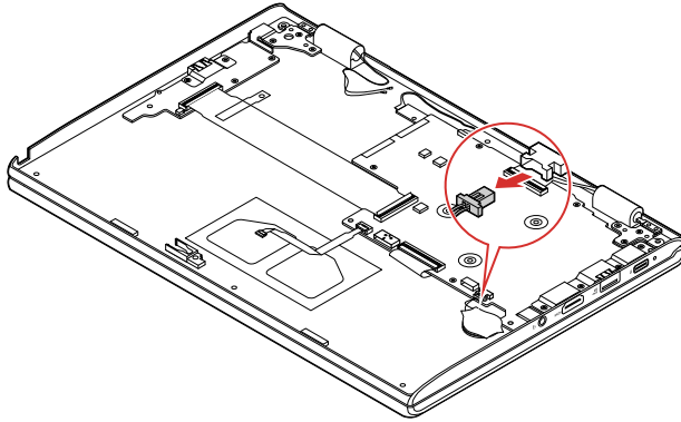
Figure 19. Detach the connector
