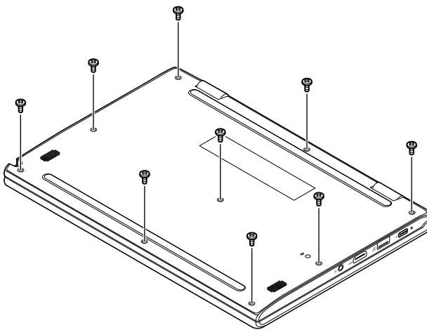
Figure 4. Remove 9 screws
