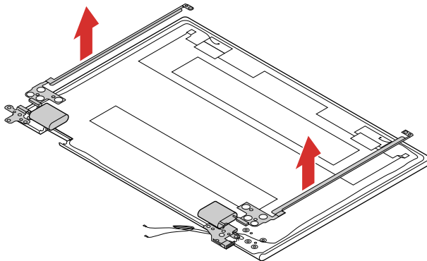
Figure 43. Remove the hinges
