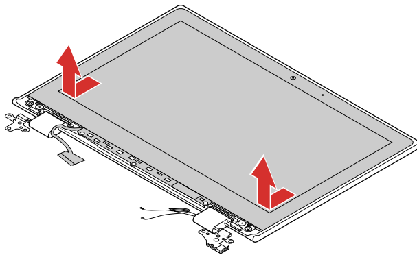
Figure 36. Remove the LCD panel
