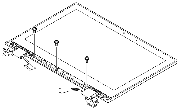
Figure 34. Remove 3 screws
