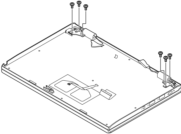
Figure 28. Remove 6 screws
