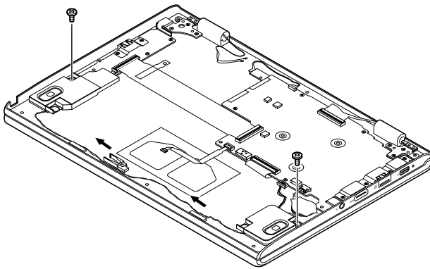
Figure 17. Remove 2 screws
