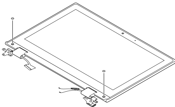
Figure 31. Remove the screw rubbers
