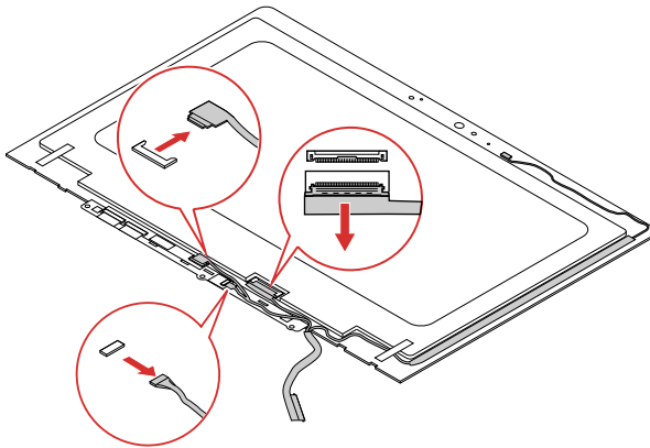
Figure 40. Detach the connectors
