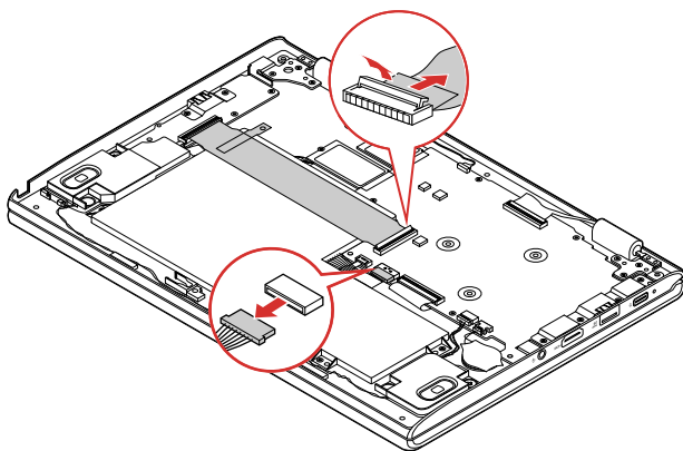
Figure 6. Detach the connectors
