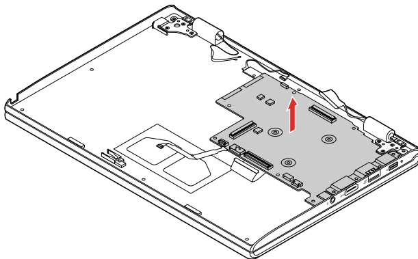
Figure 25. Remove the system board and bracket
