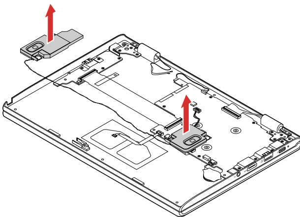
Figure 18. Remove the speakers
