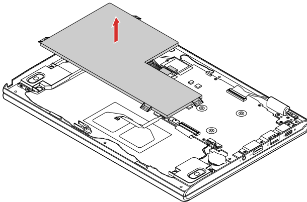
Figure 8. Take out the battery pack
