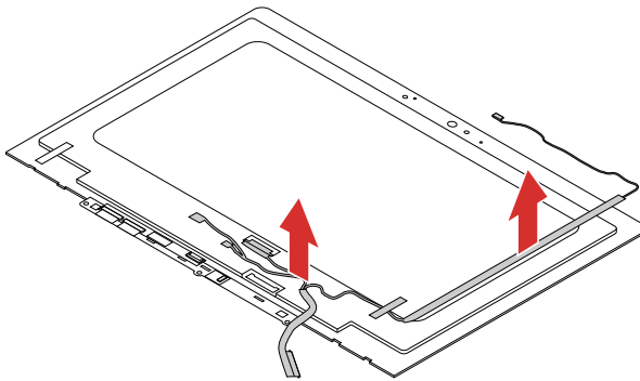
Figure 41. Remove the LCD cable
