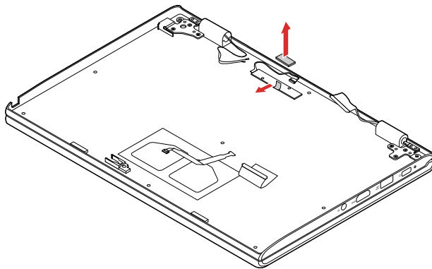
Figure 26. Remove the sponge and peel off the conductive fabric
