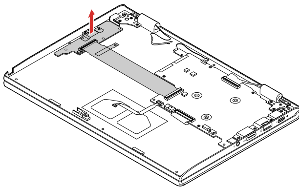
Figure 22. Remove the power board and bracket
