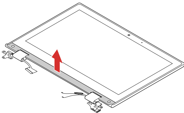
Figure 33. Remove the strip cover
