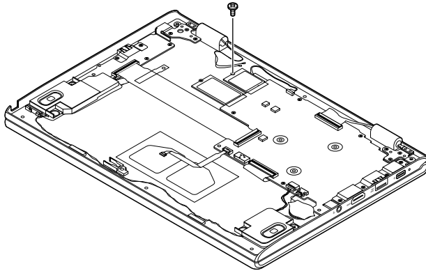
Figure 10. Remove 1 screw
