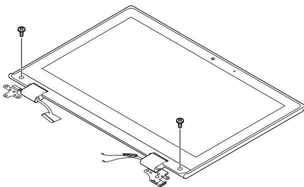
Figure 32. Remove 2 screws
