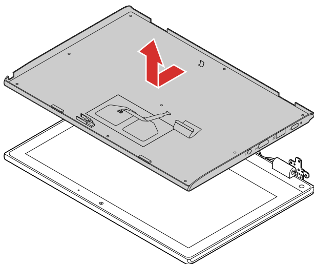
Figure 30. Remove the upper case (with keyboard)
