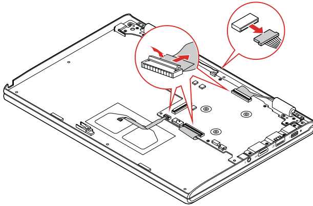
Figure 23. Detach the connectors
