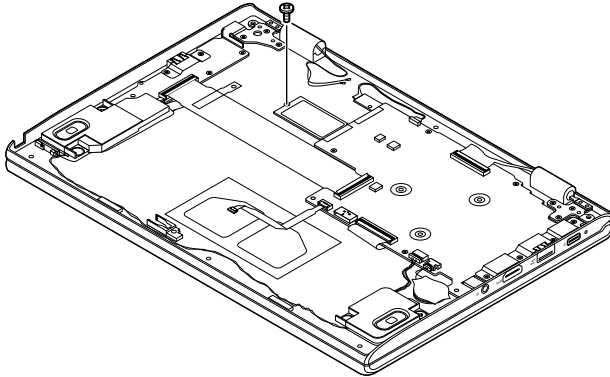
Figure 12. Remove 1 screw
