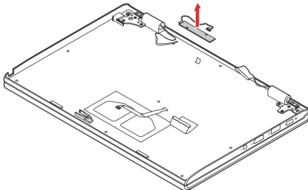
Figure 27. Remove the World-Facing camera
