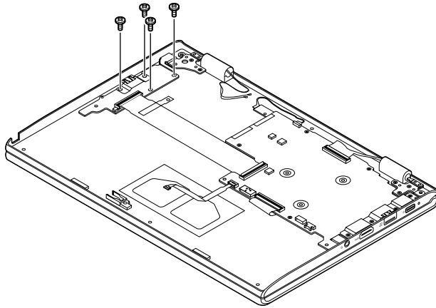
Figure 21. Remove 4 screws
