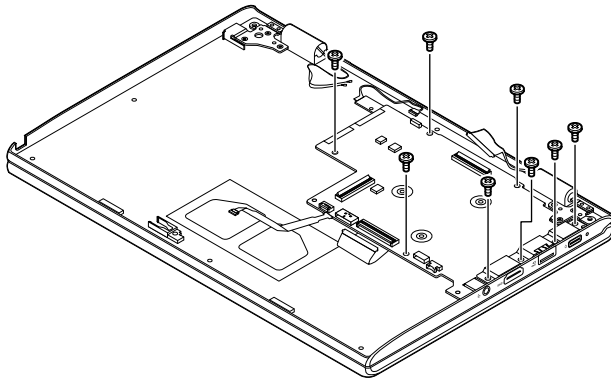
Figure 24. Remove 8 screws
