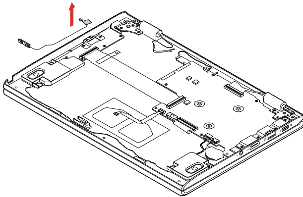
Figure 15. Remove the pen board
