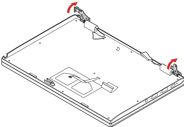
Figure 29. Open the hinges
